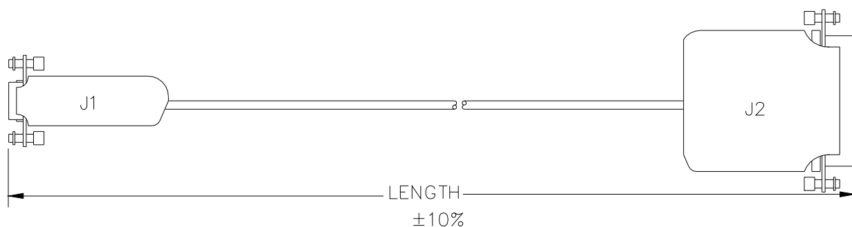
Figure 5: Part Number 89967 9-pin male RS422 Rack cable to 25-pin female RS422 Rack cable
