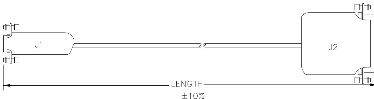
Figure 7: Part Number 89969 15-pin male RS232 cable to 9-pin female RS232 Rack cable
