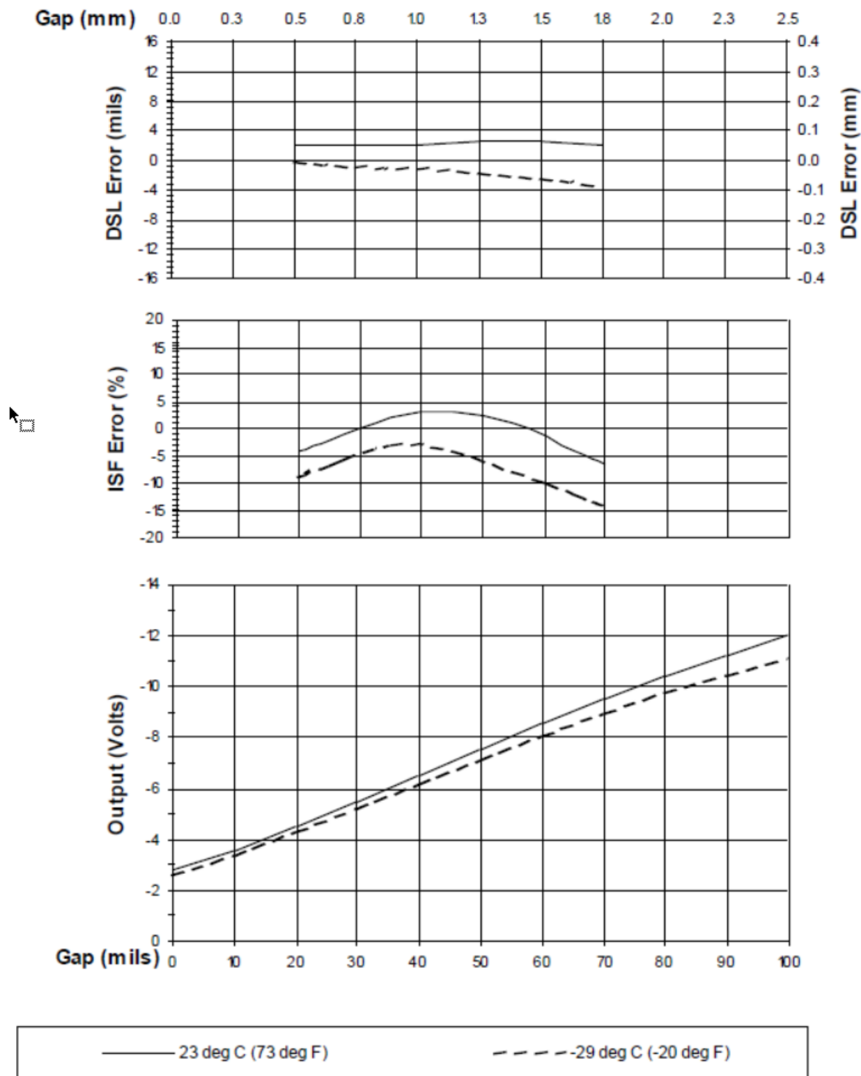
Figure 3: Typical Radiation Resistant 0.300" 15-ft Probe Only @ Tc
