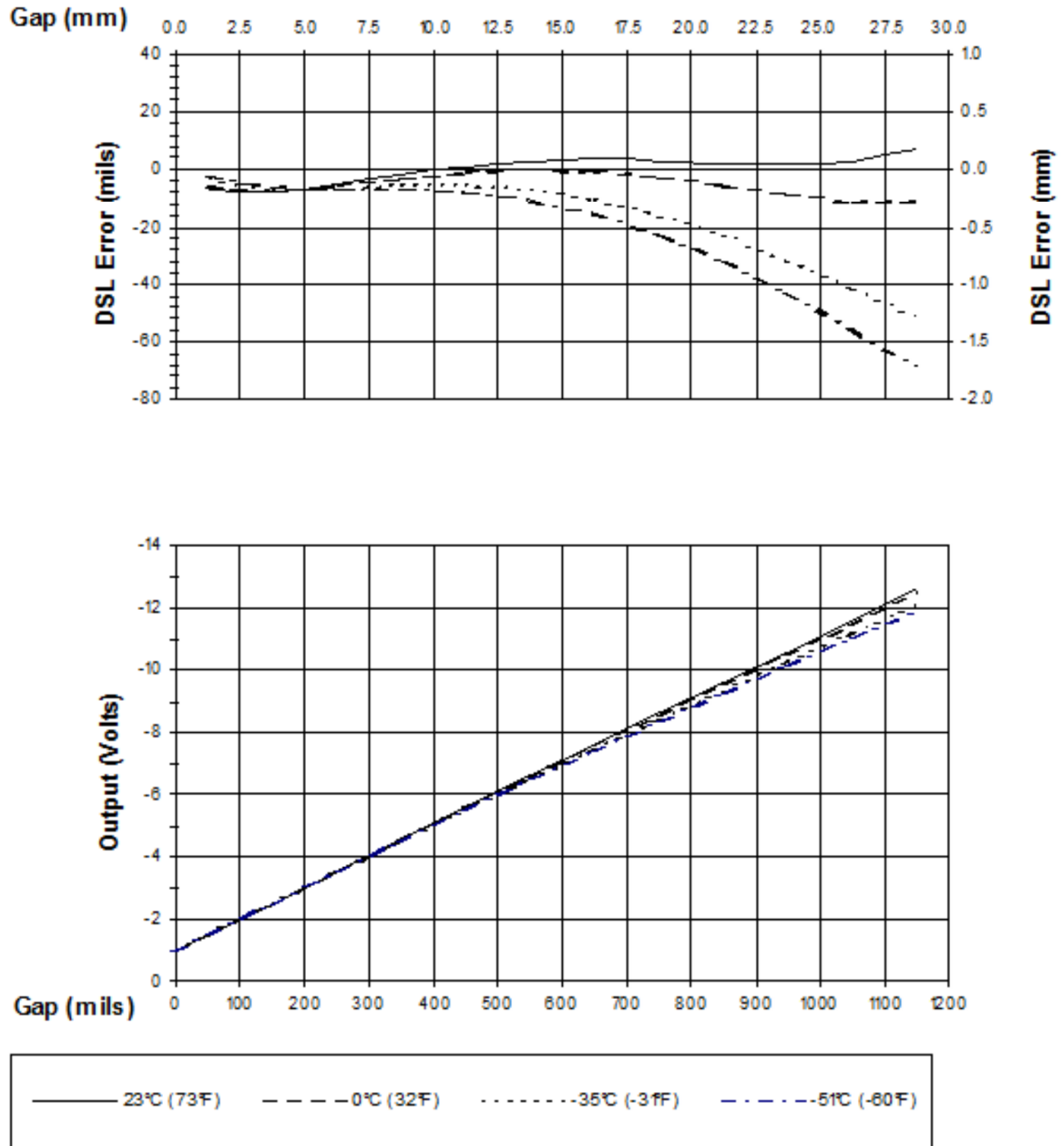
Figure 7: Typical 3300 XL 50 mm 9 m Proximity Sensor with 8 m of Extension Cable @ Low Temperature (Probe is at 25°C)
