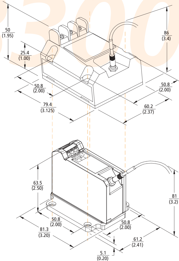
PHYSICAL MOUNTING CHARACTERISTICS SHOWING INTERCHANGEABILITY OF 330100 AND 330900 (TOP) WITH 330180 AND 330980 (BOTTOM) PROXIMITO ® SENSORS WHEN 4-HOLE MOUNTING IS USED | FIG. 1
