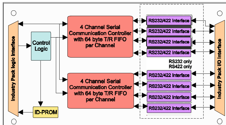
Figure 1-1 : Block Diagram
