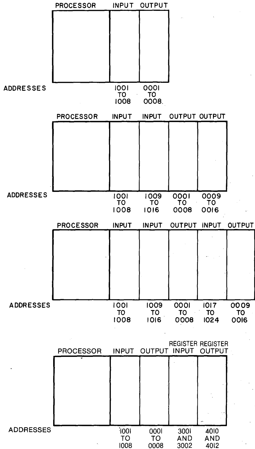
Figure 3-10. I/O Addressing
