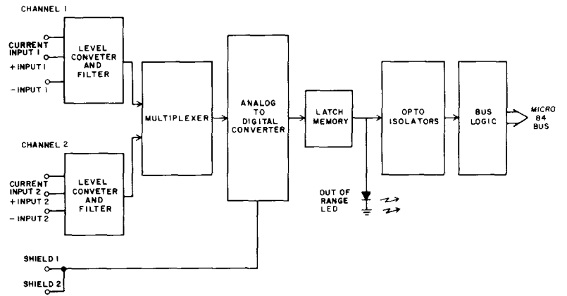
B375, 4-20 mA Analog Input Module Block Diagram
