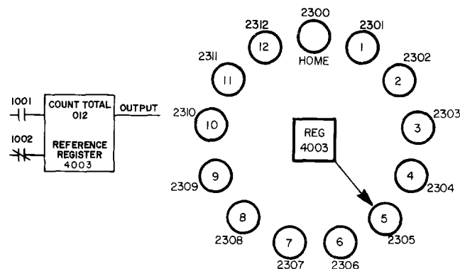
Figure 7-7. Sequencer Example
