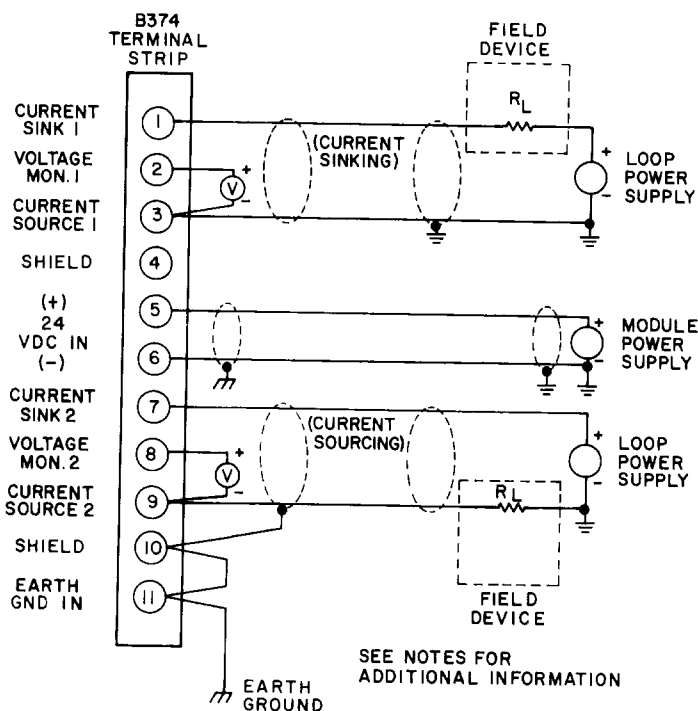
B374, 4-20 mA Analog Output Module Terminal Numbering and Output Connections
