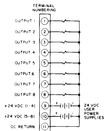
B356-001 OUTPUT MODULE TERMINAL NUMBERING AND CONNECTIONS
