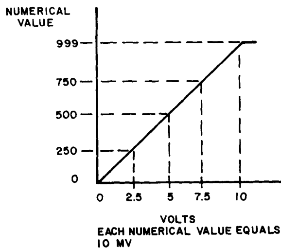
Relationship Between Numerical Value and Voltage Inputs
