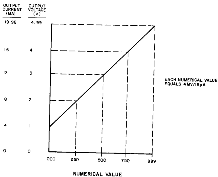
Relationship Between Current/Voltage Output and Numerical Input
