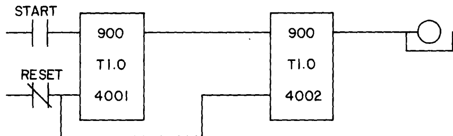
Figure 7-5. Interconnecting Timers
