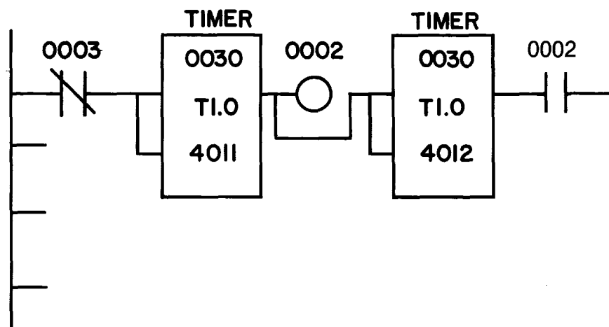
Figure 7-3. Coil Used as Discrete Input
