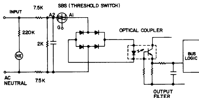
B351 115 VAC Input Module Simplified Schematic
