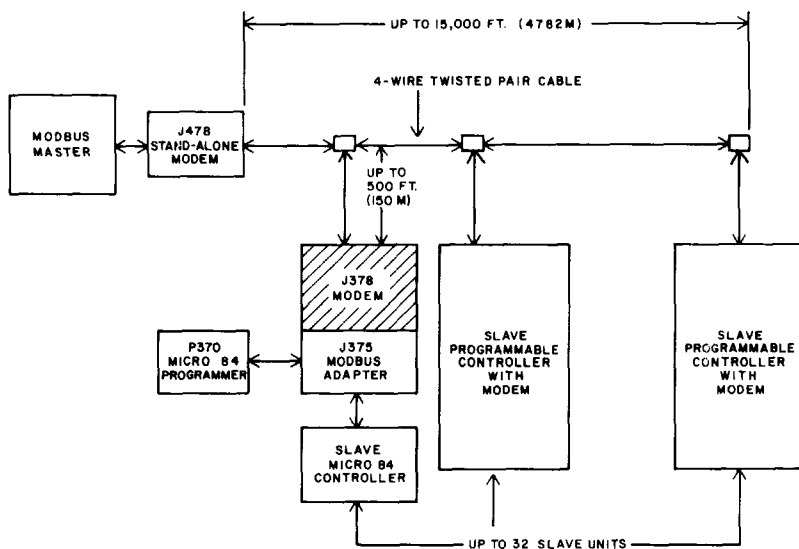
Typical Modbus Network Showing Placement of J378 Modem Within Network
