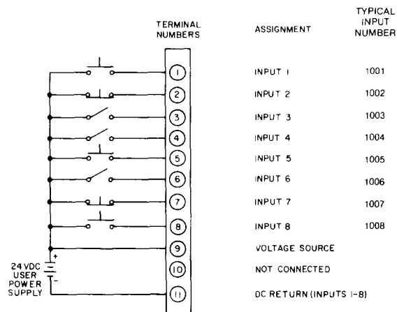
B357-001 INPUT MODULE TERMINAL NUMBERING AND CONNECTIONS
