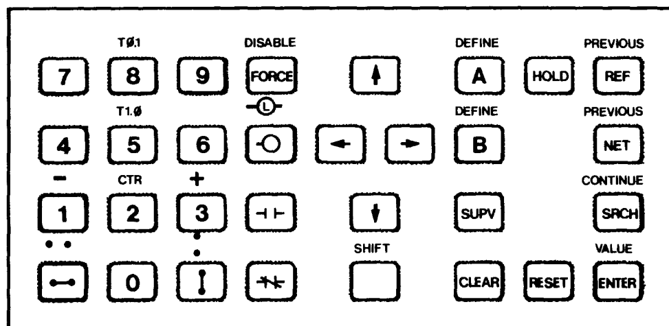
Figure 6-6. Function Keyboard
