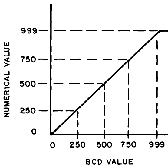
Numerical Output of B371 is Directly Proportional to Input BCD Value
