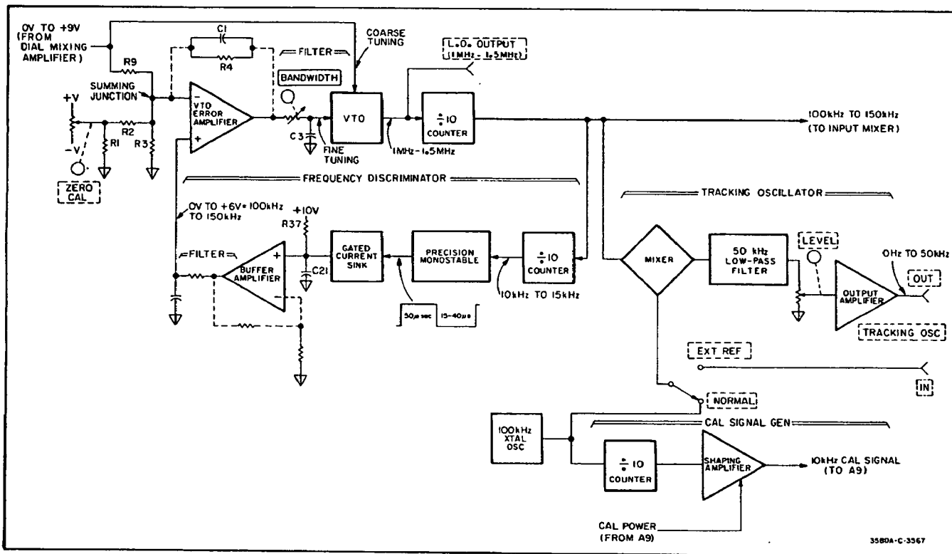
Figure 4-15. VTO and Tracking Oscillator (AS).
