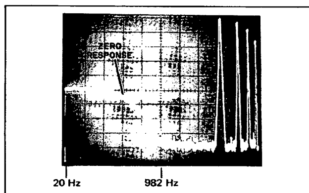
Figure 3-25. Log Sweep (300 Hz BW).
