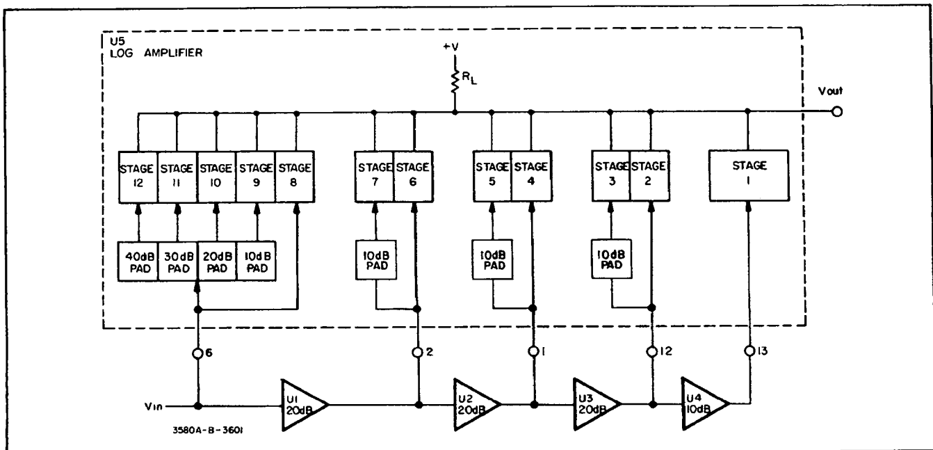
Figure 4-6. Log Amplifier.
