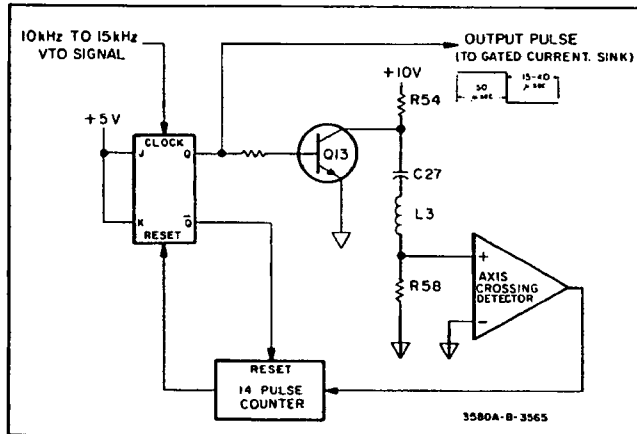
Figure 4-16. Precision Monostable.
