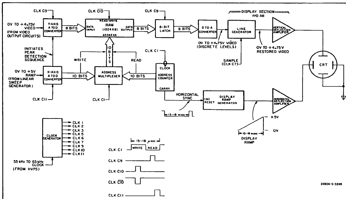
Figure 4-21. Digital Storage and Display Sections.
