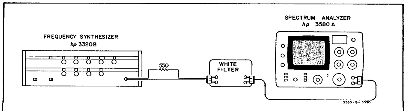
Figure 5-3. Spurious Response Test.
