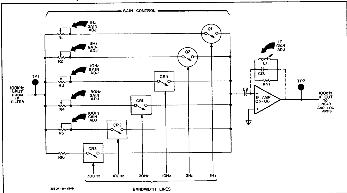
Figure 4-4. IF Amplifier.
