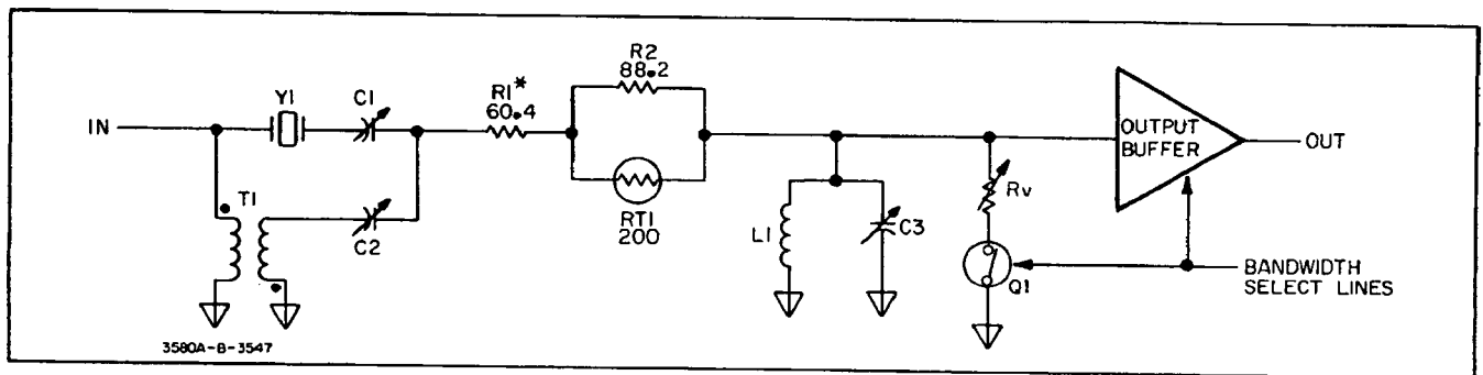
Figure 4-2. Typical Crystal Filter Stage.
