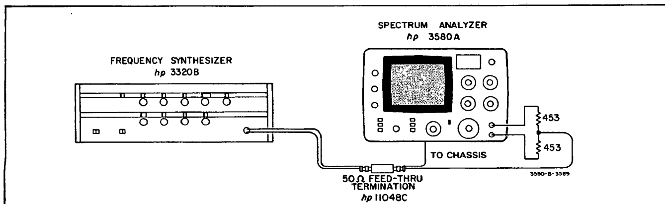
Figure 5-4. Common Mode Rejection Test.
