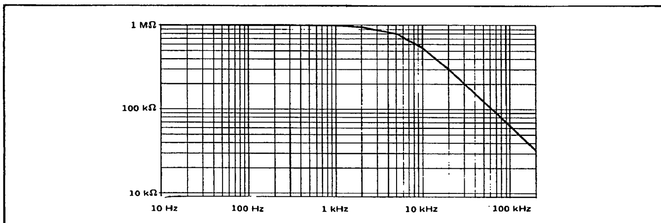
Figure 3-4. Graph Z_t vs. Frequency.
