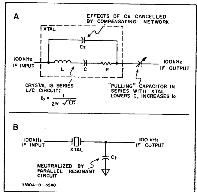
Figure 4-3. Crystal Filter.
