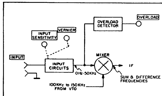
Figure 3-7. Input Section.
