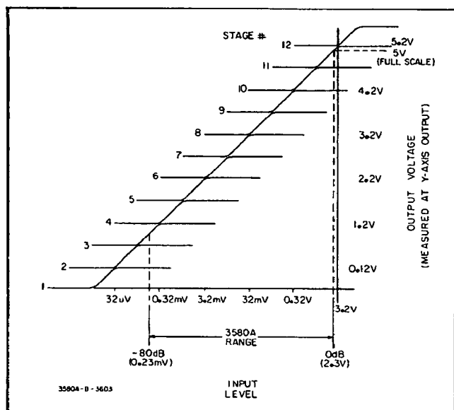
Figure 4-8. Log Amplifier Input and Output Levels.
