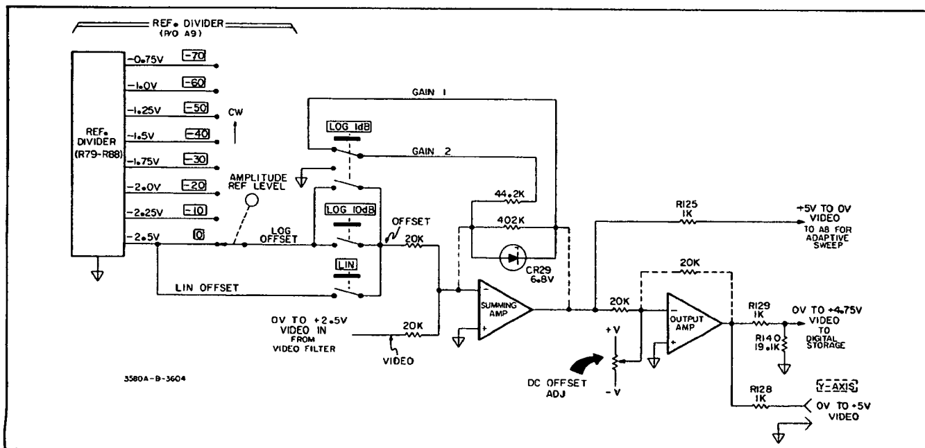
Figure 4-9. Video Output.
