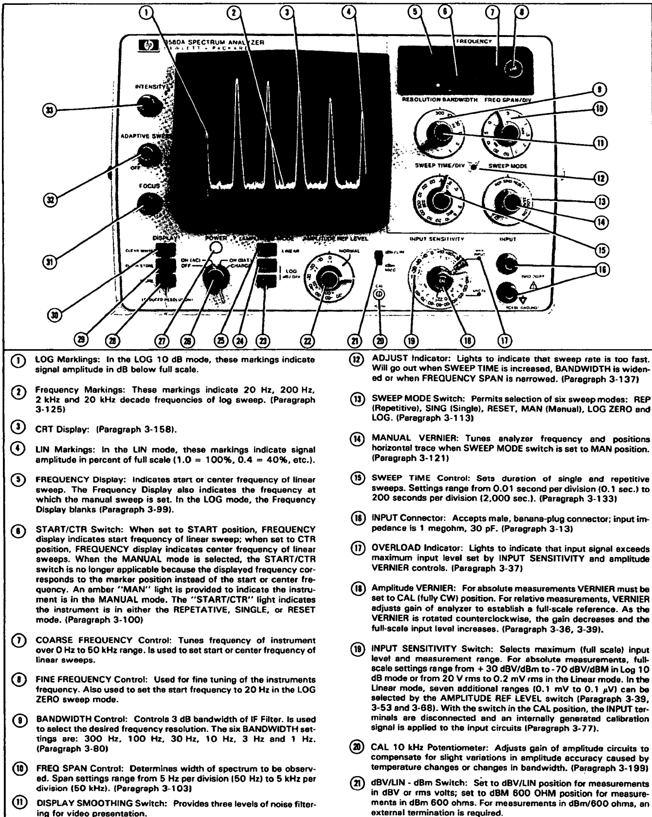
Figure 3-1. Front Panel.
