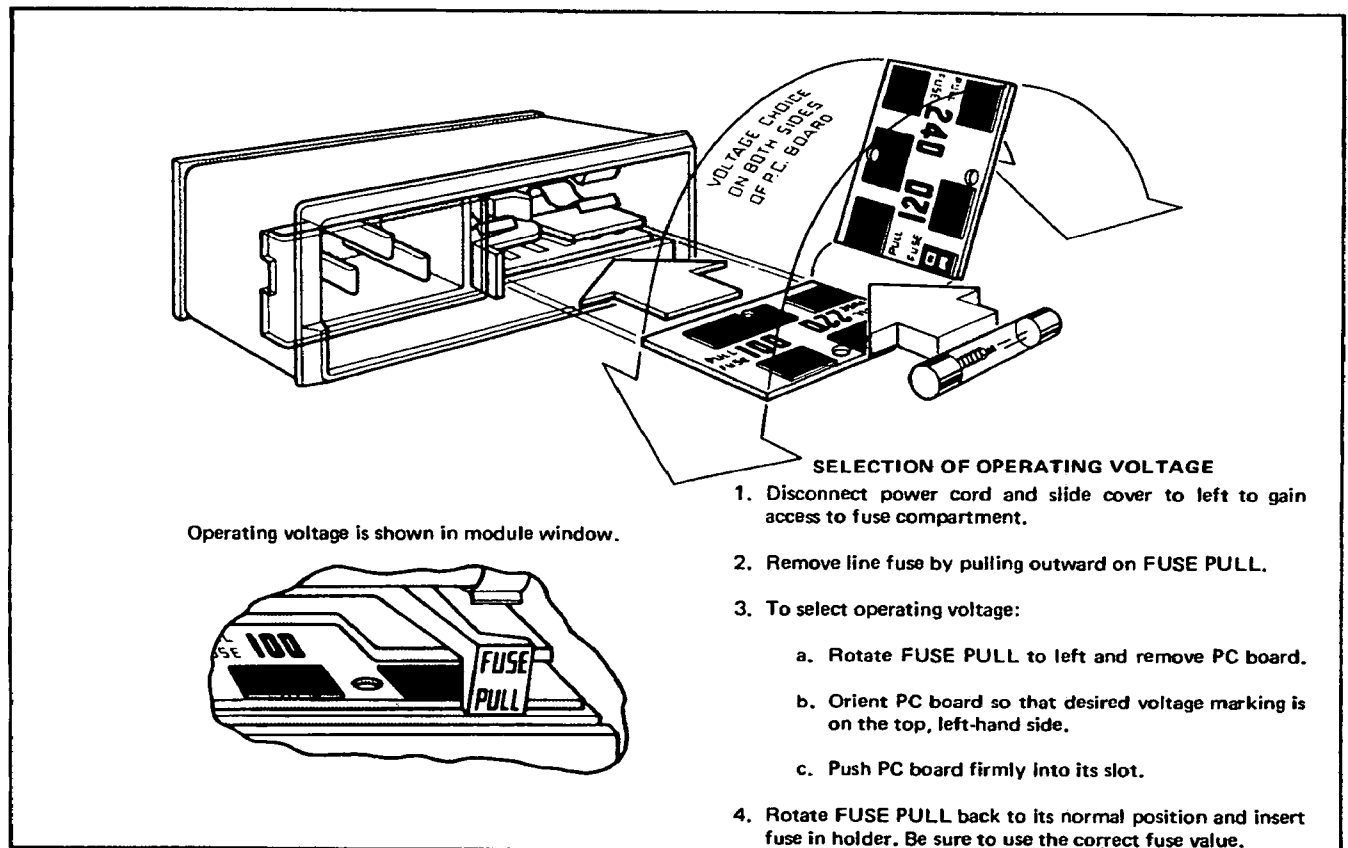
Figure 3-33. Voltage Selection.
