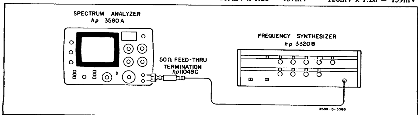
Figure 5-6. Proper Hookup.
