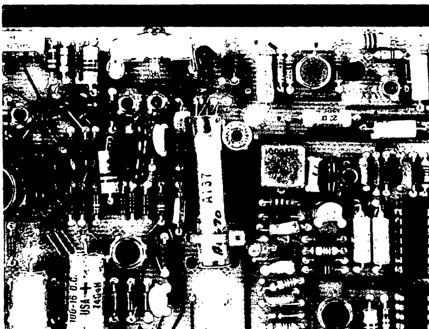
Figure 8-5. New Crystal on Modified A2 Board.
