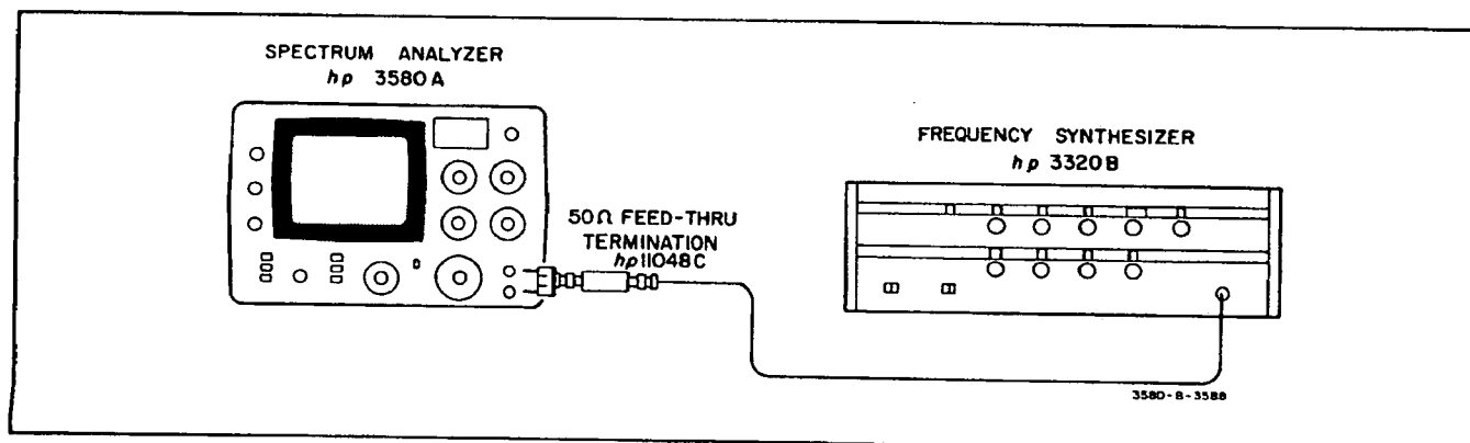
Figure 5-2. Proper Hookup.
