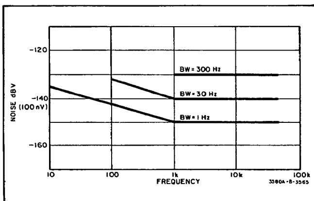
Figure 3-9. Noise vs. Frequency.
