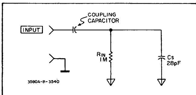
Figure 3-3. Equivalent Input Circuit.
