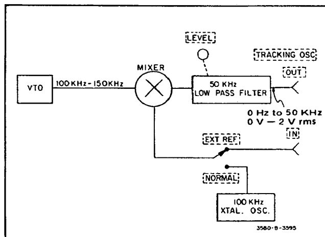
Figure 3-31. Tracking Oscillator.
