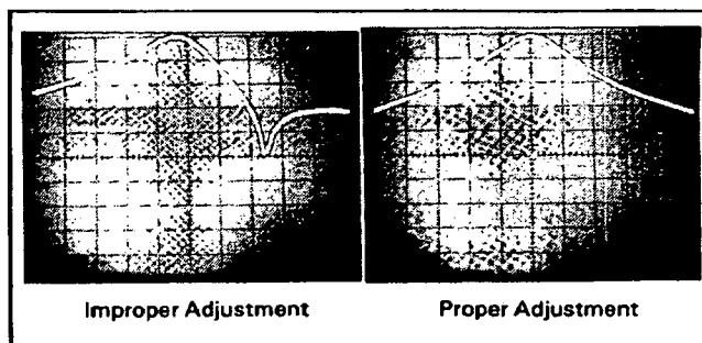
Figure 5-5. Symmetry Adjustment.
