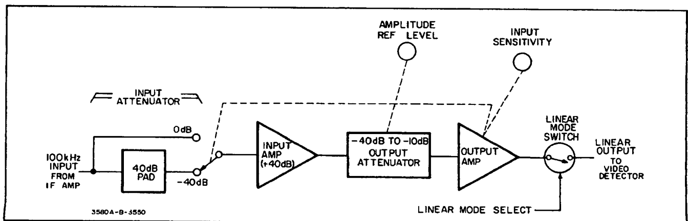
Figure 4-5. Linear Amplifier.
