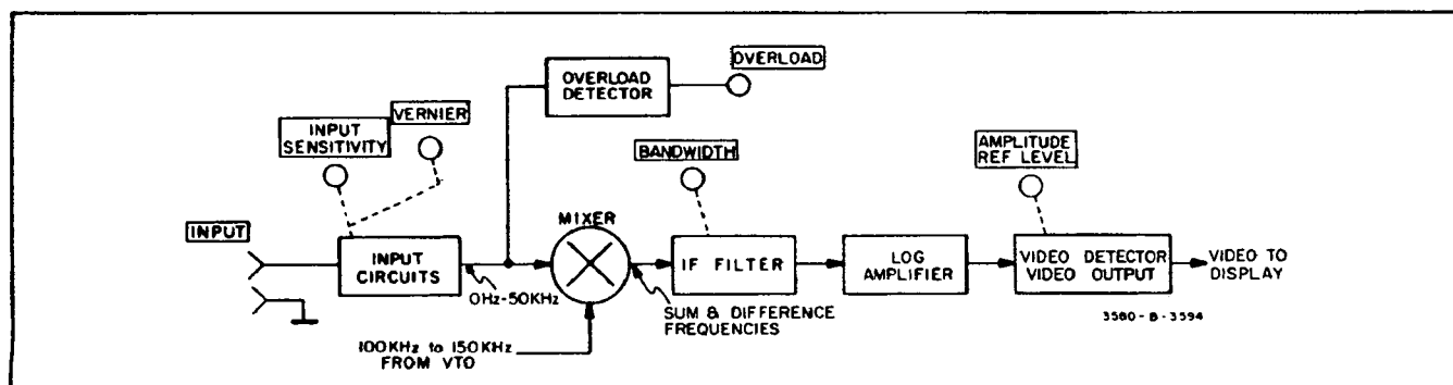
Figure 3-11. Amplitude Section (Log Mode).
