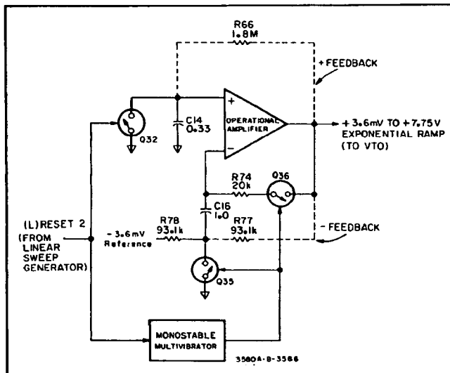
Figure 4-18. Overall Log Sweep Generator.
