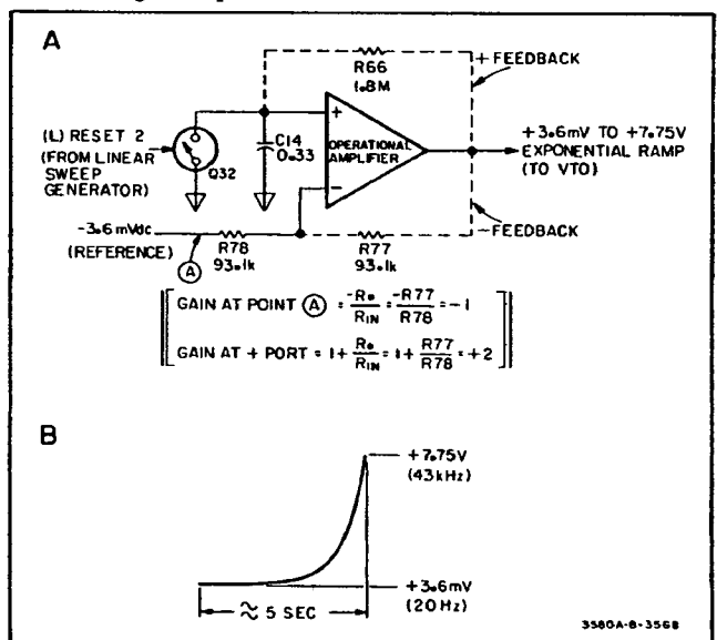
Figure 4-17. Basic Log Sweep Generator.
