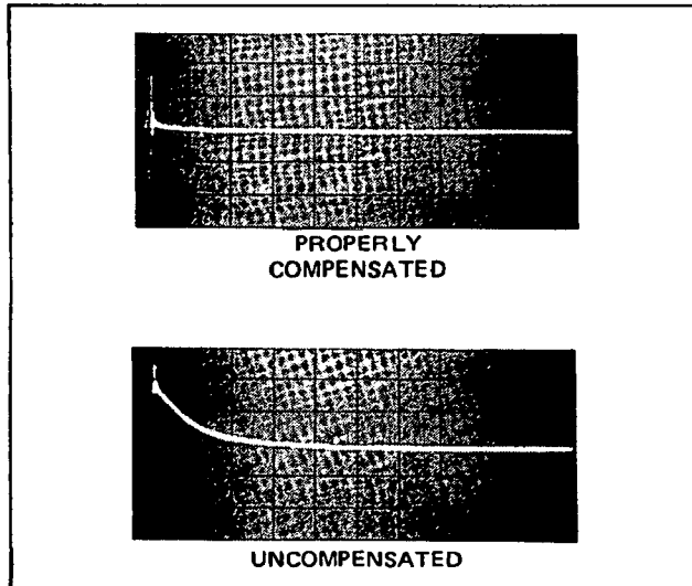
Figure 3-35. Probe Compensation.
