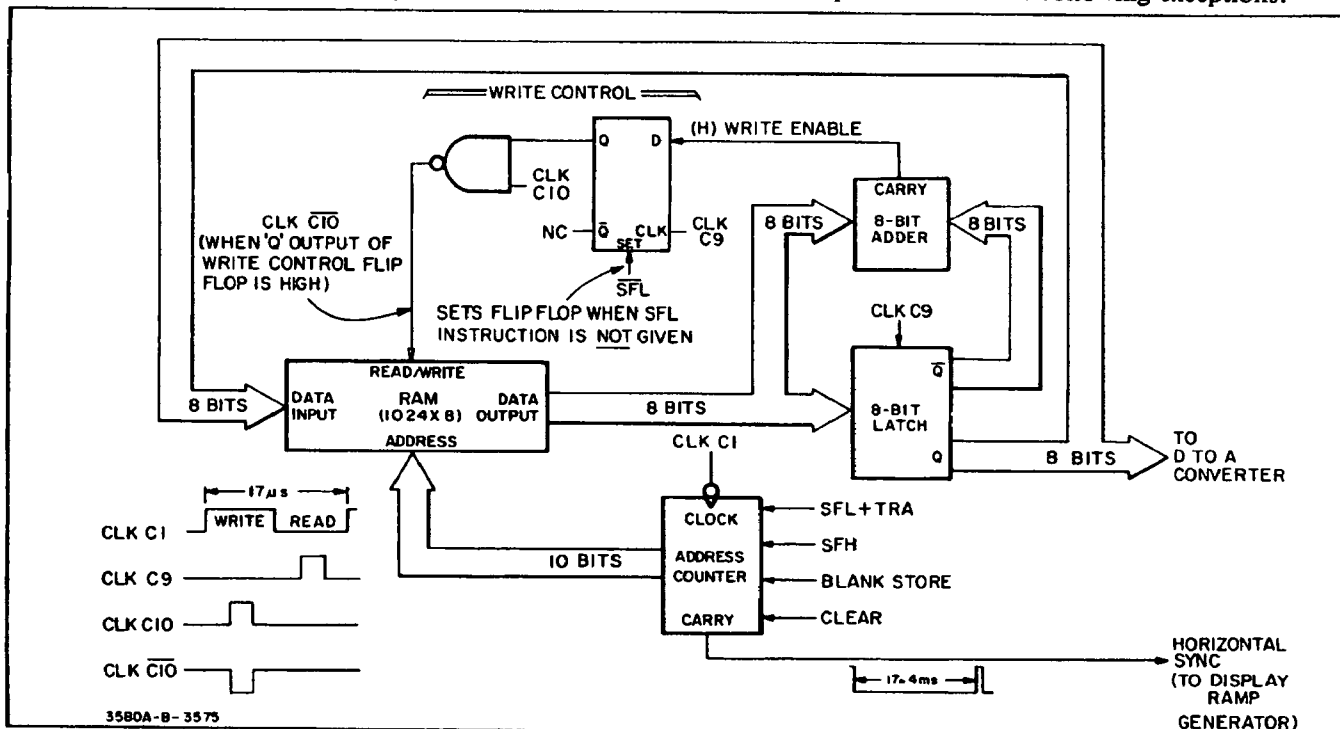
Figure 4-24. Equivalent Circuit (State 1).
