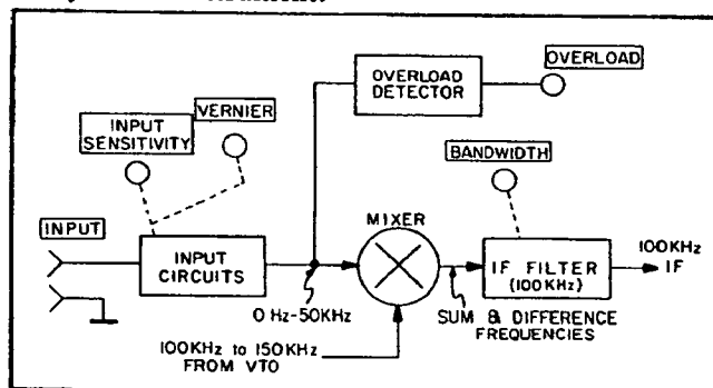
Figure 3-13. Frequency Tuning.
