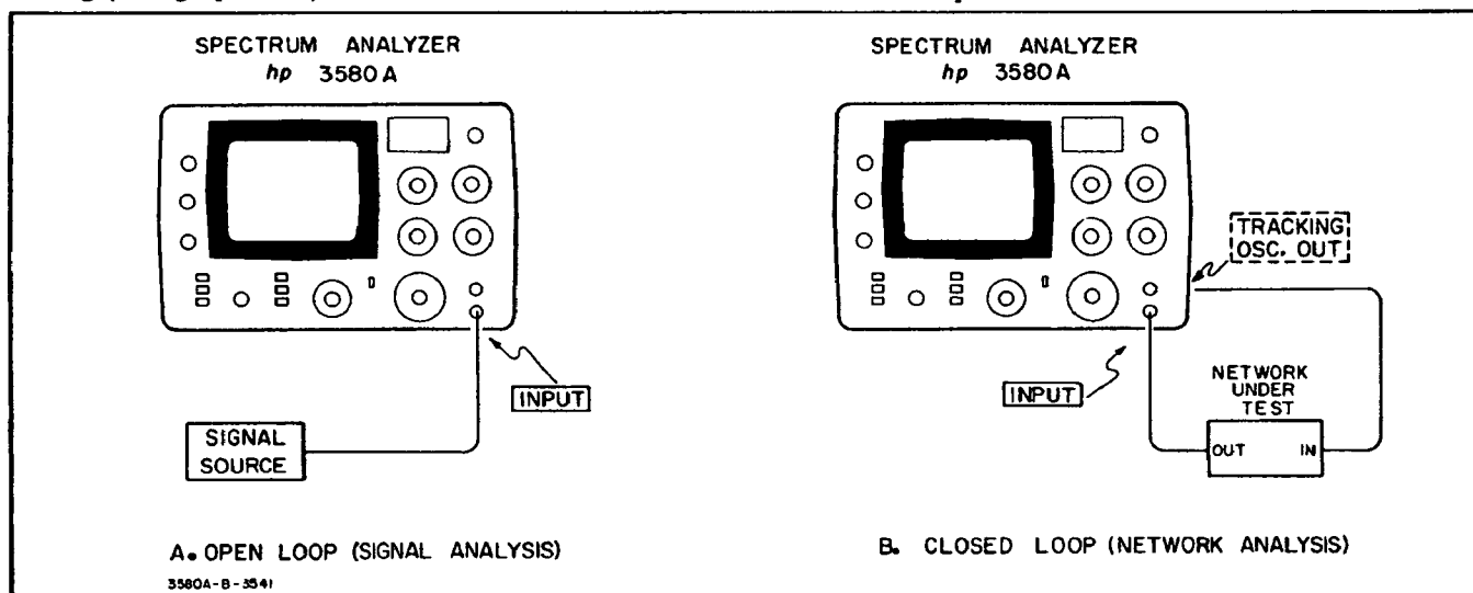
Figure 3-6. Measurement Configurations.
