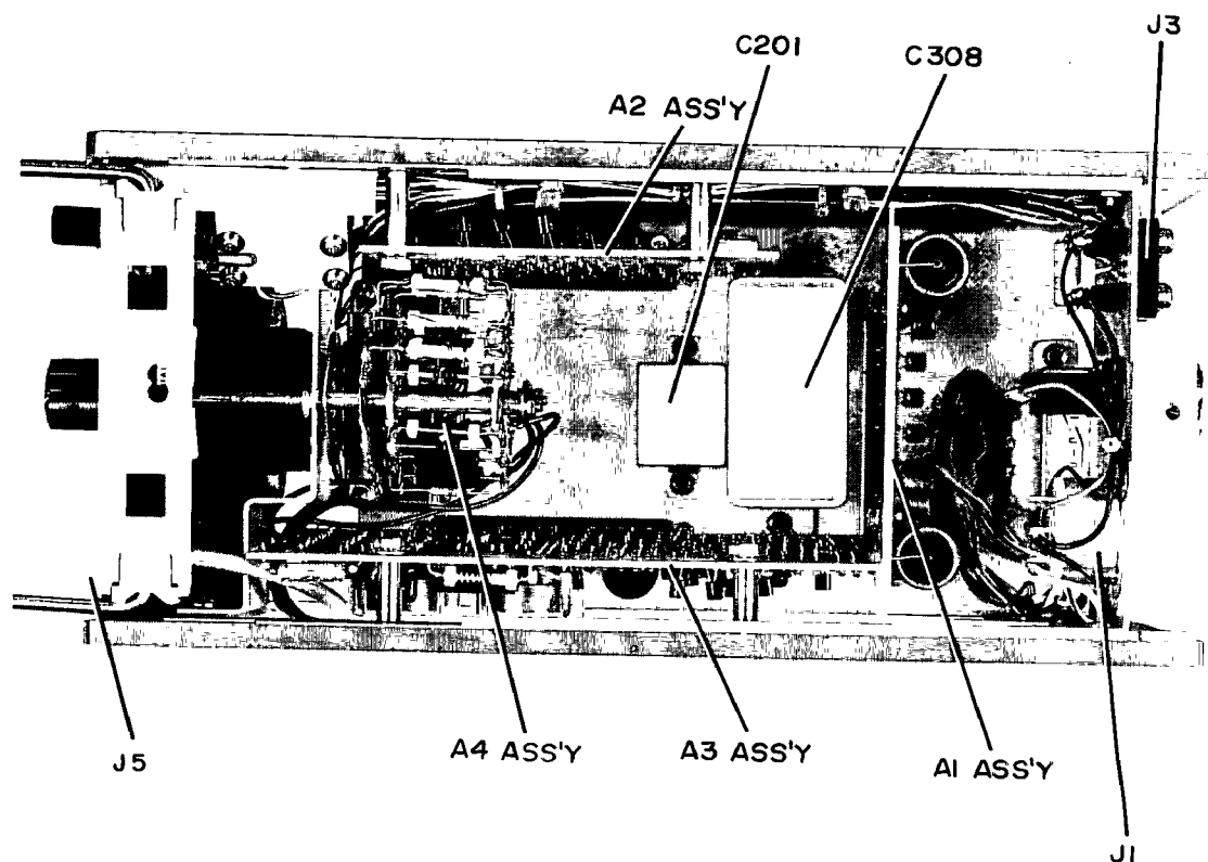
Figure 8-6. Model 4328A Bottom Internal View
