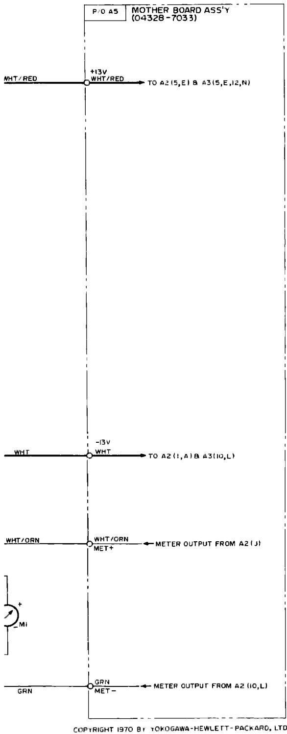
Figure 8-19 Power Supply Ass'y A1 Mother Board Ass'y A5
