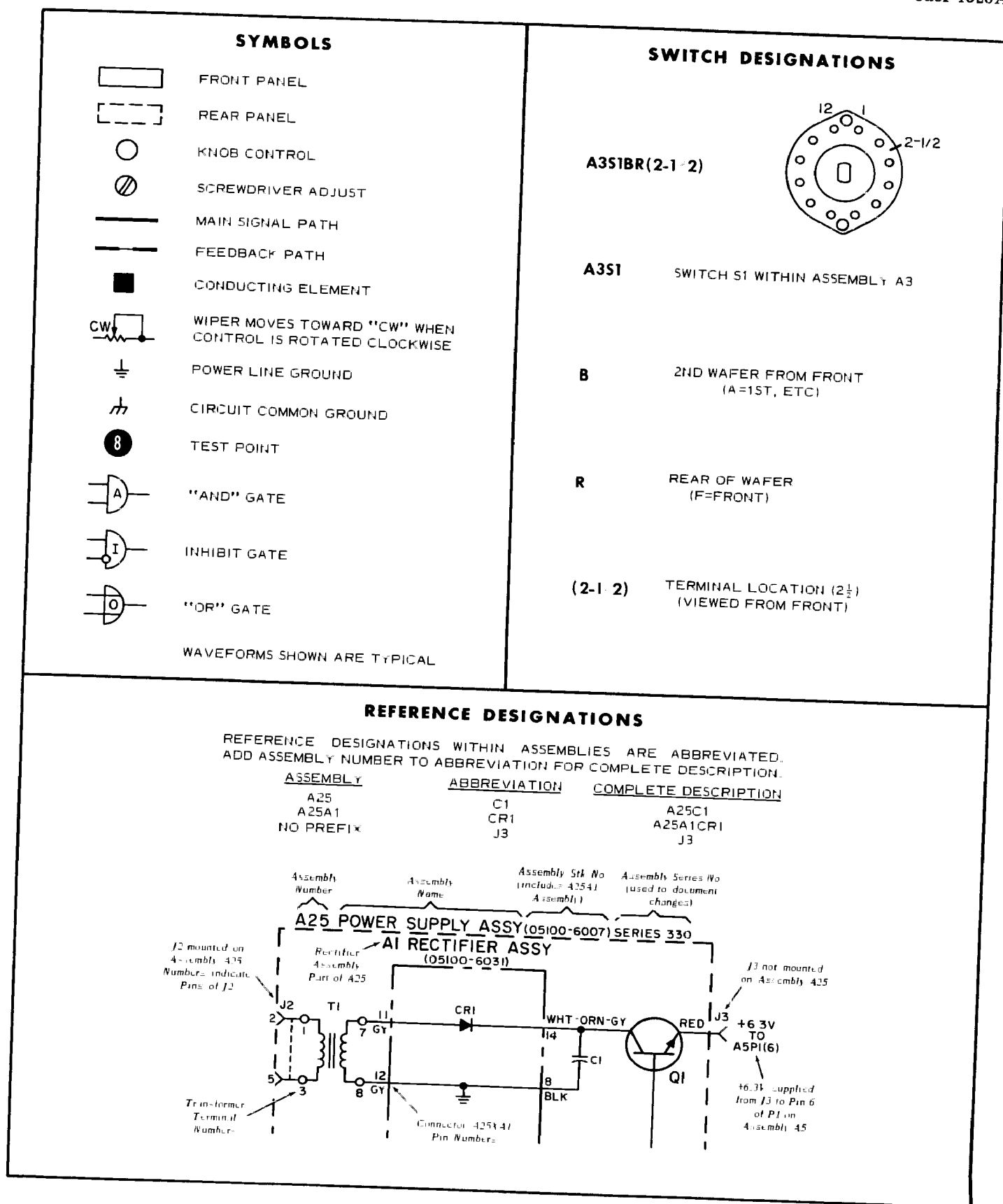
Figure 8-1 Schematic Diagram Notes
