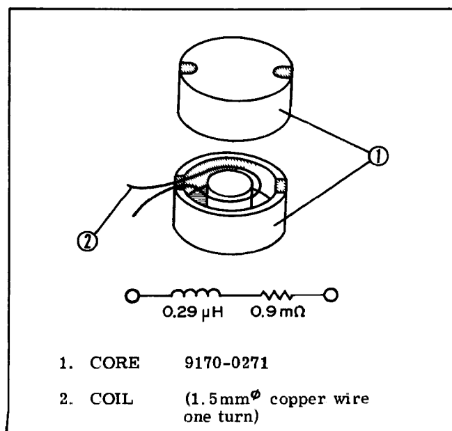
Figure 5-2. (0.9\text{m}\Omega + j1.8\text{m}\Omega) Impedance
