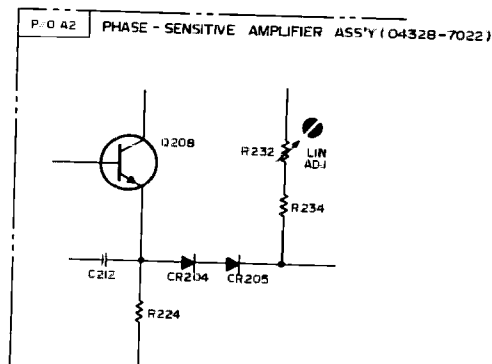
Figure 7-1. Partial Schematic of A2 Ass'y
