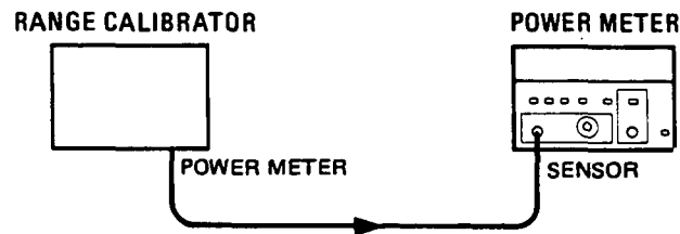
Figure 4-3. Calibration Factor Test Setup
