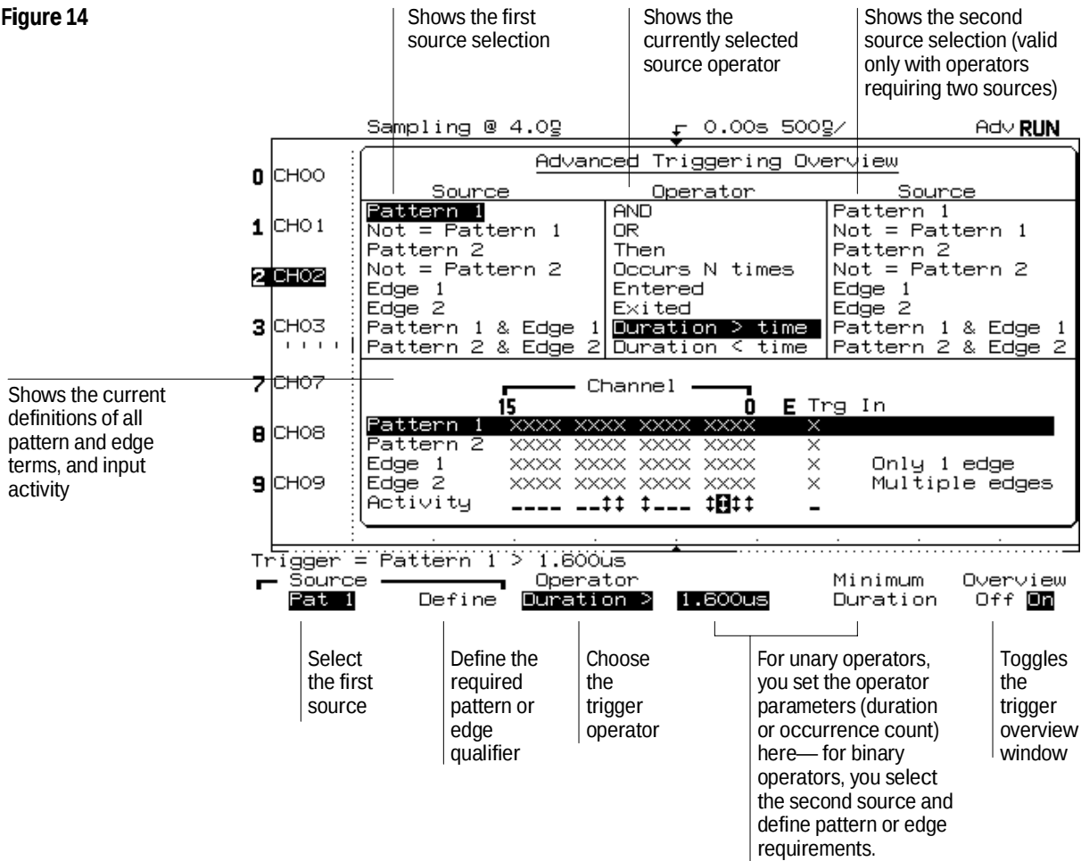
Advanced Trigger Setup (with Overview On)
