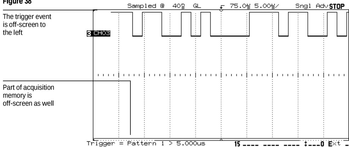
Single Acquisition, Time Reference Center, Positive Delay of 75 \mu\text{s}
