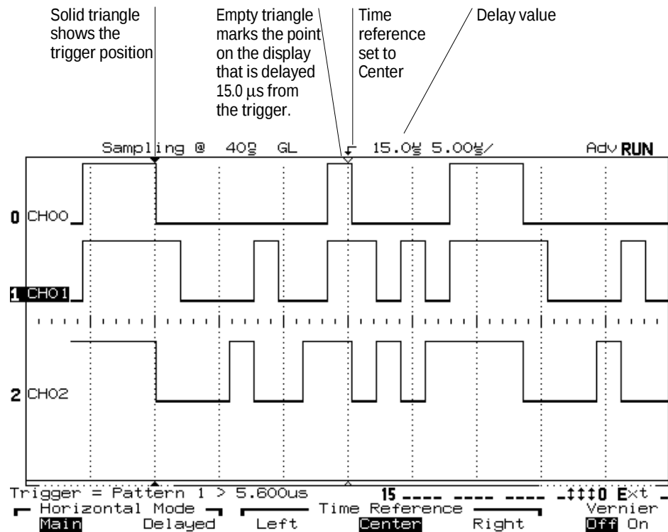
Time Reference at Center, Delay of 15 \mu s on Main Sweep
