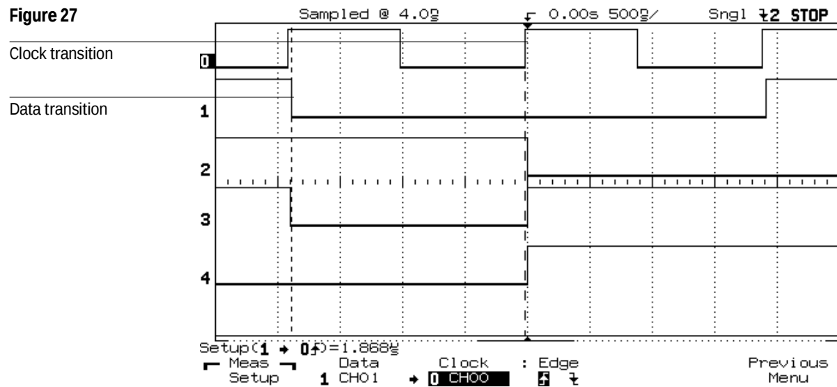
Setup Time Measurement
