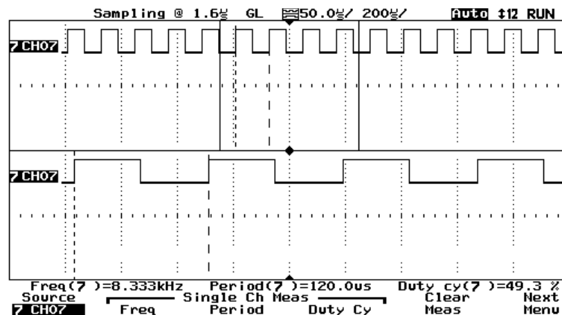
Waveform Display with Auto Glitch Detect Enabled
