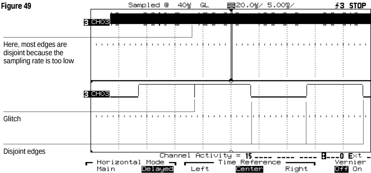
Waveform Display with Sampling Rate Too Low
