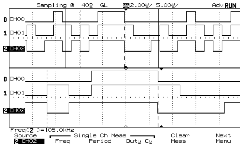
Measurement Within the Delayed Sweep Window
