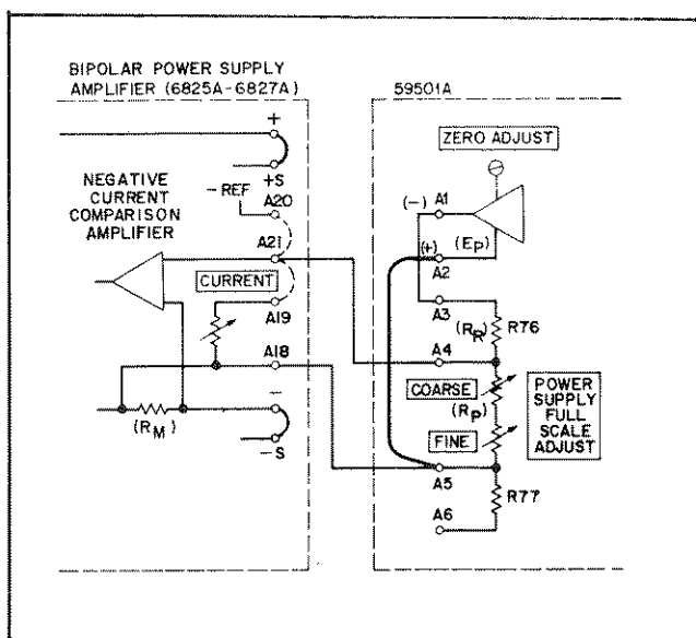
Figure 3-17. Negative CC Programming Connections for BPS/A's 6825A-6827A
