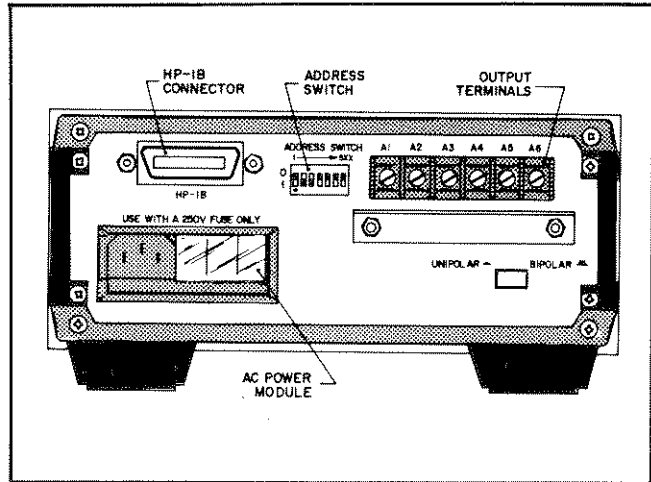
Figure 3-2. 59501A Rear Panel
