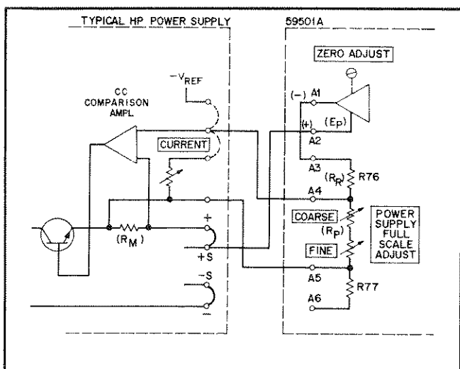
Figure 3-6. Typical Connections for CC Programming
