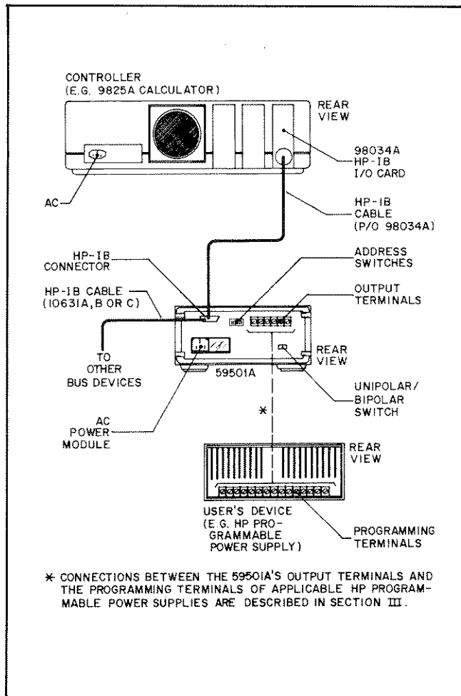
Figure 2-3. System Connections
