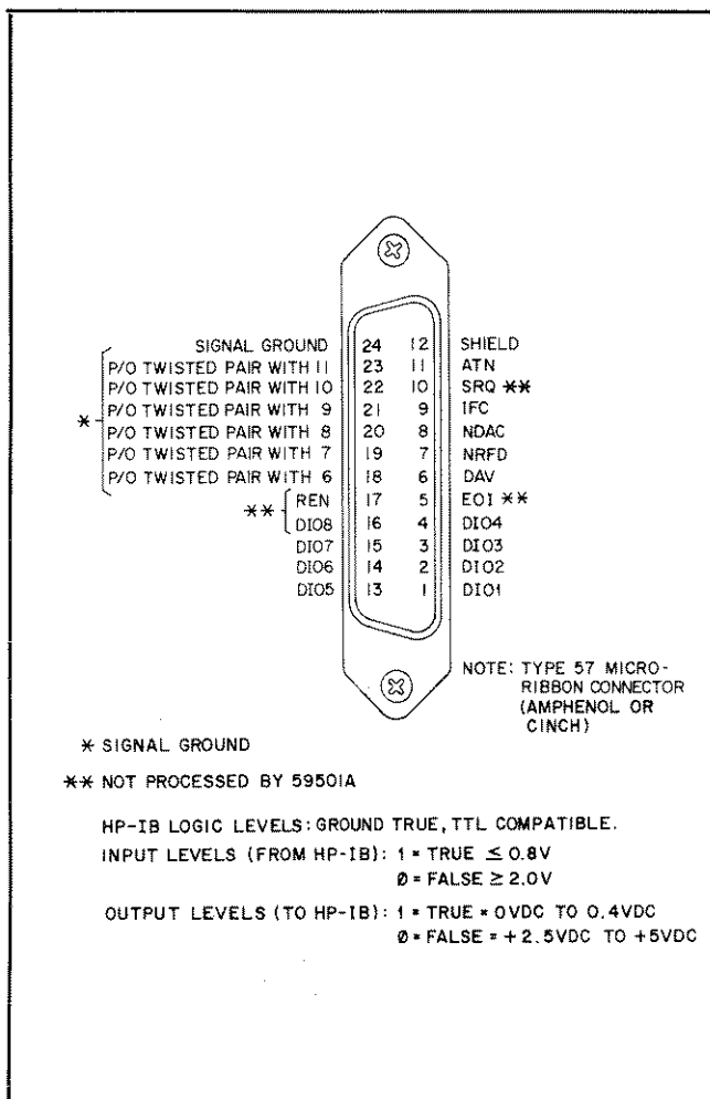
Figure 2-2. HP-IB Connector
