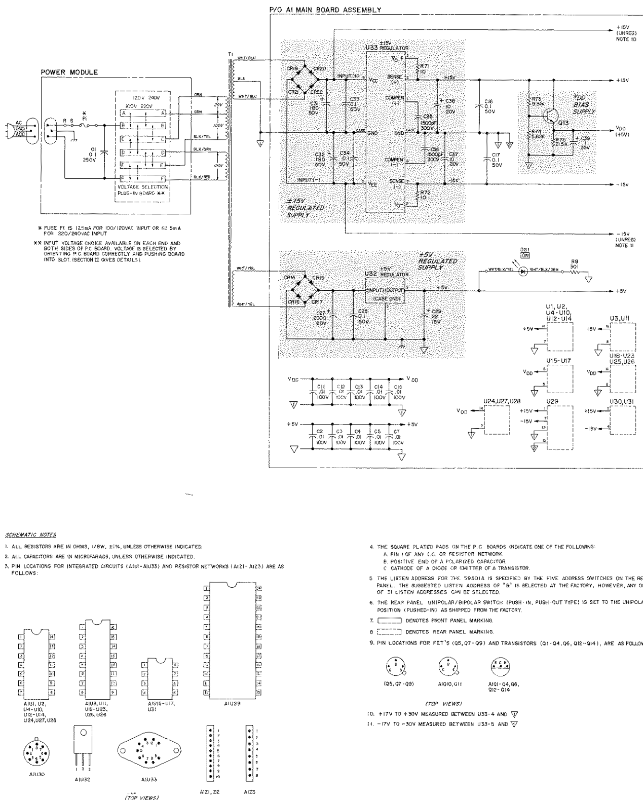
Figure 7-3 (Sheet 1). Model 59501A, Bias Voltage Supplies, Schematic Diagram
