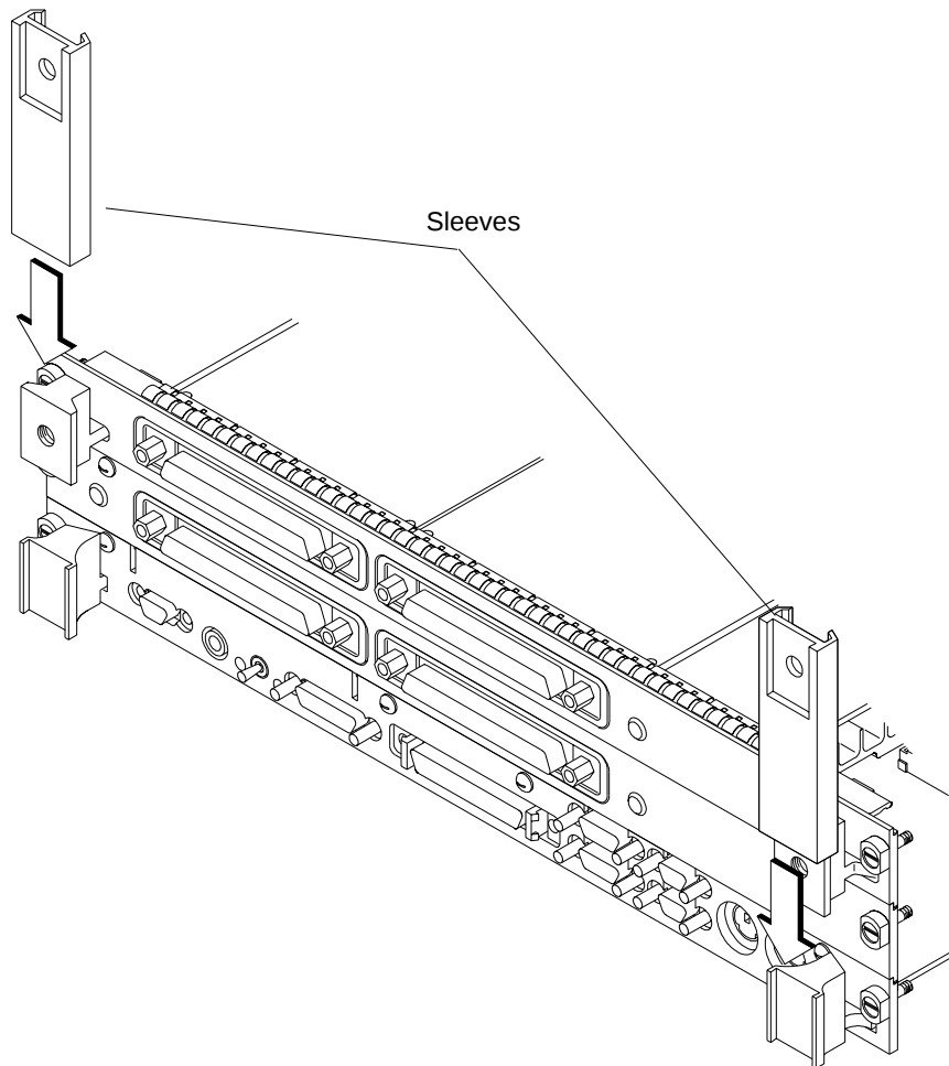
Figure 2-13 Installing Ejector Handle Sleeves
