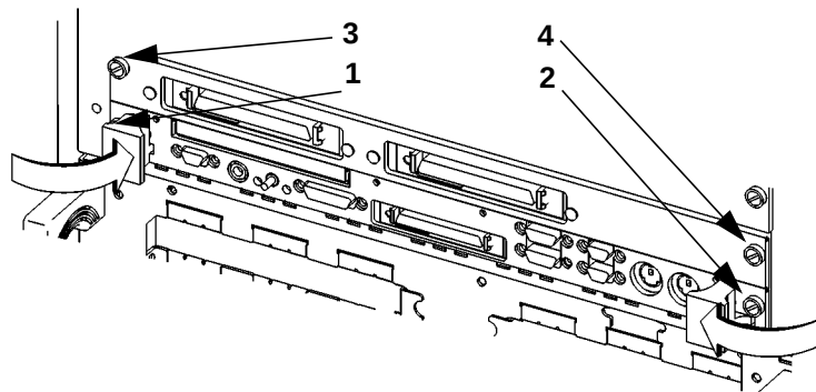
Figure 3-1 Board Computer Captive Screws
