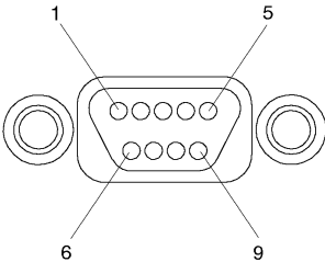
Figure 4-9 RS-232 Serial Connector
