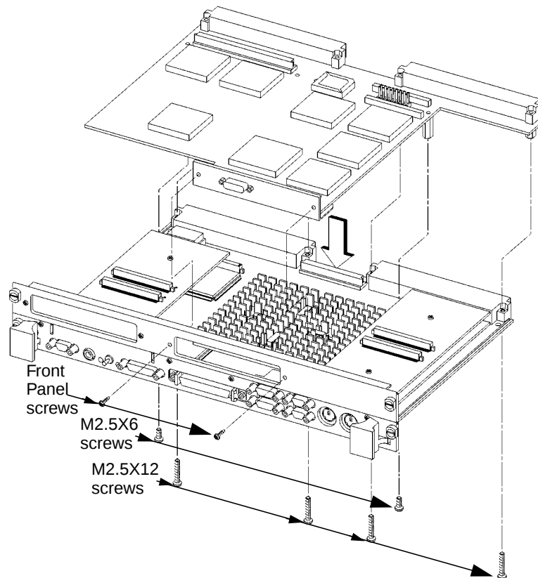
Figure 2-5 Installing an HCRX Graphics Board
