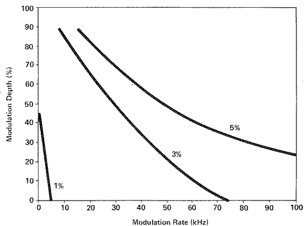
Typical AM Distortion (Center Frequency \geq 10 MHz)
