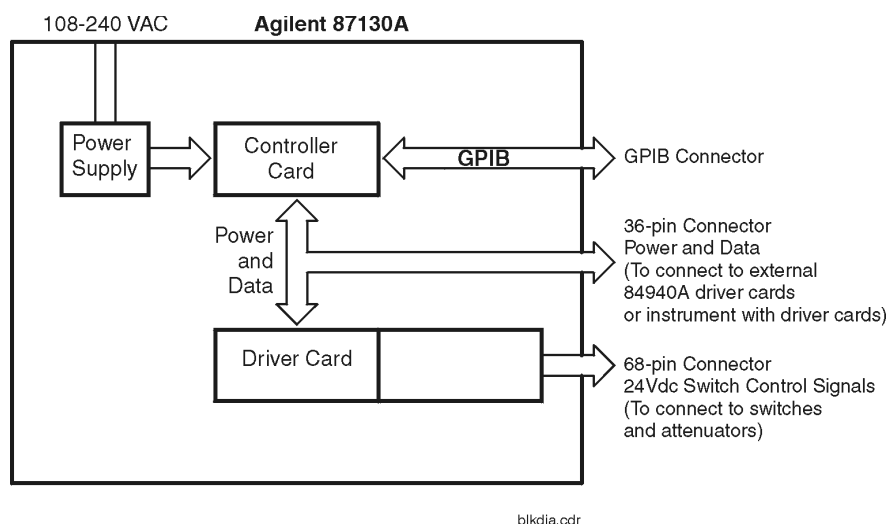
Figure 1-1 87130A Block Diagram
