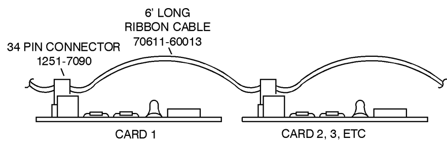
Figure 2-7 Daisy Chain of Driver Cards in Single Enclosure
