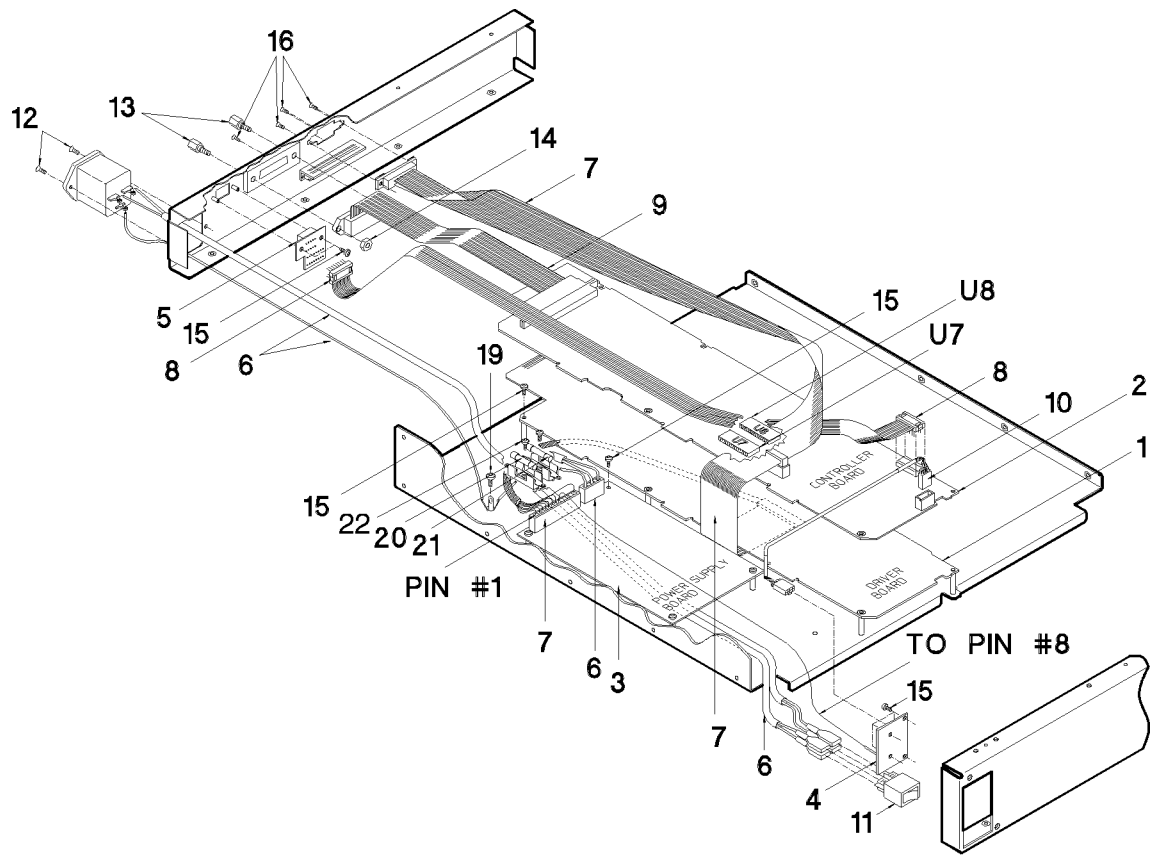
Figure 5-3 87130A Cable Assembly
