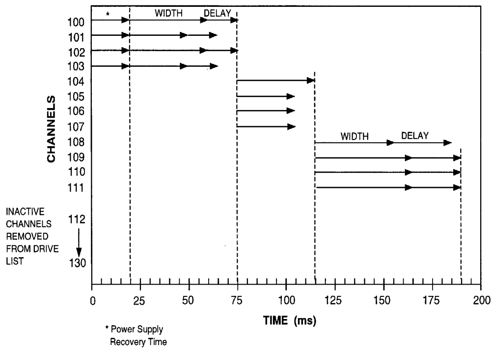
Figure 4-1 Timing Chart
