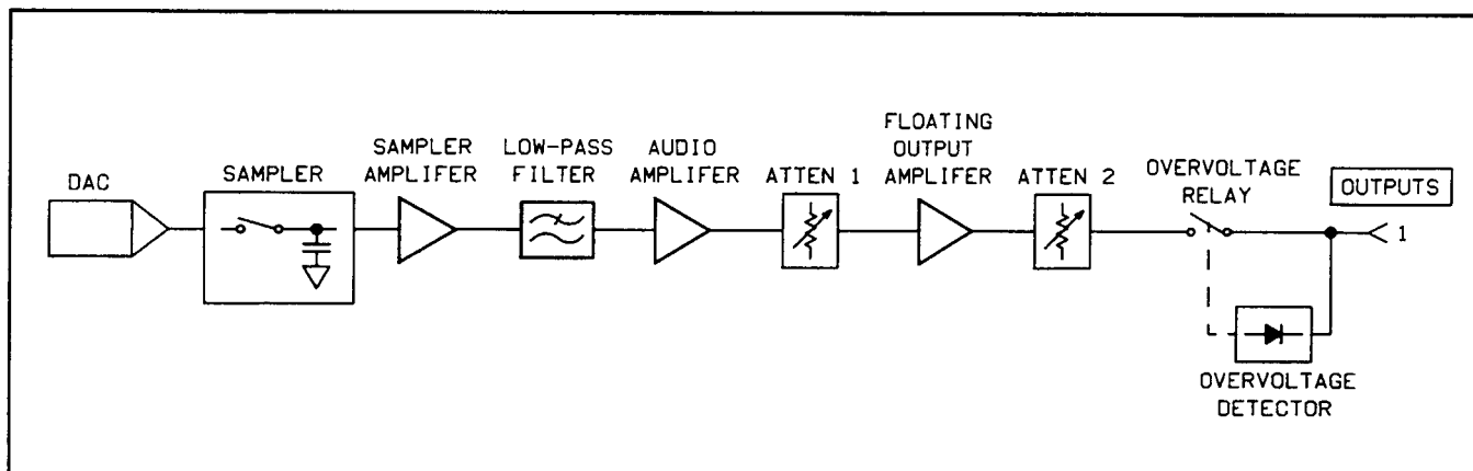
Figure 8-7. Analog Output Block Diagram
