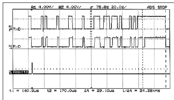
Figure 3: The time interval for this 12-bit sequence is 29.1 \mu s from the acknowledge bit to the next start bit.
