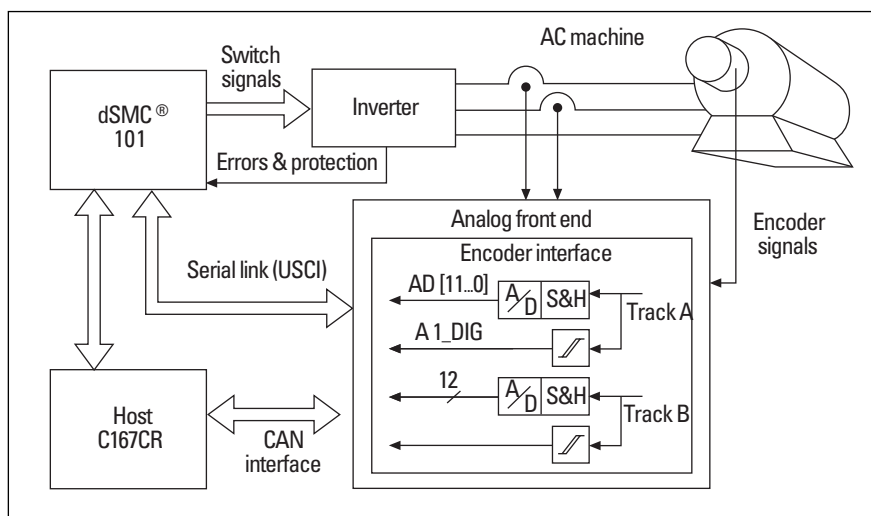
Figure 1: Block diagram of a high-precision position controller.
