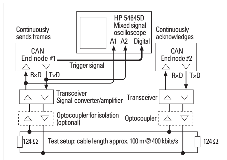
Figure 2: Test system configuration for cable length measurement; a mixed signal oscilloscope can measure both the analog and digital signals in this point-to-point CAN system. If the CAN network also includes optocouplers, we need to measure and account for their delay as well.
