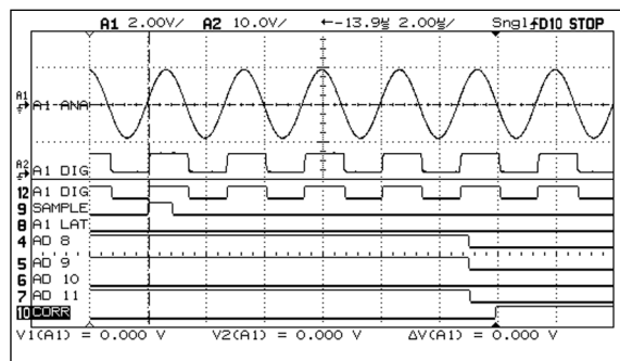
Figure 2: In this HP 54645D screen shot, signals AD 11 and A1 LAT give conflicting information about the sampled signal.
