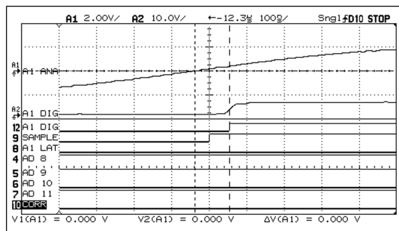
Figure 3: The cause uncovered: the sampling edge occurred immediately after the zero crossing.
