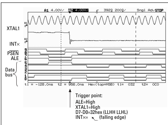
Figure 2: In this HP 54645D screen shot, a closer inspection of the external interrupt edge (analog line A2) relative to the RETI fetch (digital lines 0-7) and oscillator segment and phase reveals the offending condition.
