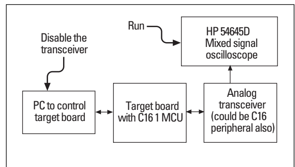
Figure 1: Measuring the transceiver disable time.
