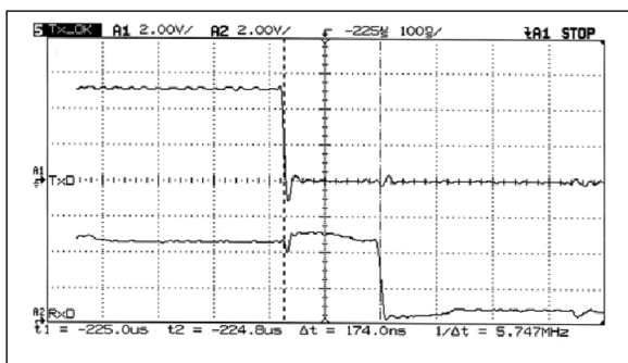
Figure 1: Signal propagation delay (Tx/D - Rx/D) through one transceiver is 174 ns (87 ns in each direction).
