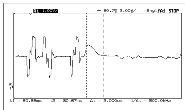
Figure 3: By panning and zooming, I found the trigger disable time—an event only 2 \mu s long.
