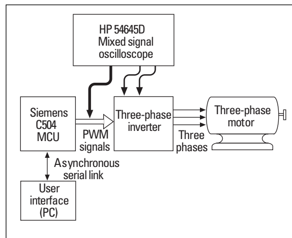
Figure 1: Block diagram of an open-loop configuration for generating safe PWM signals to drive a three-phase motor.
