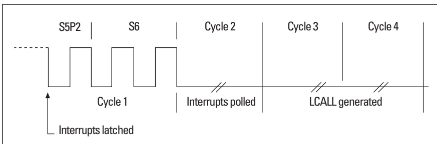
Figure 1: The CPU timing diagram shows why LCALL gets blocked after the RETI command is generated.
