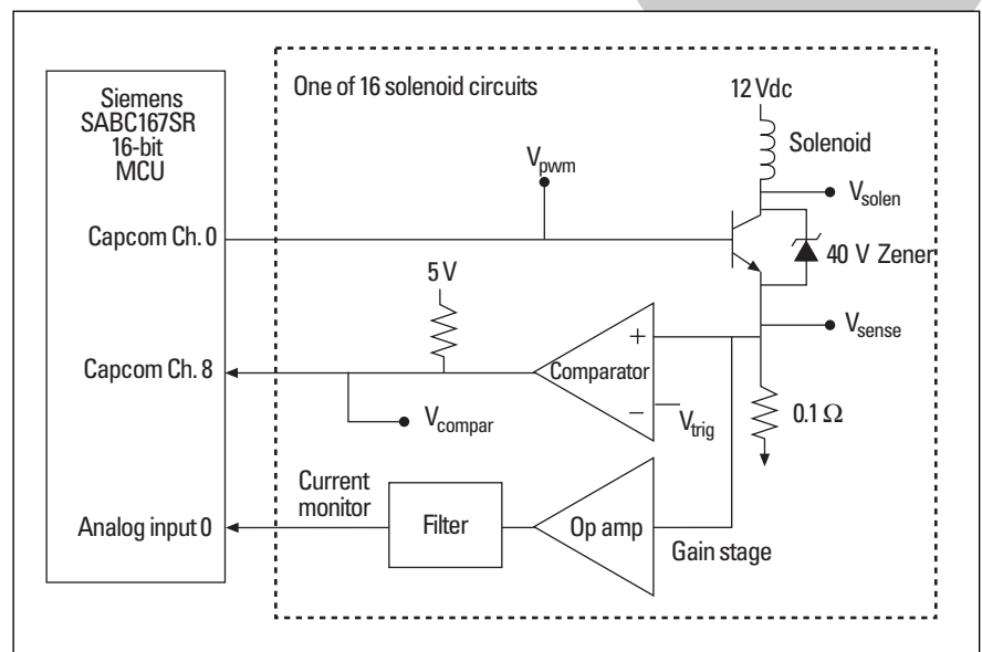
Figure 1: The capcom channels are individually programmed for "input capture" and "output compare" functions, which drive each solenoid and sense the peak current threshold, respectively. Capcom channel 0 drives a power transistor; the sense resistor at the emitter leg is for current monitoring. The op-amp conditions this signal and provides feedback to Analog Input 0, which monitors the holding current. The comparator signals when peak current is reached.
