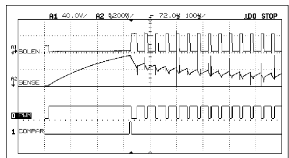
Figure 2: Four key signals from Figure 1. SOLEN is an analog signal from the low side of the solenoid; the zener diode clamps inductive spikes at 40 V. SENSE, measured across a 0.1 \Omega resistor, peaks around 380 mV, which corresponds to 3.8 A PWM drives the power transistor. The initial 300 \mu s pulse is the time required to achieve peak current. COMPAR triggers at 380 mV across the sense resistor and is fed into capcom channel 8 to signal the MCU to enter hold mode until the solenoid is turned off.
