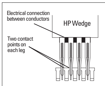
Figure 1: The HP Wedge inserts between adjacent pairs of pins on a fine-pitch IC package, providing secure, redundant, mechanically noninvasive contact.
