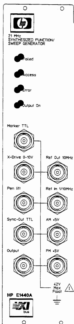
Figure 1-2. HP E1440A Front panel
