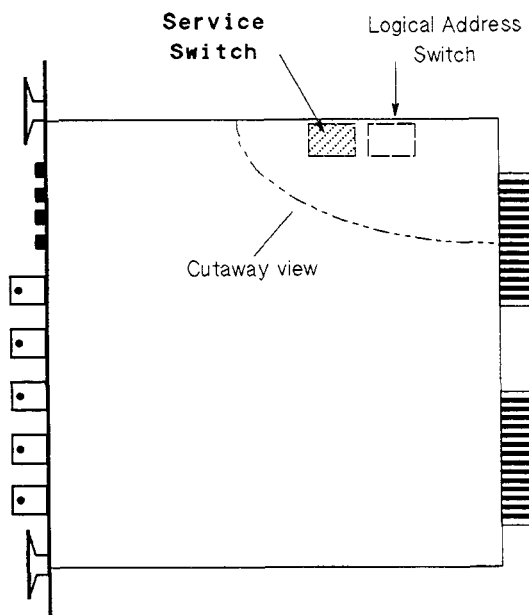
Figure C-1. Service Switch
