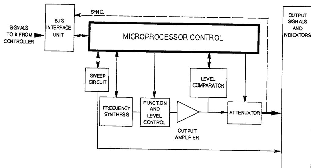
Figure 1-1. Block Diagram of the HP E1440A
