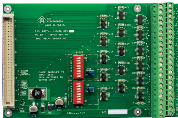
xx03DVR Relay Driver Board, P/N 115490
