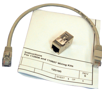
ICS Wiring Kit with 1 foot cable
