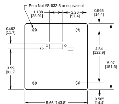
Remote Mounting Front Panel (rear view) in [mm]
