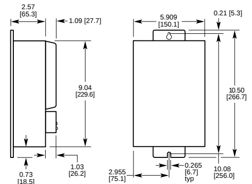
Minimum Depth Mounting Dimensions in [mm]
