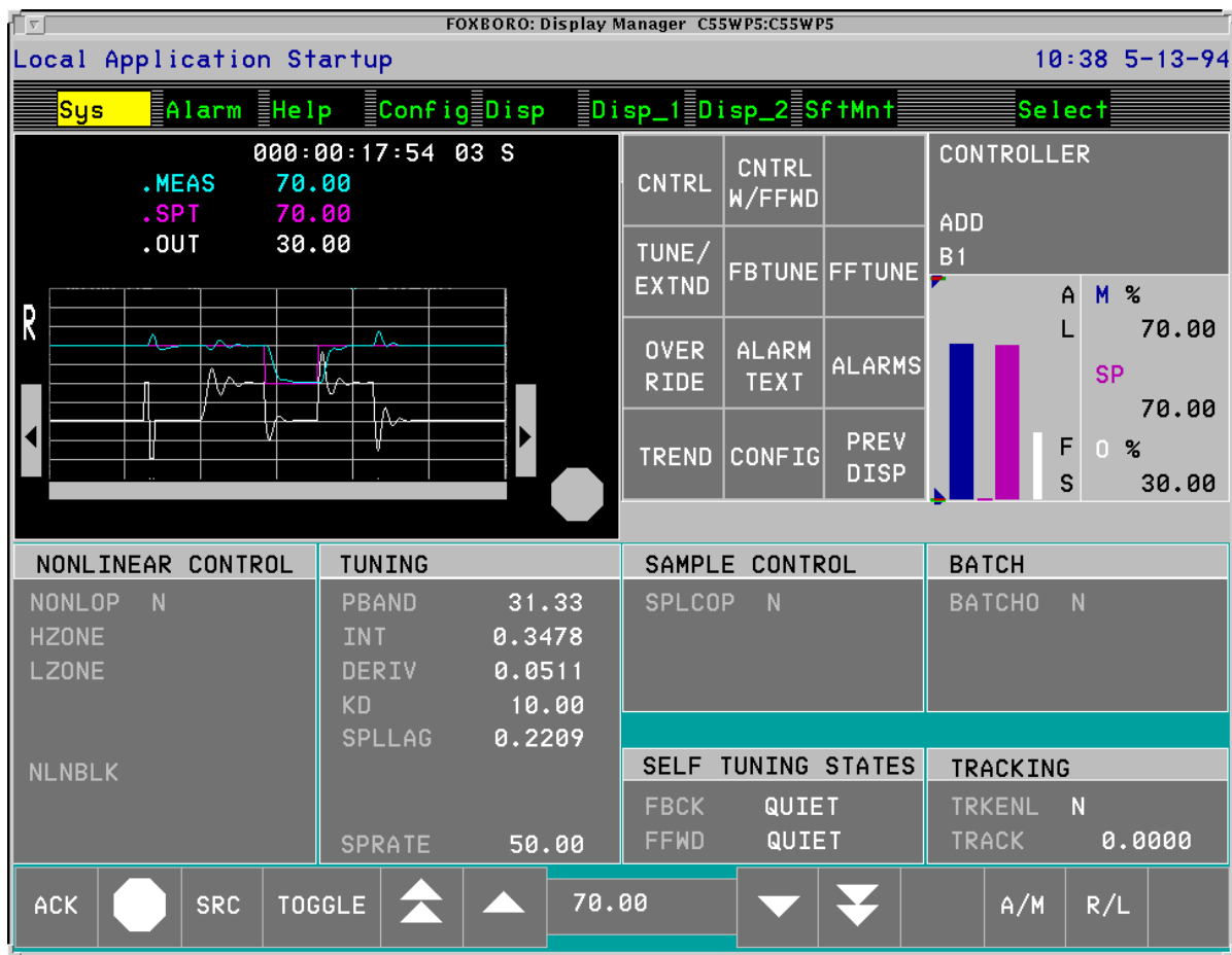
Figure 6. Example of PIDA Block Detail Display
