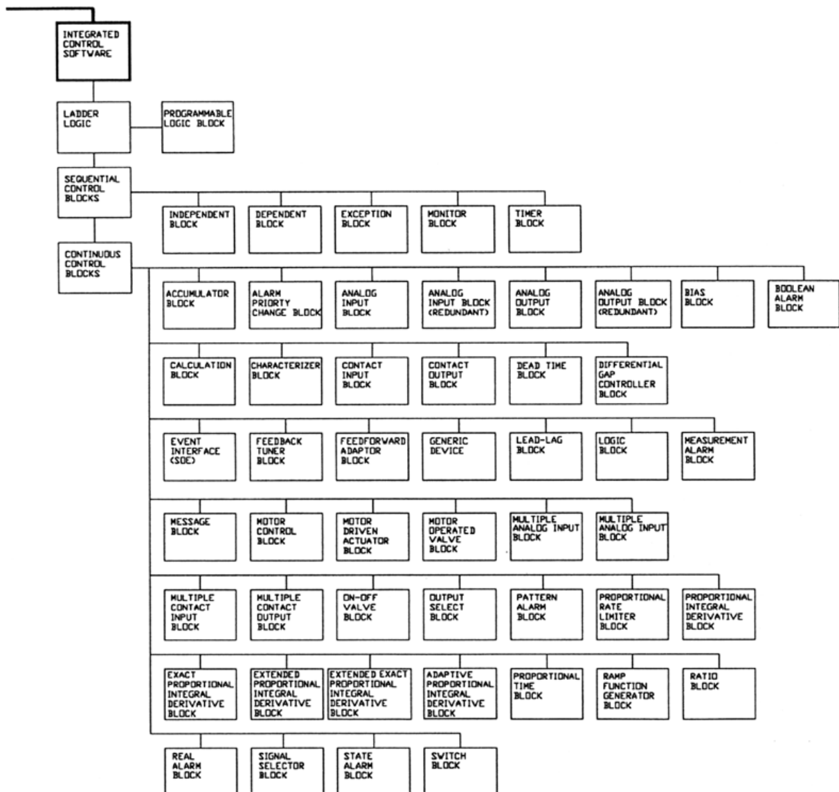
Figure 2. Integrated Control Blocks
