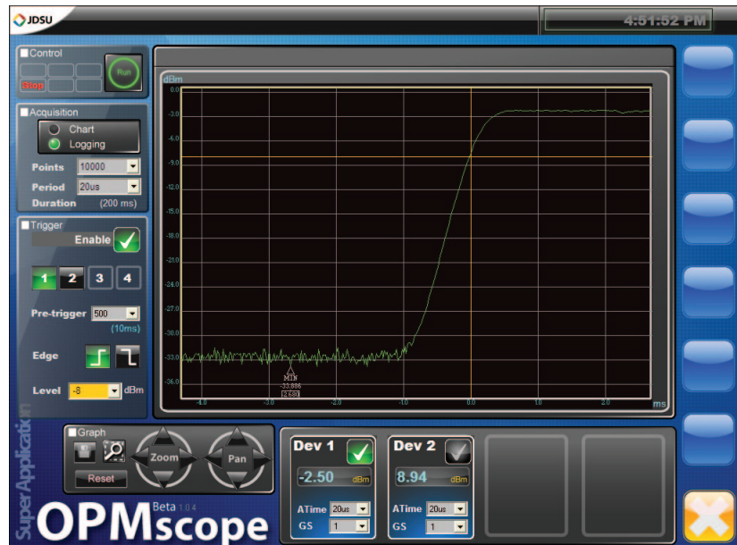
Figure 2. OPMscope main user interface
