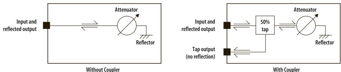
Optical Configurations for the Variable Backreflector Cassette
