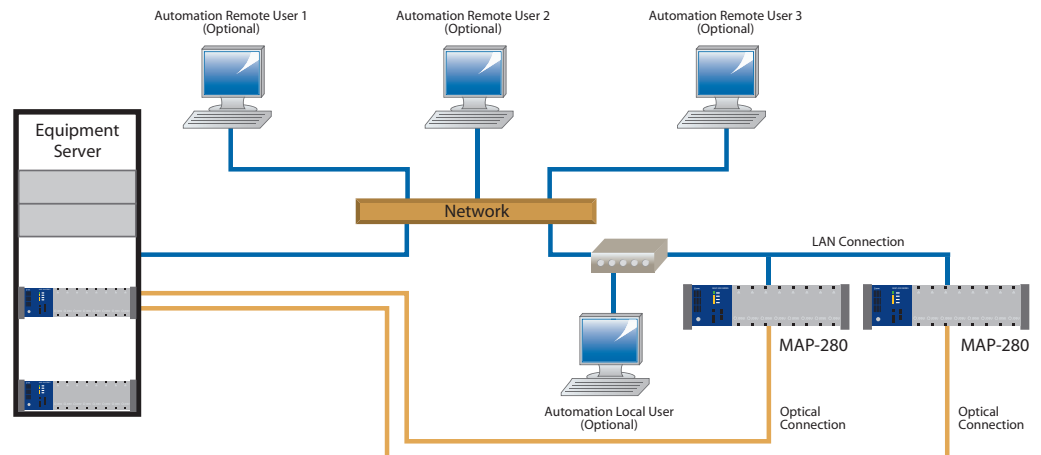
Figure 3 MAP implementation within a shared resource environment
