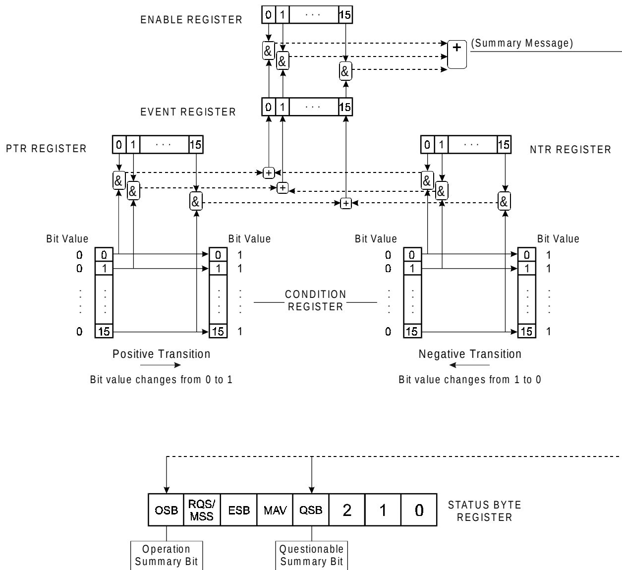
Figure 8: Data Structures
