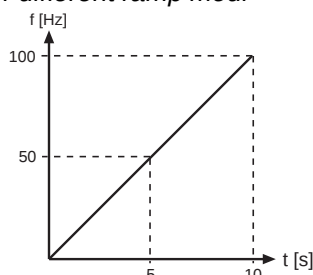
Picture 6.4.6.b Example for different ramp modi
