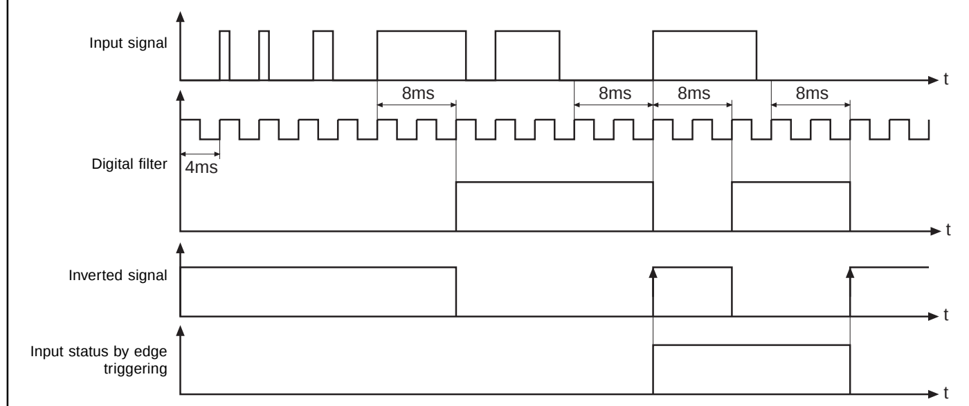
Picture 6.3.7 Example of a signal transit-plan for Input I1 (di.0=2; di.2=16; di.14=16)
