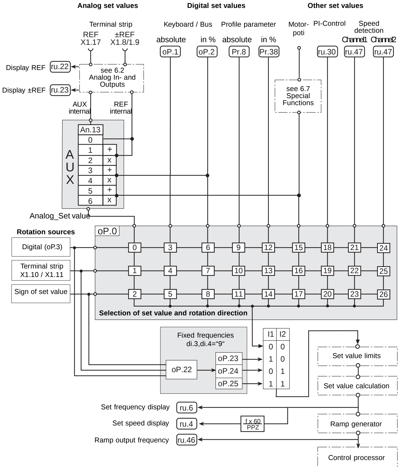
Picture 6.4.2 Set value and AUX-function
