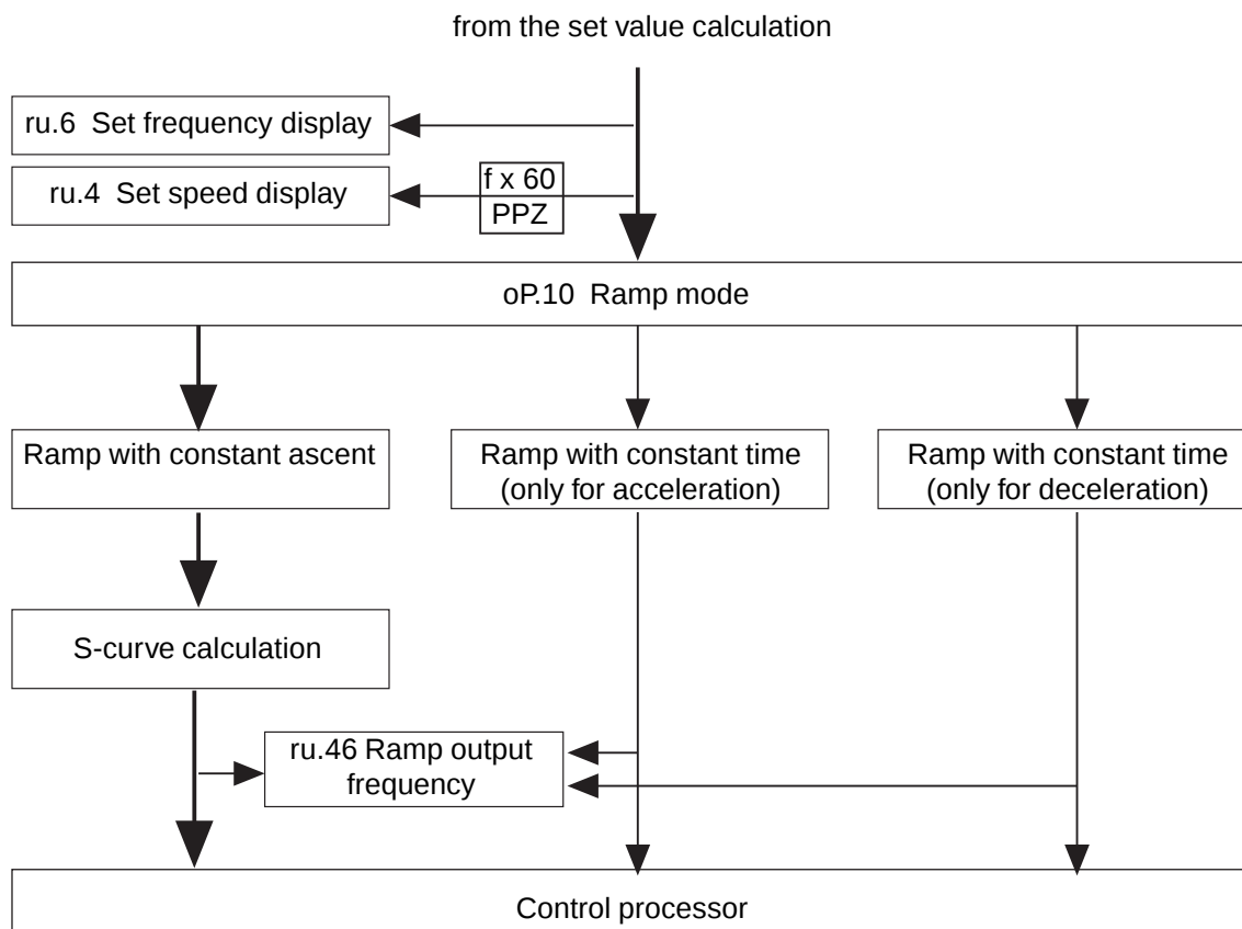
Picture 6.4.6.a Survey of ramp generator
