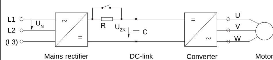
Picture 2.1.2 Block diagram of an inverter power circuit
