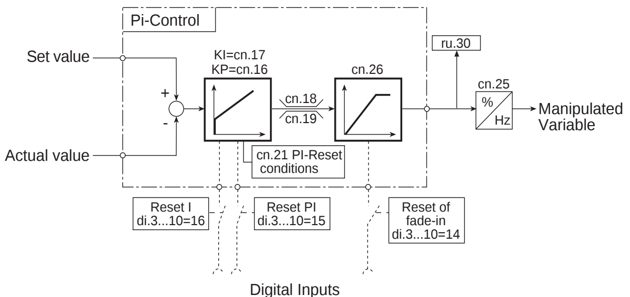
Picture 6.11.1 PI-Controller
