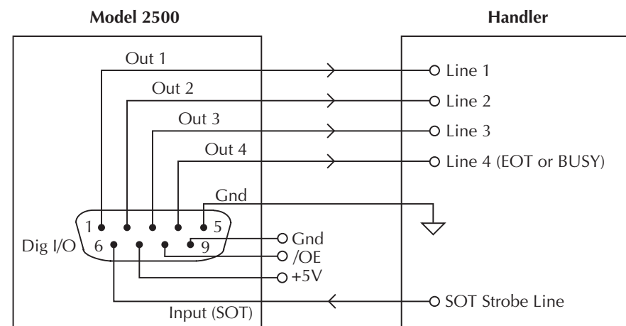
Handler interface connections
