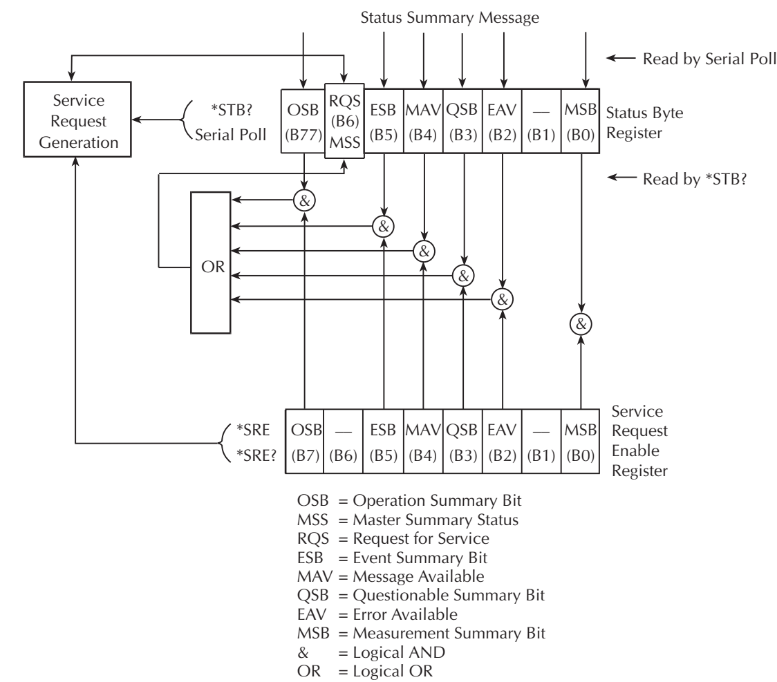
Figure 14-3 Status byte and service request (SRQ)
