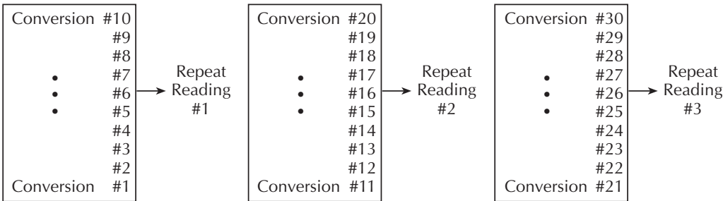
Figure 6-3 Repeat filter (count 10)
