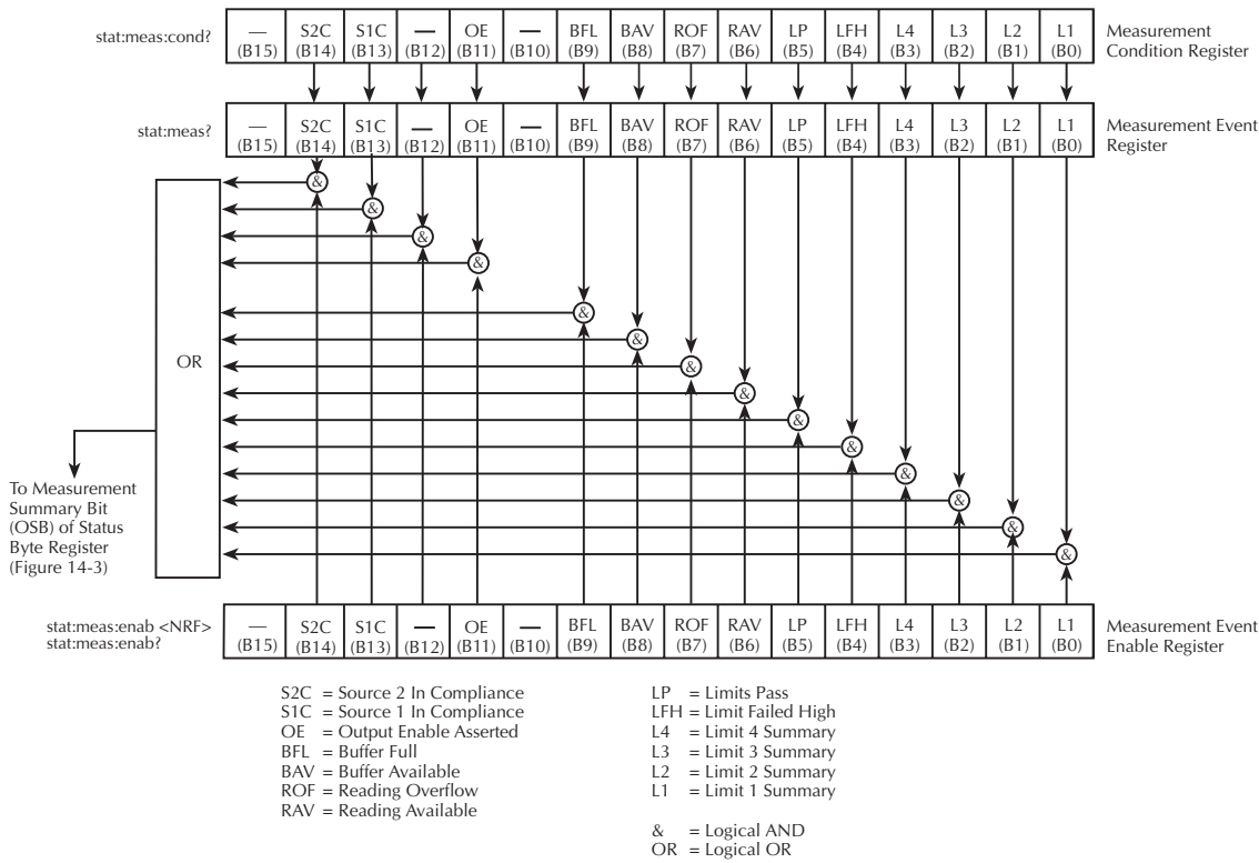
Figure 14-6 Measurement event status
