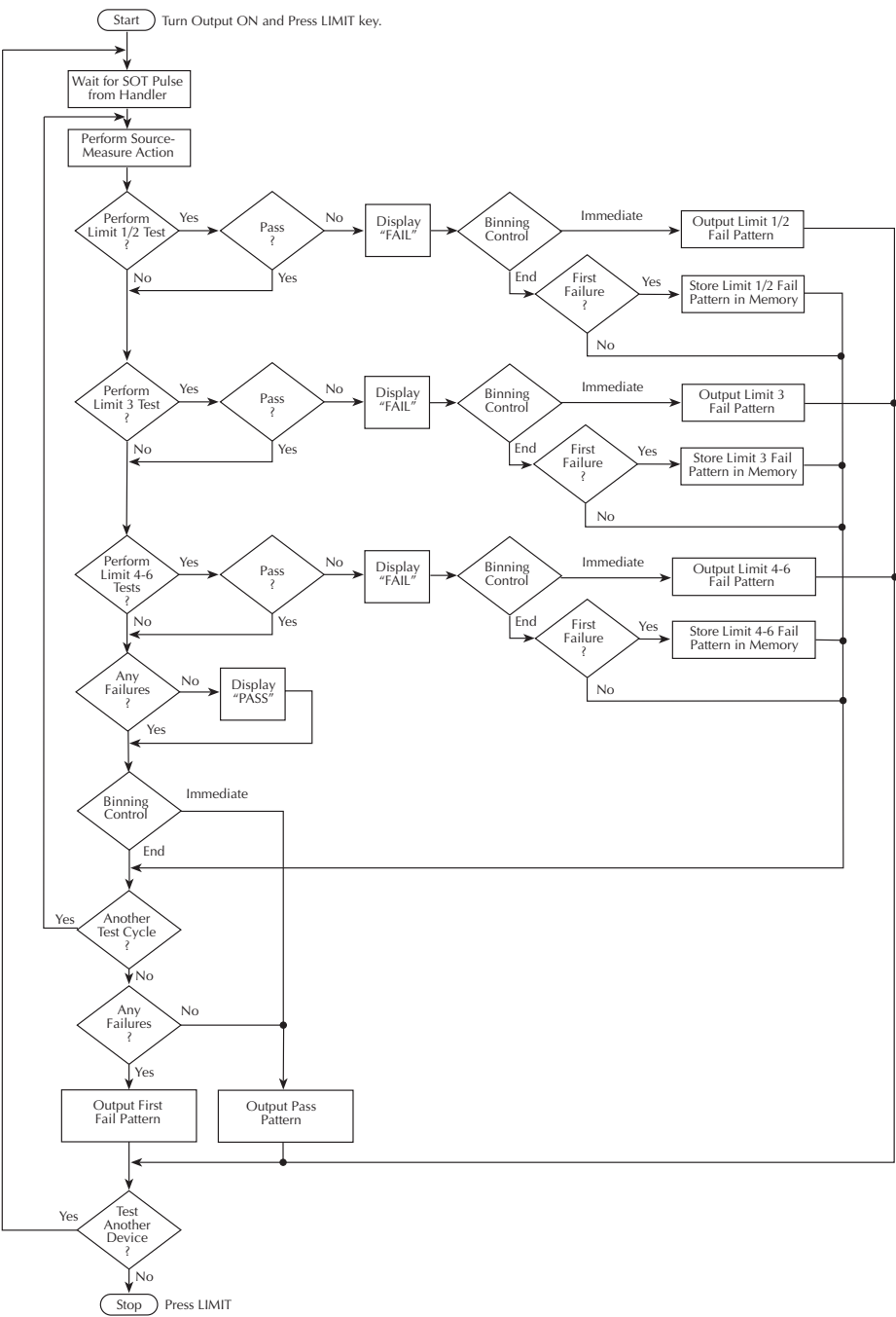
Figure 11-2 Grading mode limit testing
