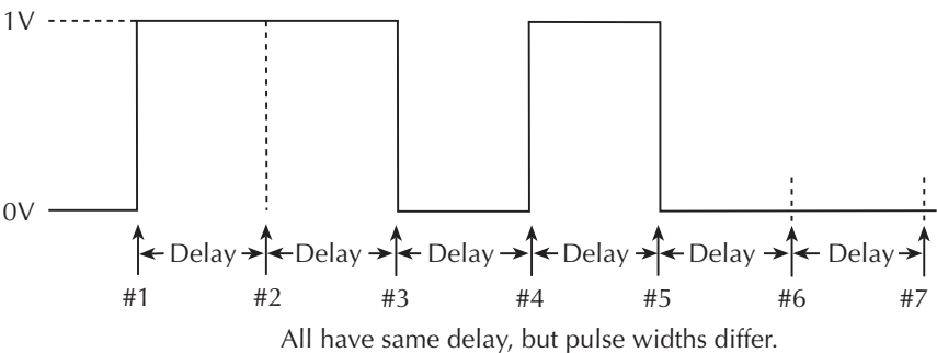
Figure 9-4 Custom sweep with different pulse widths
