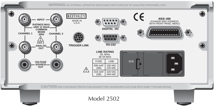
Figure 1-3 Model 2502 rear panel
