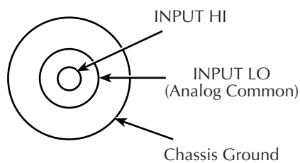
INPUT Triax Connector
