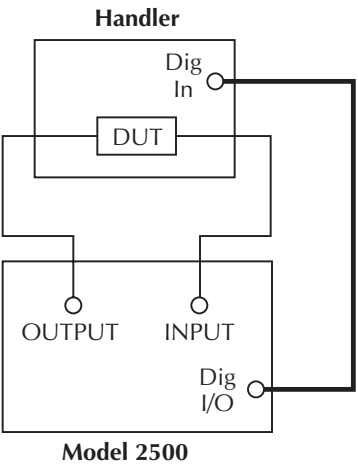
Figure 11-7 Binning system—single element devices
