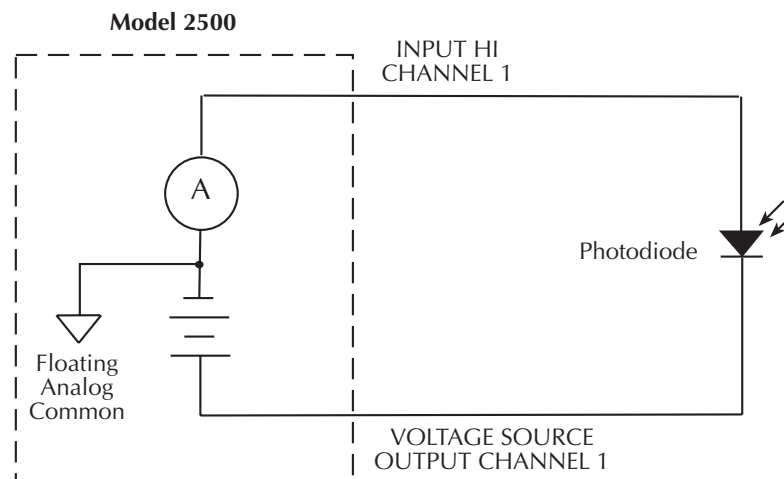
Circuit configuration for photodiode measurements
