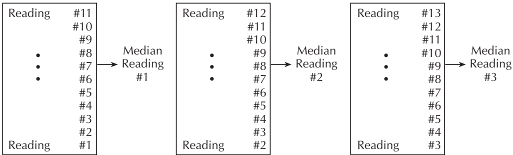
Figure 6-4 Median filter (rank 5)
