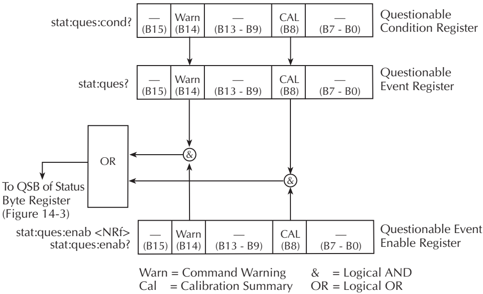
Figure 14-7 Questionable event status
