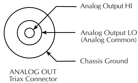
Figure 2-9 Analog output connector terminals
