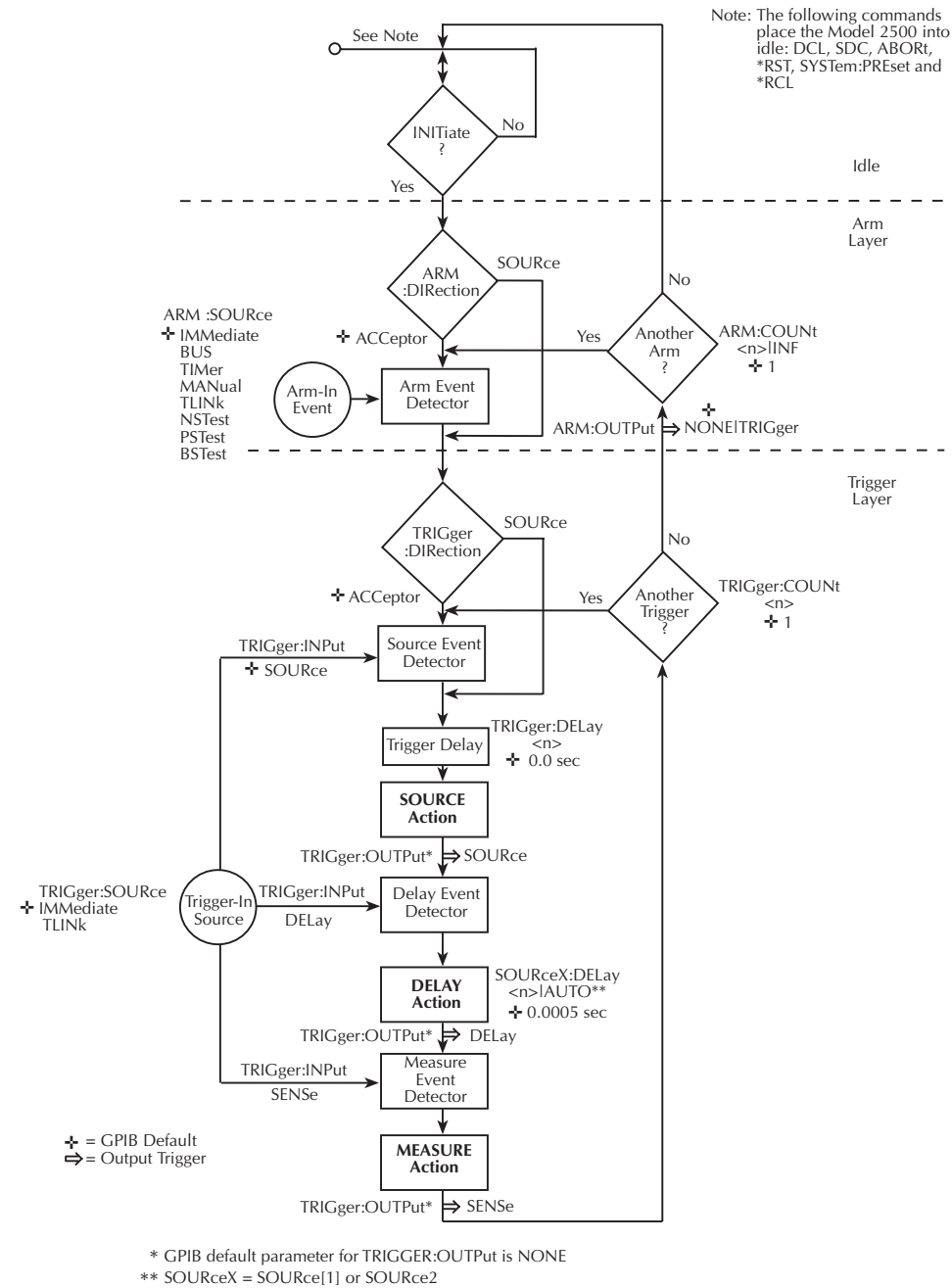
Figure 10-9 Trigger model (remote operation)
