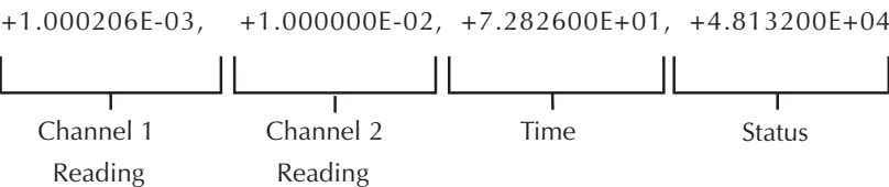
Figure 17-1 ASCII data format
