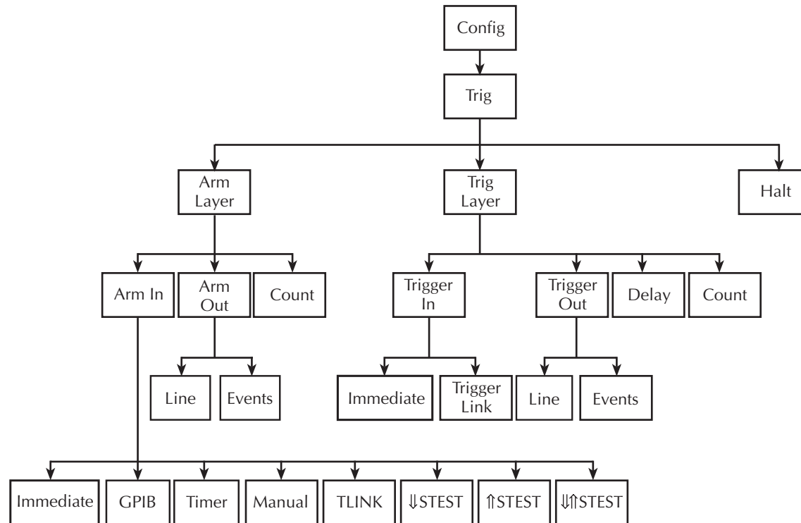
Configure trigger menu tree
