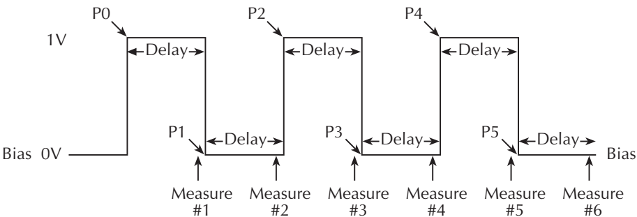
Figure 9-3 Custom pulse sweep
