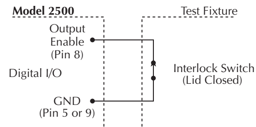
A. Model 2500 OUTPUT can be turned on.
