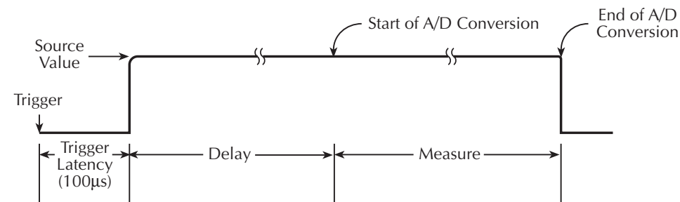
Source-delay-measure (SDM) cycle
