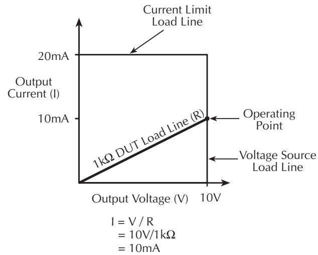
Figure 5-5 Loading effects
