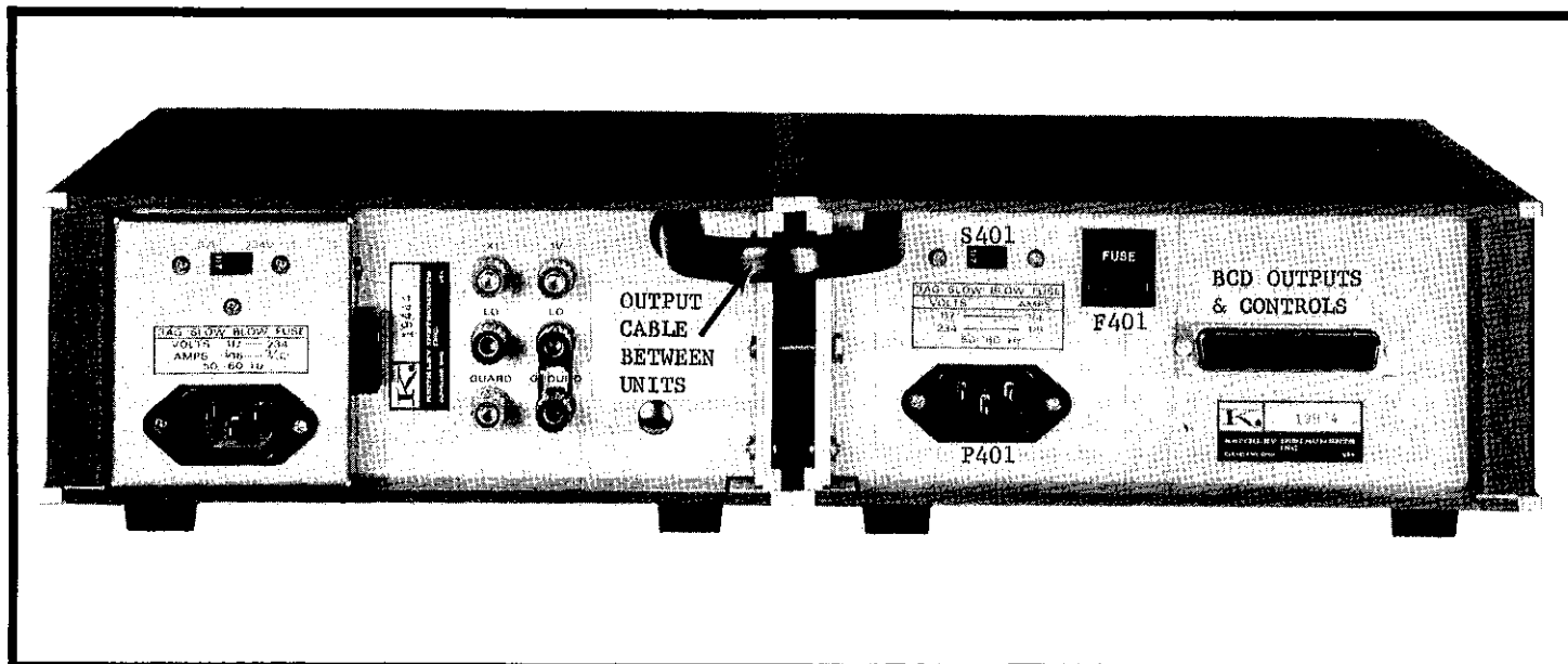
FIGURE 17. Rear Panel of Model 616 and 6162.
