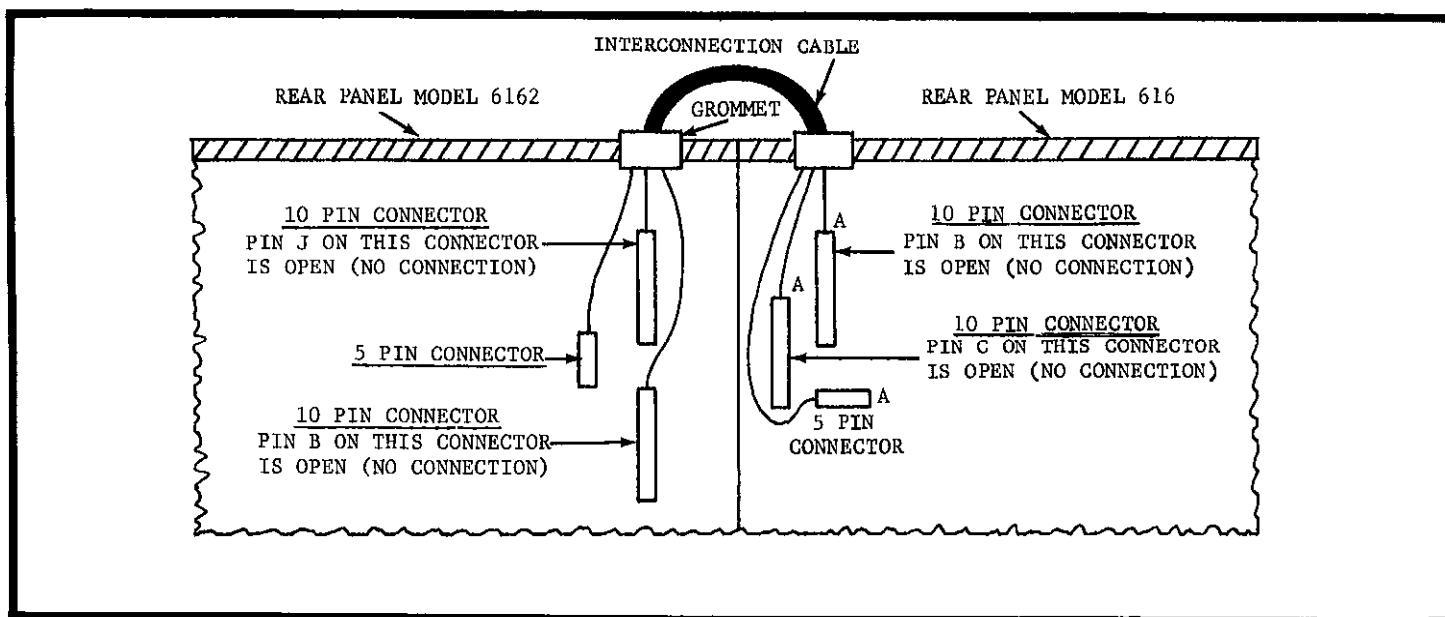
FIGURE 18. Diagram of Interconnection Cable Between 616 and 6162.
