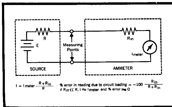
FIGURE 8. Loading Effects in Ammeter Function.
