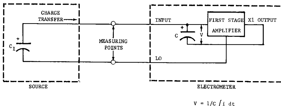
FIGURE 10. Operation As A Coulombmeter in FAST Mode.
