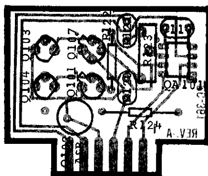
FIGURE 39. Component Layout, PC-361.
