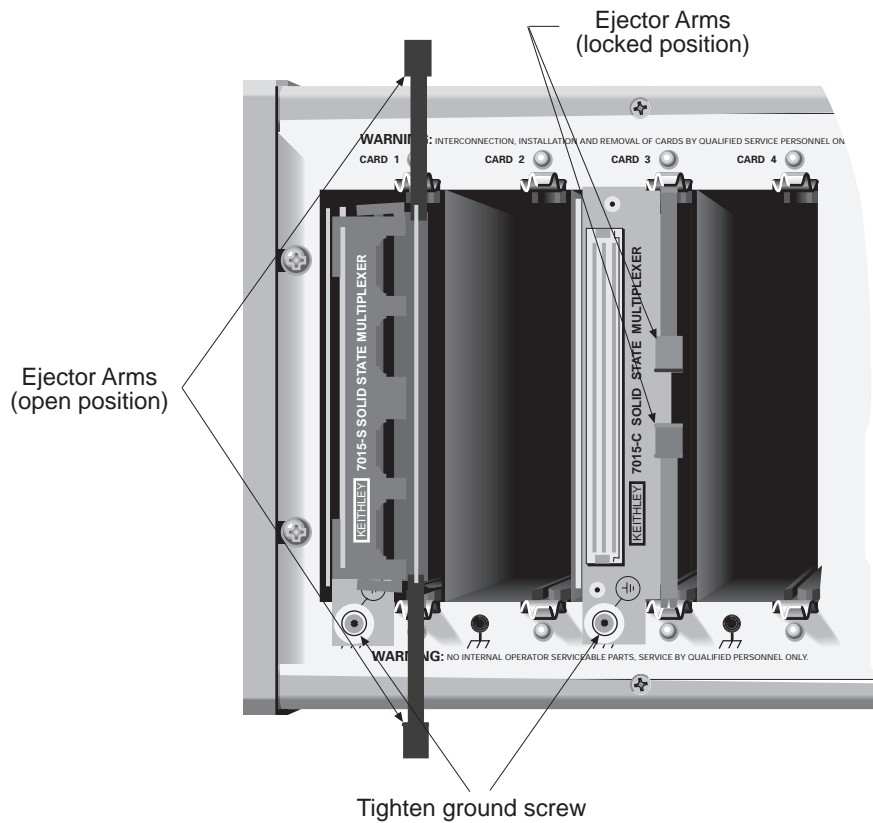
Figure 3-18 Model 7015 card installation in Model 7002
