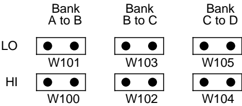
Figure 3-2 Bank-to-bank jumper terminal identification
