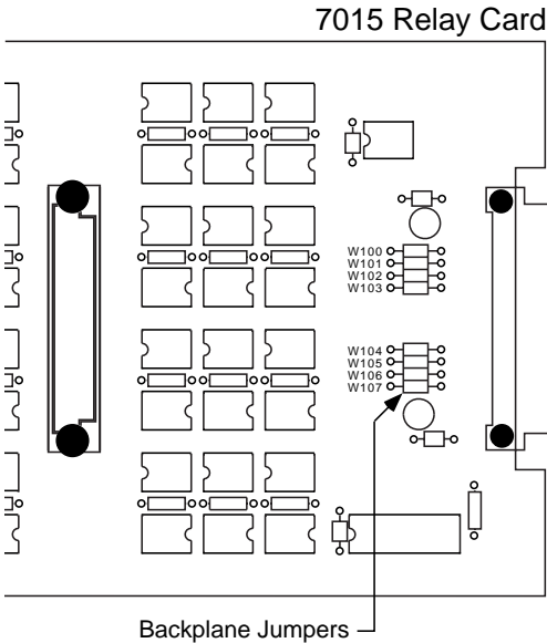
Figure 3-4 Backplane jumpers
