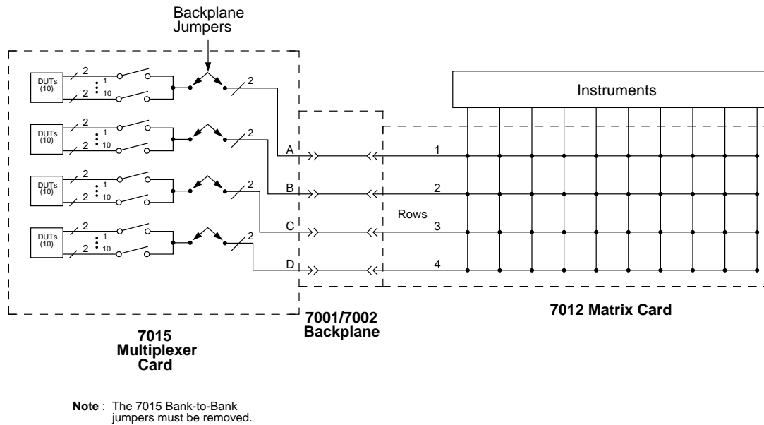
Figure 4-8 Connecting multiplexer and matrix cards together
