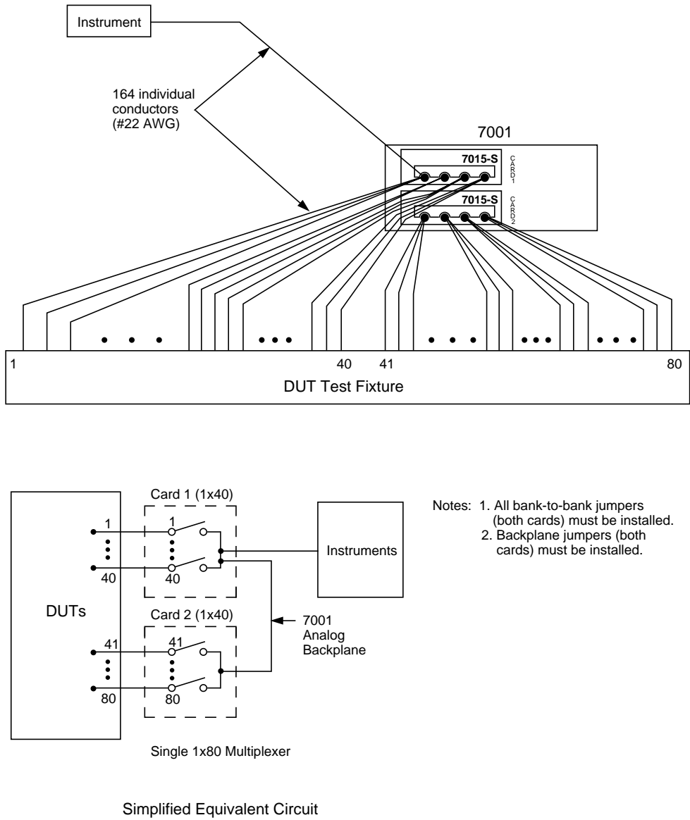
Figure 3-14 Two-card system example (screw terminal connector card)
