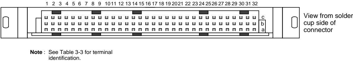
Figure 3-9 Model 7011-MTR connector pinout
