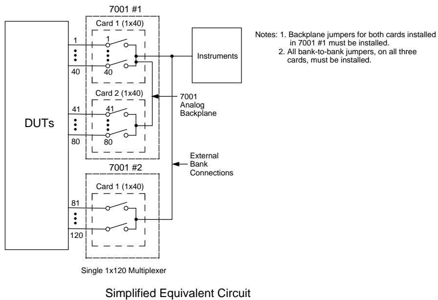
Figure 3-15 Two-mainframe system example (multi-pin connector card)
