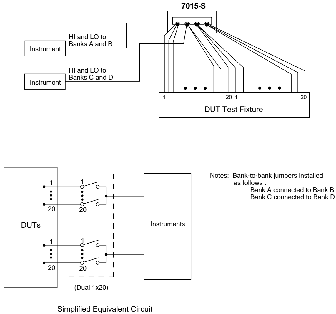
Figure 3-12 Single-card system example (screw terminal connector card)
