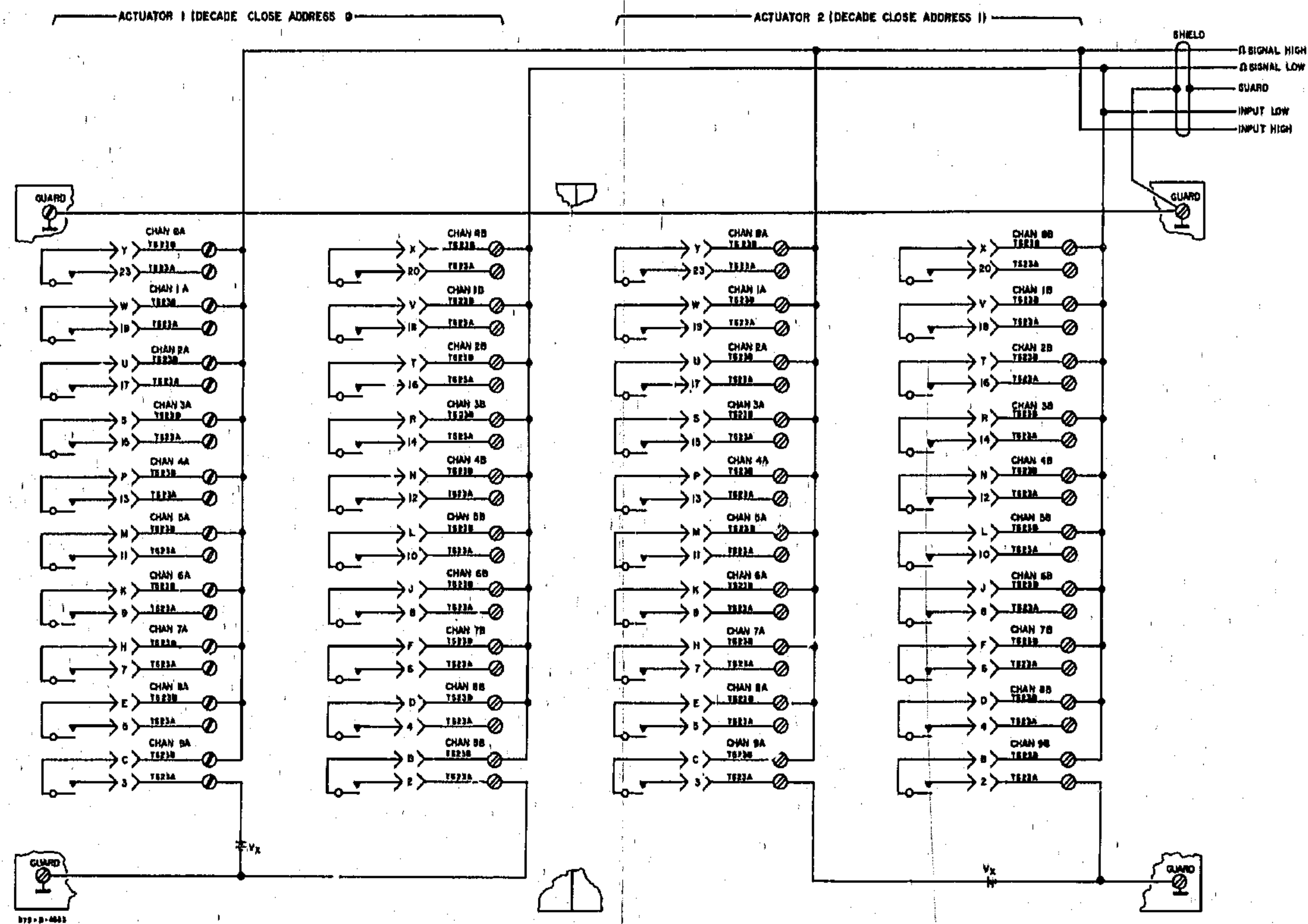
Figure 3-12. Functional Diagram of Voltage Scanning (Option 002). 3-17/3-18
