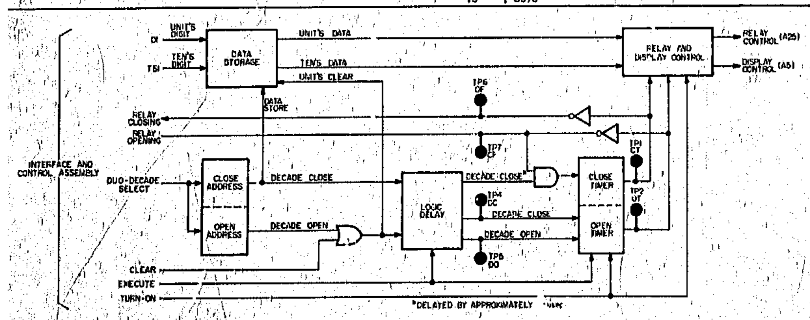
Figure 7-D-7. A40 Block Diagram.
