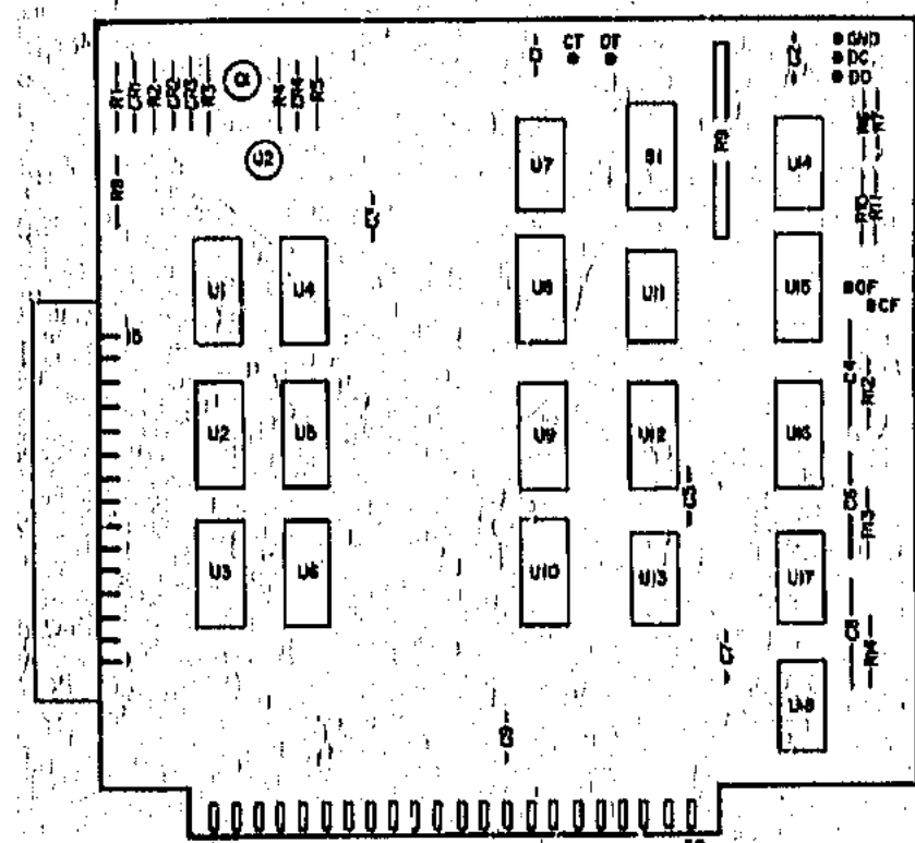
Figure 7-D-6. A40 Component Location.
