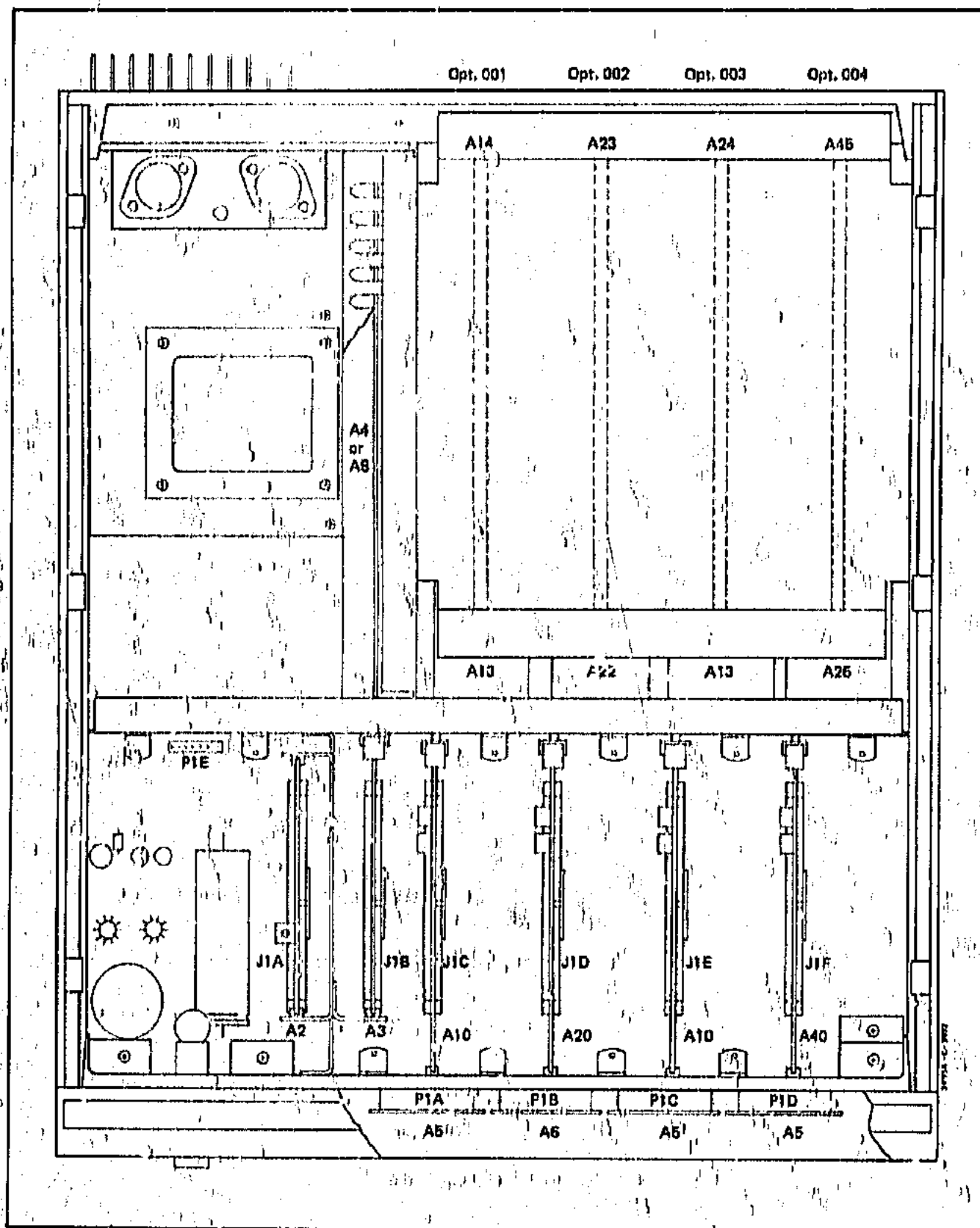
Figure 2-2. Location of Option Assemblies.
