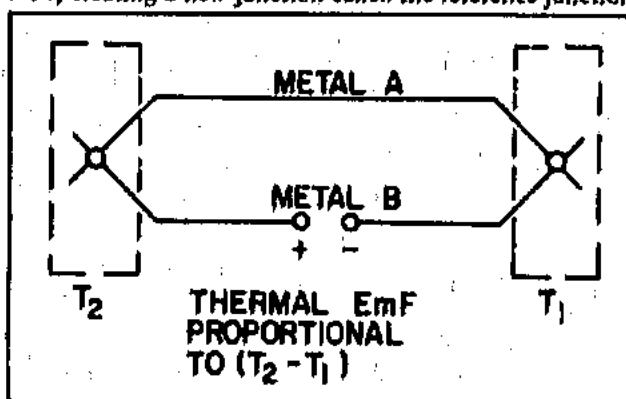
Figure 3-14. Thermocouple Circuit.
