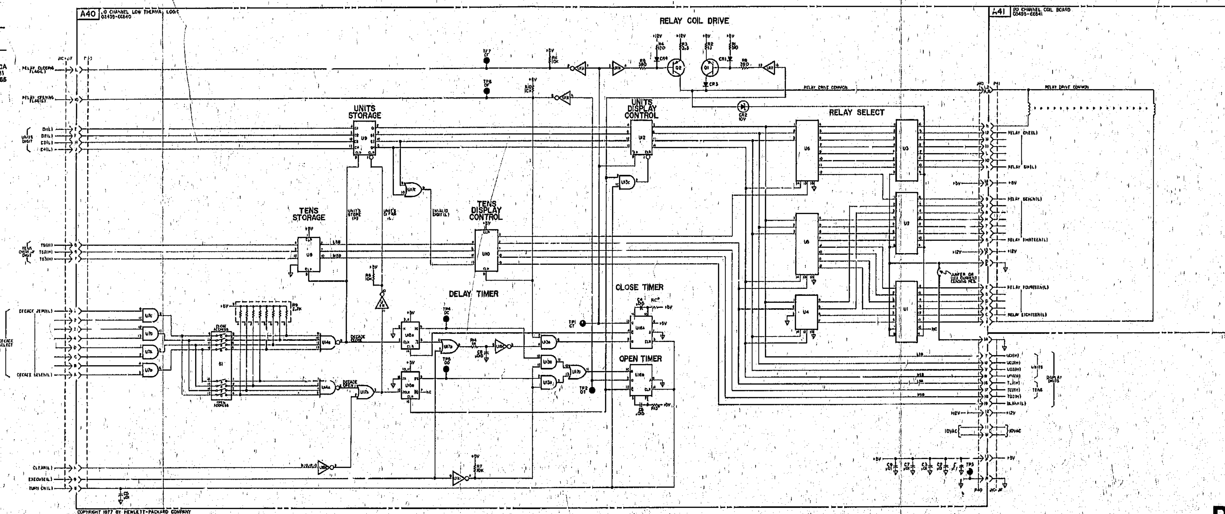
Figure 7-D-8. Duo-Decade Logic A40.
