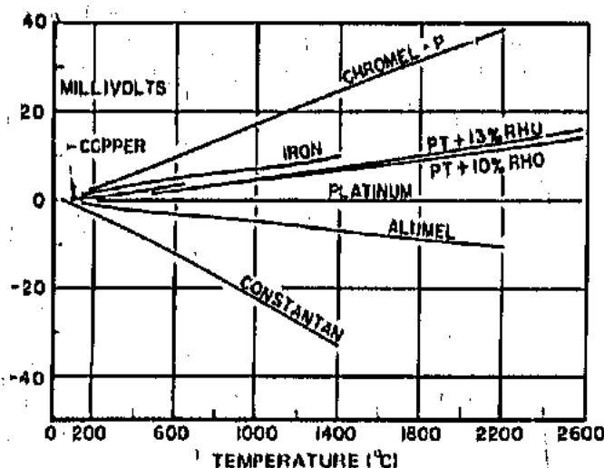
Figure 3-16. V vs. T for Common Thermocouple Materials.
