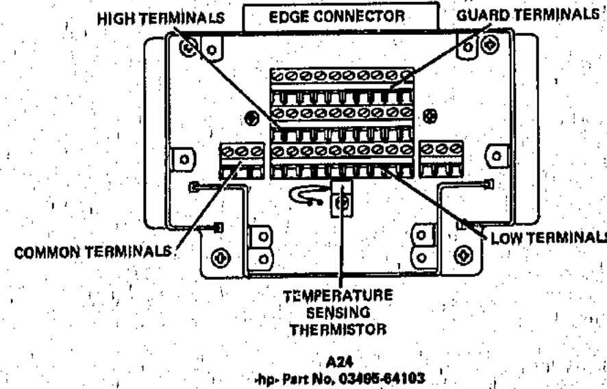
Figure 7-B-21. Low Thermal Channel/Display A5, A11 through A14, A24 7-B-21/7-B-2
