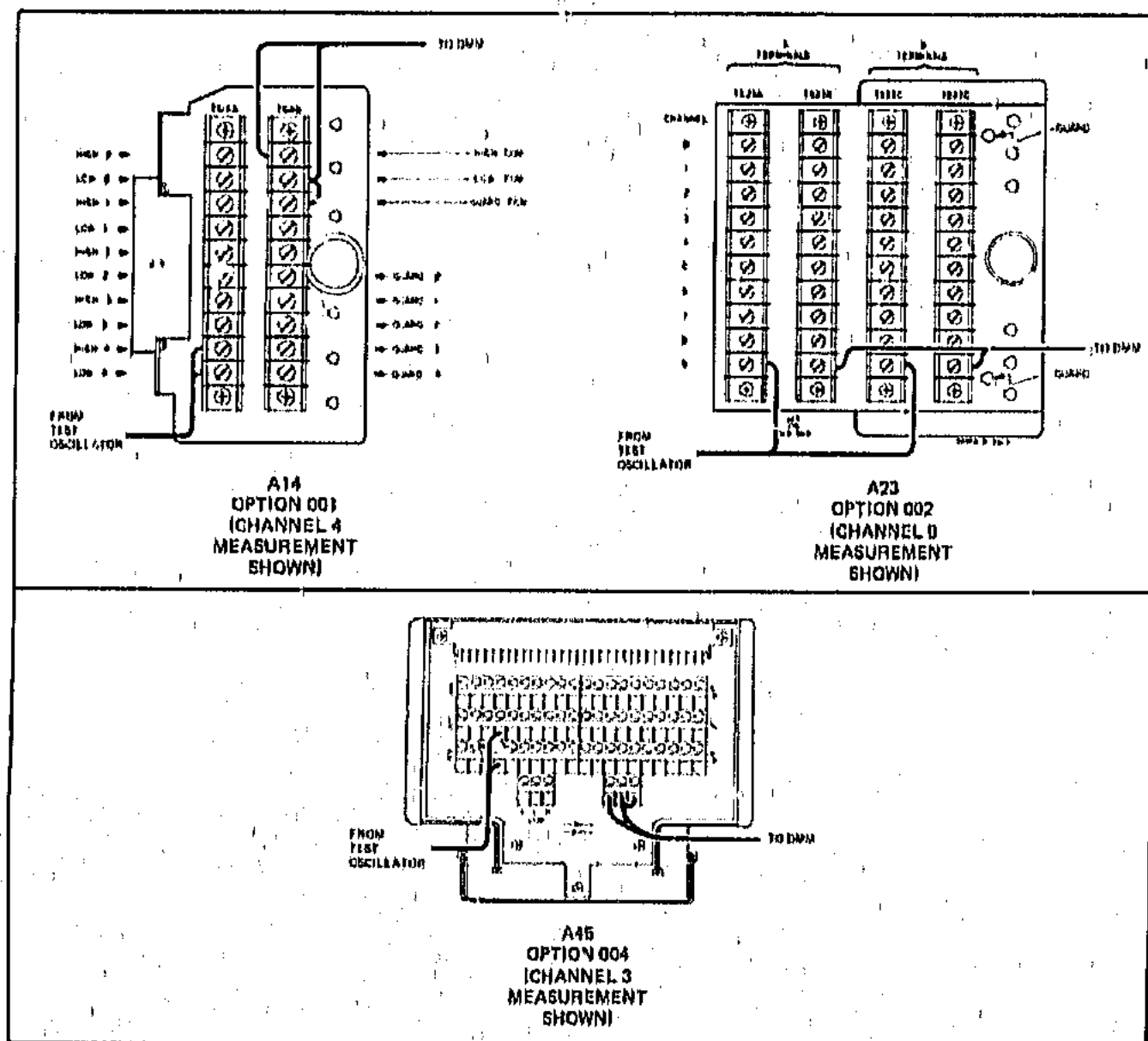
Figure 4-9. Frequency Response Test Wiring Diagrams.
