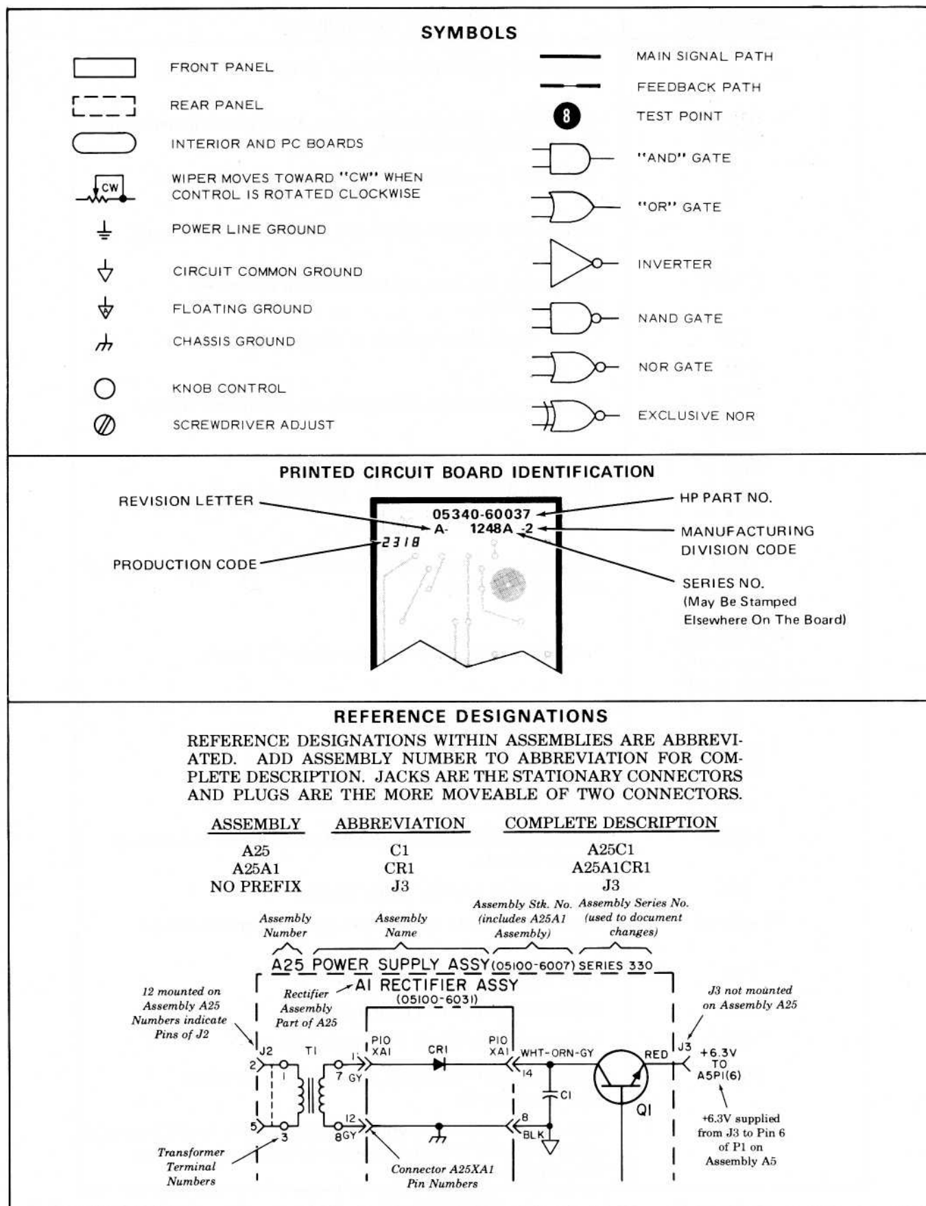
Figure 6-1. Schematic Diagram Notes
