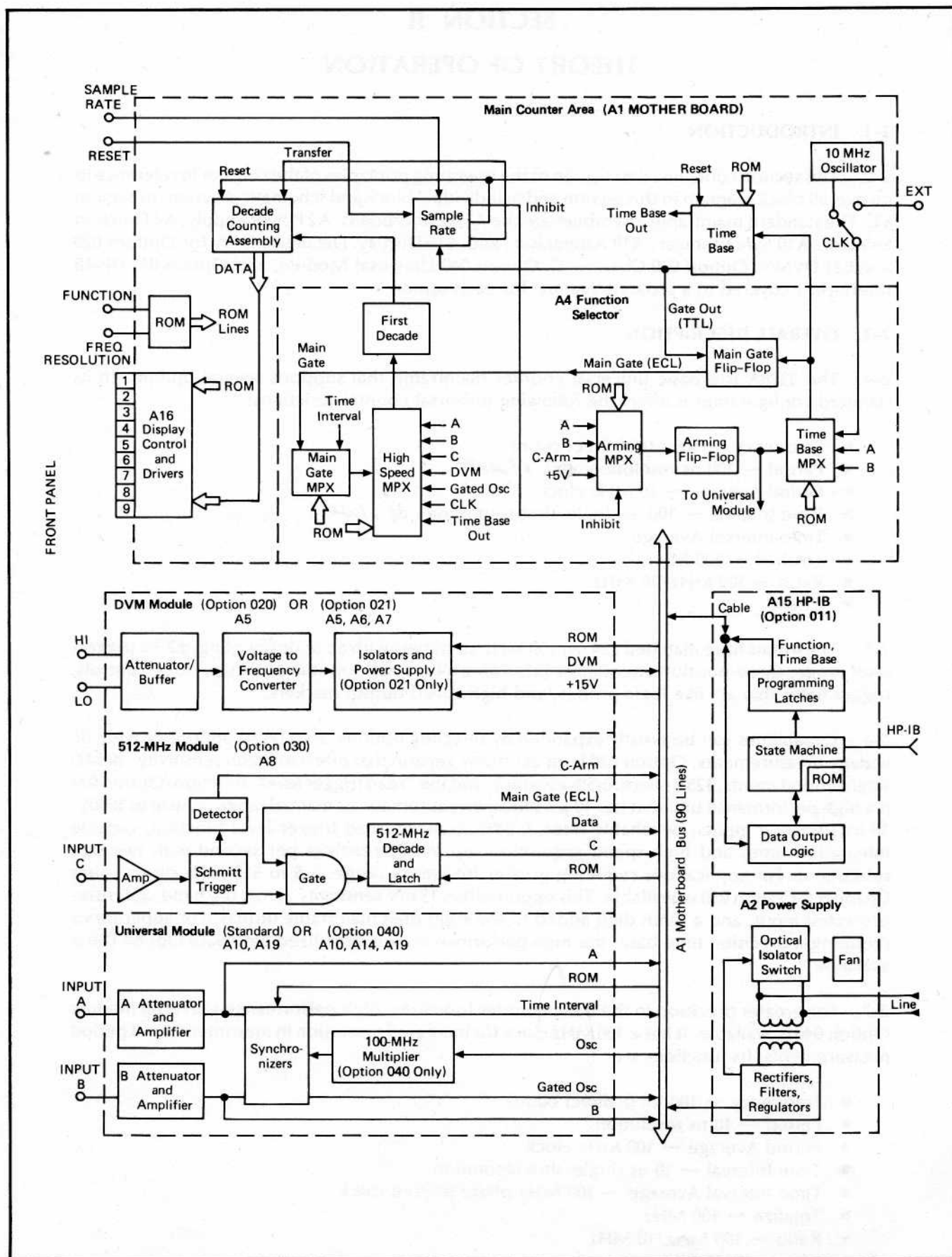
Figure 2-1. Block Diagram
