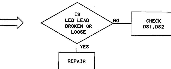
Figure 3-5. Standard A19 /
