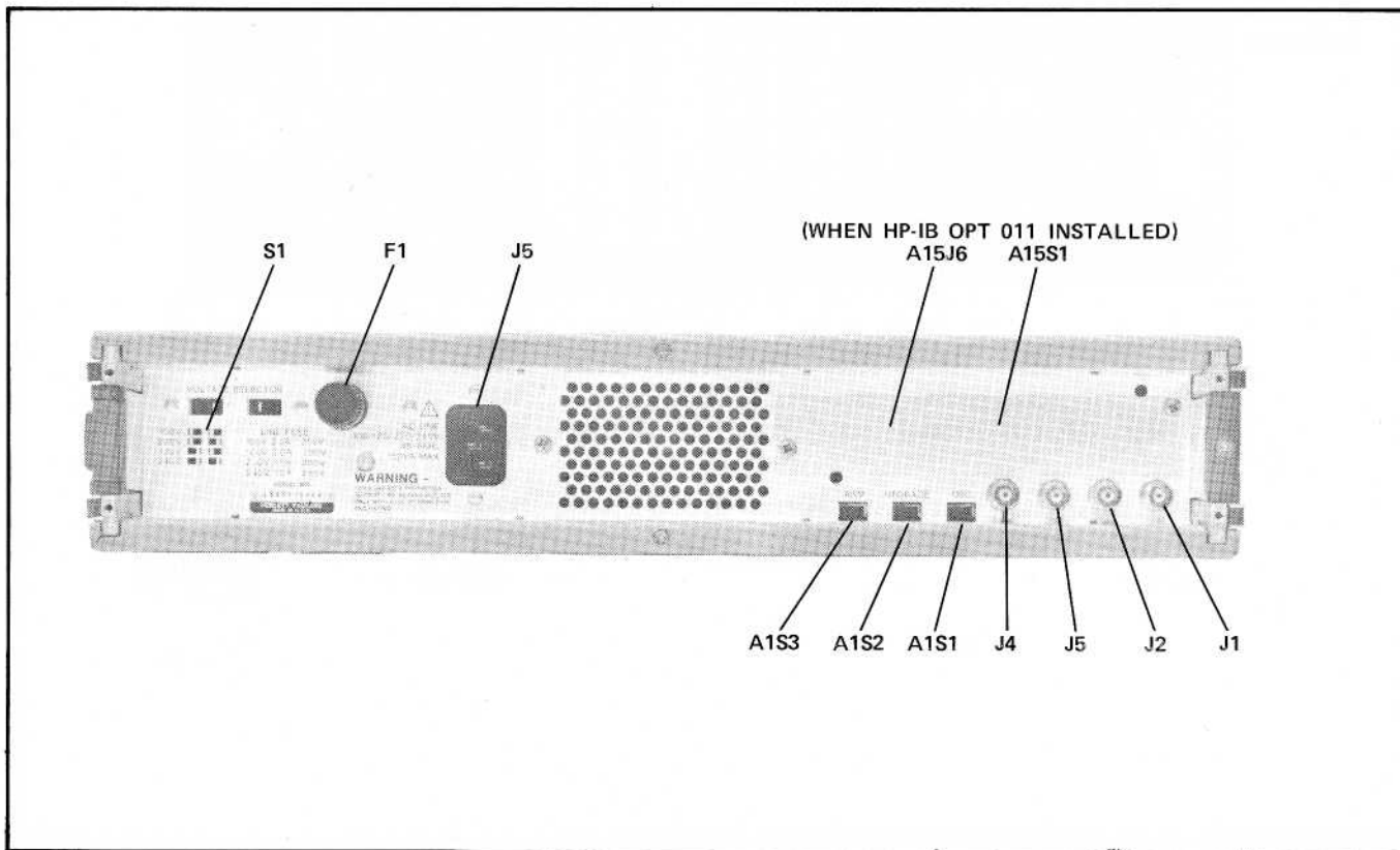
Figure 6-3. 5328A Rear View
