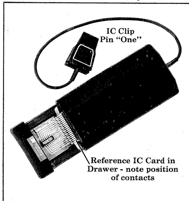
Figure 3-3. Reference IC Card in Comparator Drawer
