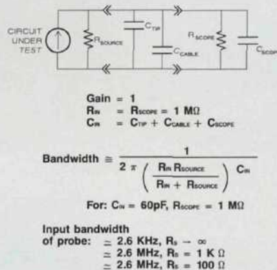
Figure 1. Equivalent circuit of a 1:1 probe
