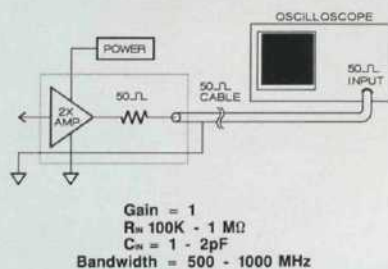
Figure 4. One version of an active probe.
