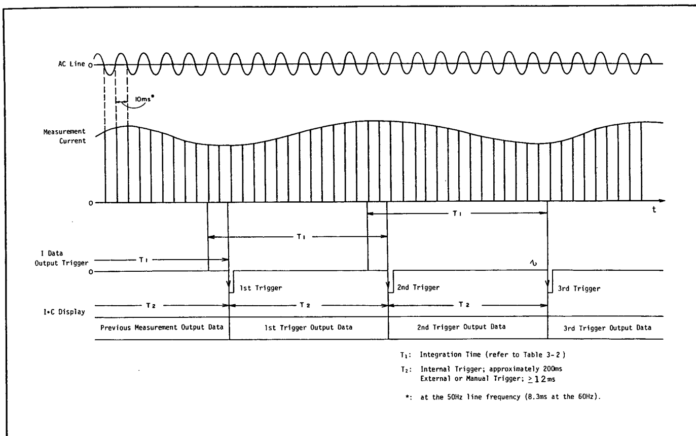
Figure 3-5. Integration Time and Data Output (When FUNCTION is Set to I).
