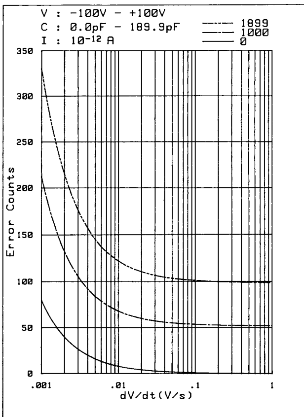
Figure 3-22. C-V Measurement Accuracy (Sheet 3 of 4).
