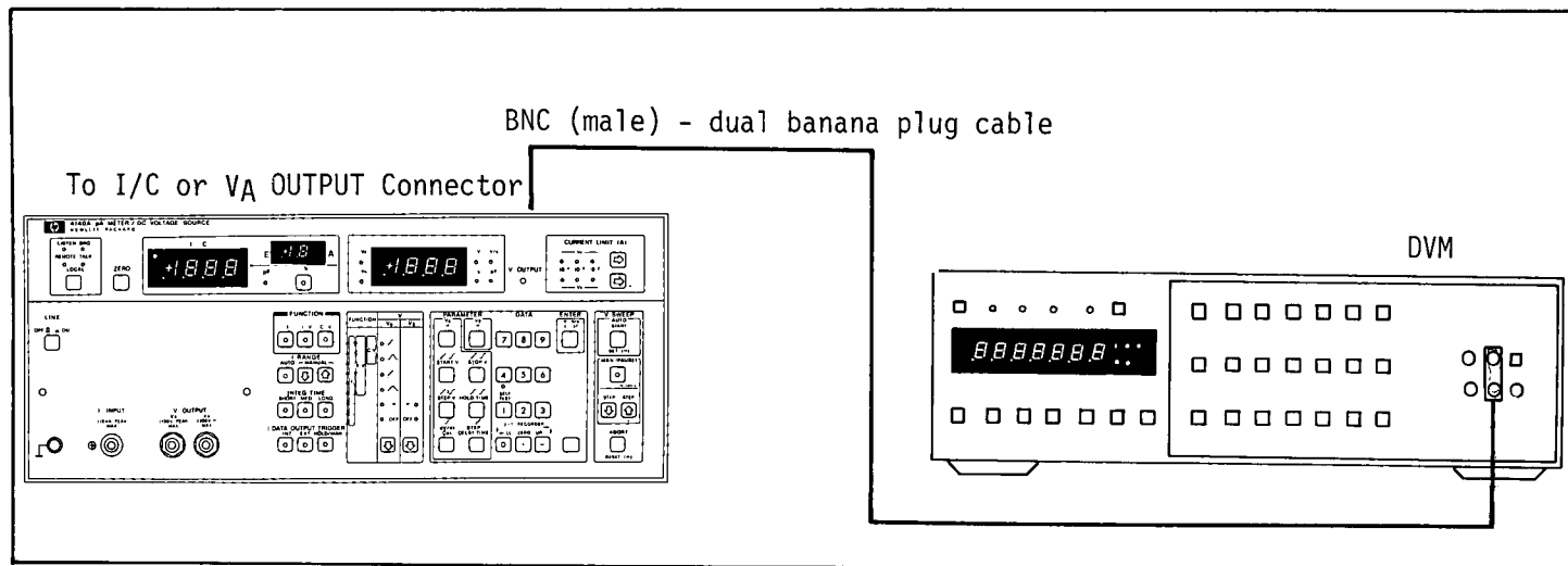
Figure 4-8. Analog Output Accuracy Test Setup.
