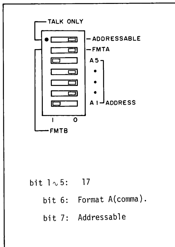
Figure 3-25. HP-IB Control Switch.
