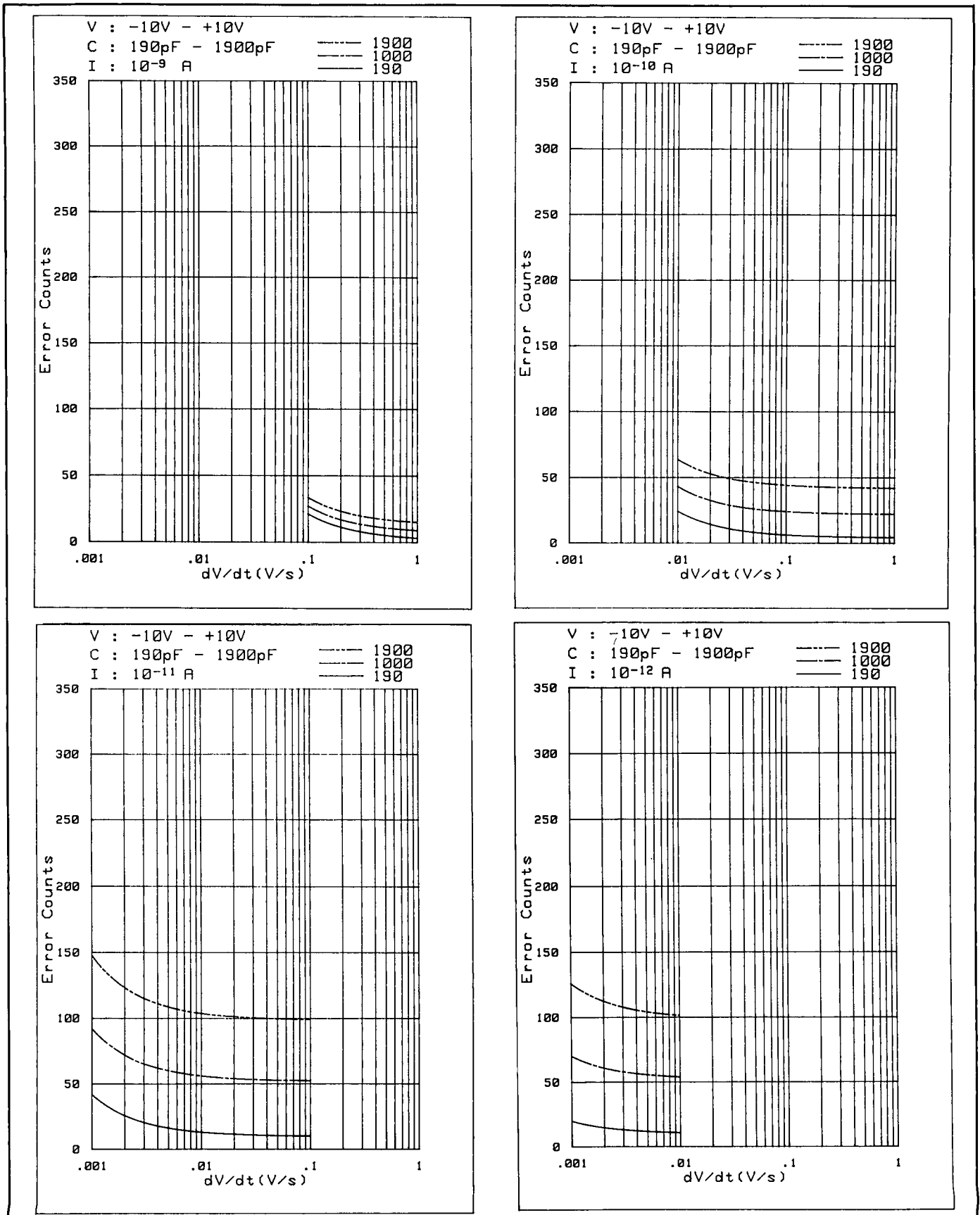
Figure 3-22. C-V Measurement Accuracy (Sheet 2 of 4).
