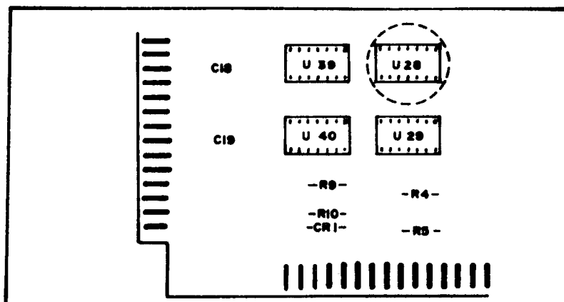
Figure B. Part of A4 Board Component Locations.
