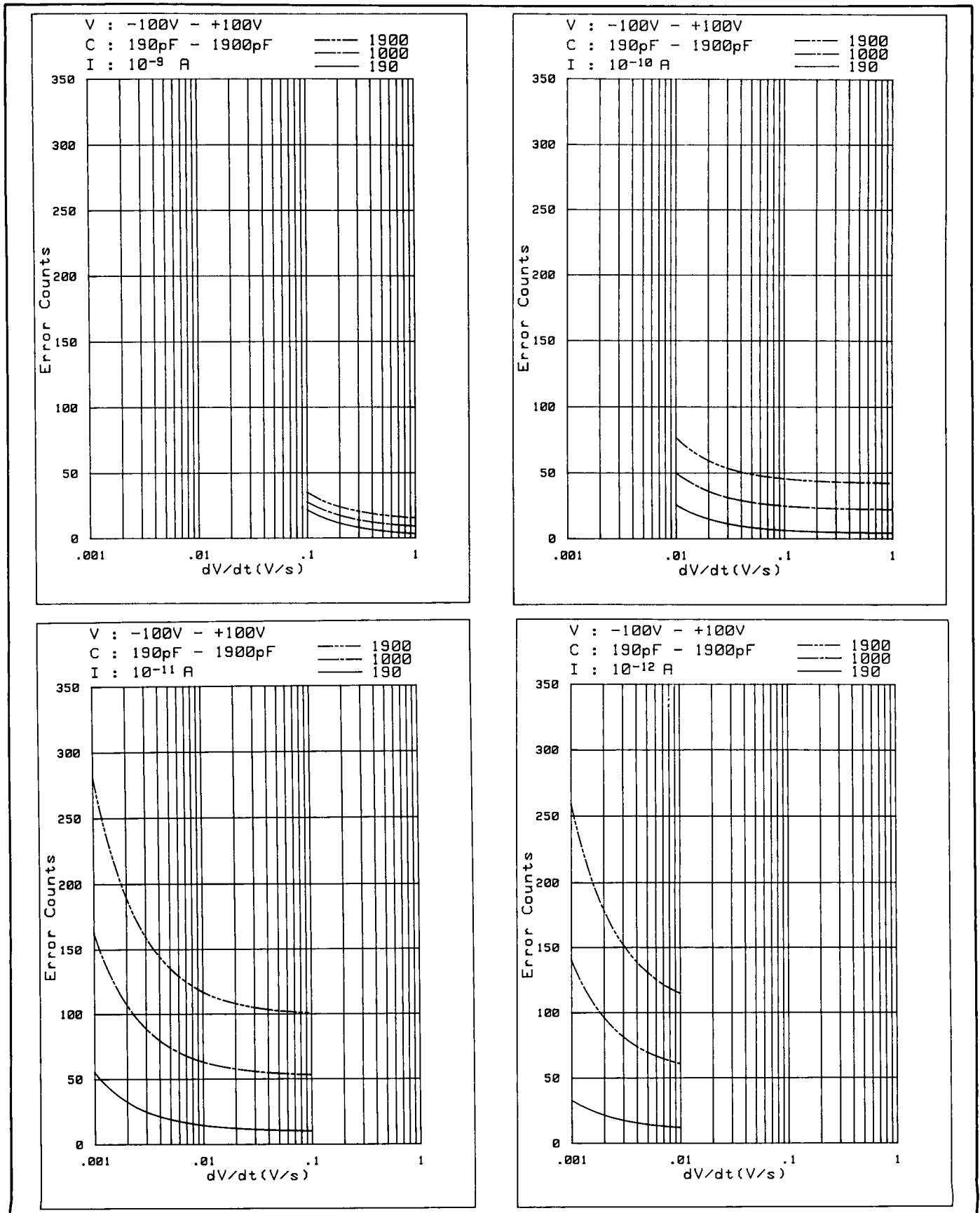
Figure 3-22. C-V Measurement Accuracy (Sheet 4 of 4).
