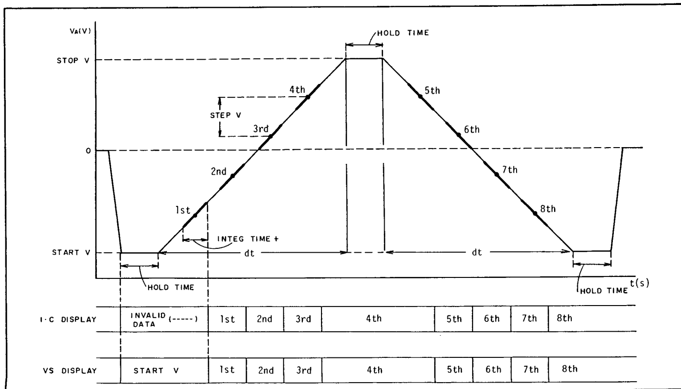
Figure 3-19. Relationship between C-V Measurement and Displays for \nearrow \searrow (Double Ramp Wave).
