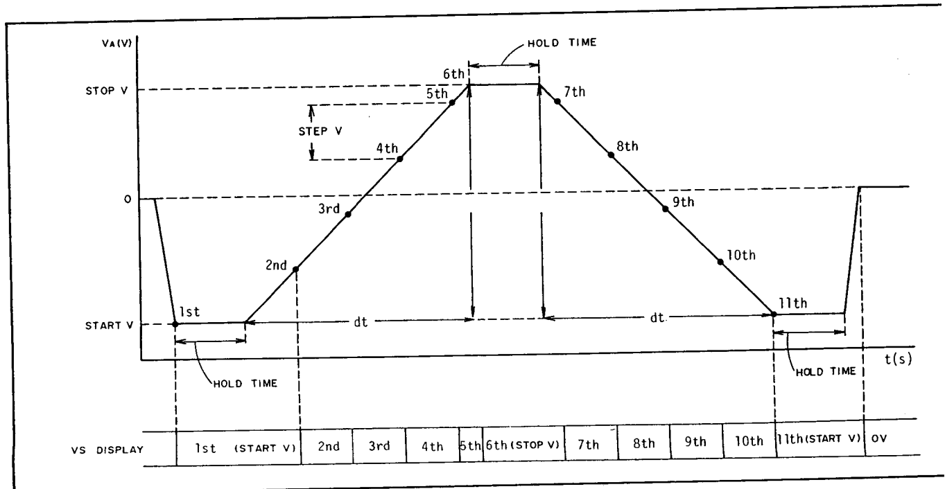
Figure 3-10. Relationship between Output Voltage and Display for \wedge (Double Ramp Wave).
