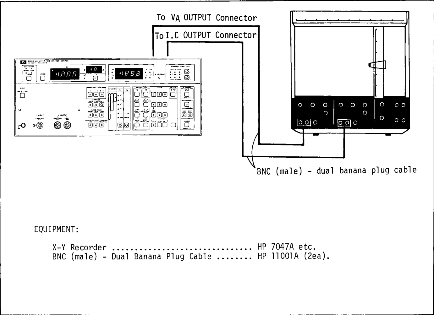
Figure 3-24. Option 001 Analog Output Operating Instructions (sheet 1 of 2).
