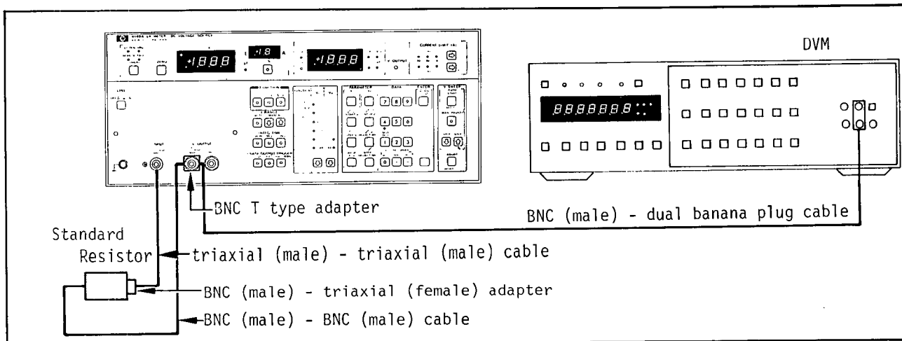
Figure 4-3. Current Accuracy Test Setup ( 10^{-8}\text{A} \sim 10^{-12}\text{A} Ranges).
