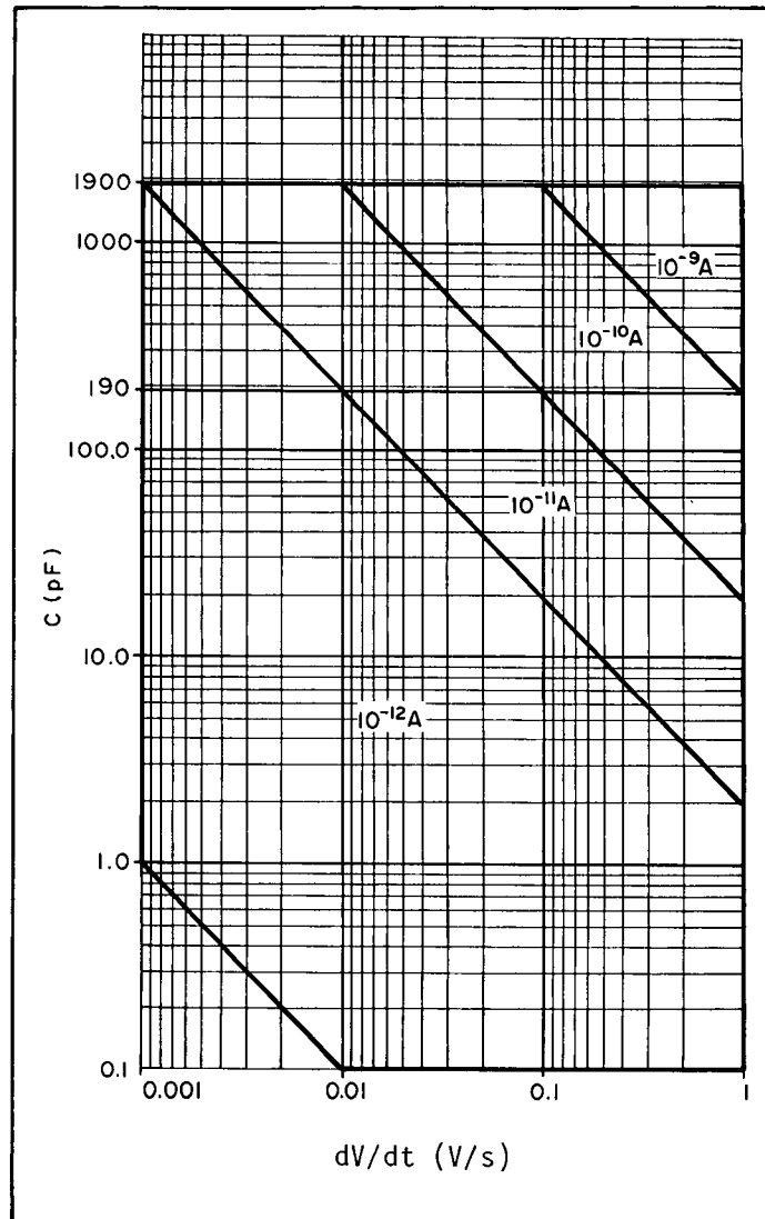
Figure 3-21. Suitable Current Ranges for C-V Measurements,
