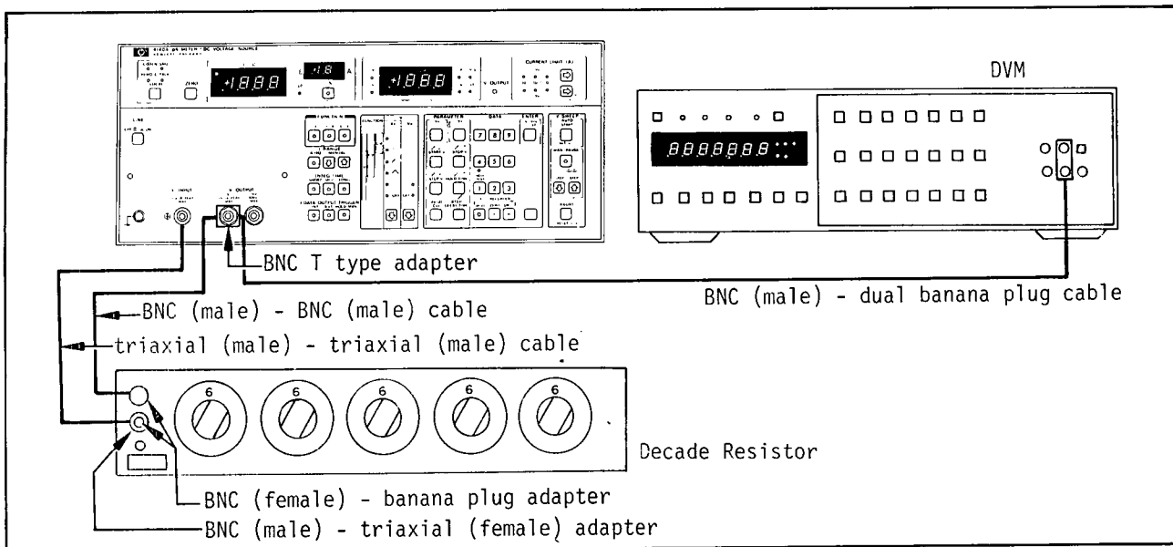
Figure 4-2. Current Measurement Accuracy Test Setup ( 10^{-2}\text{A} \sim 10^{-7}\text{A} Ranges).
