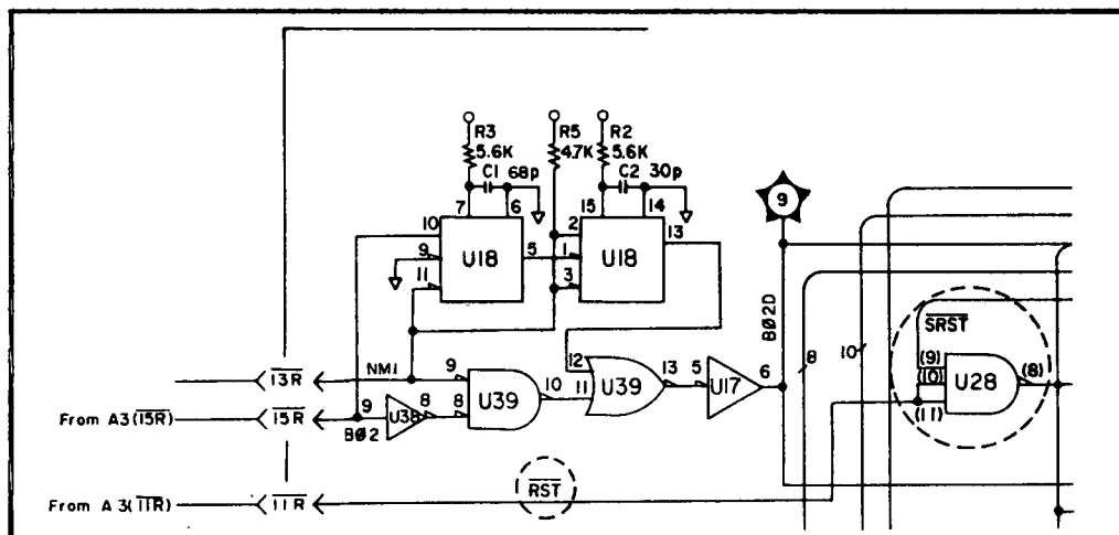
Figure A. Part of A4 Board Schematic Diagram.
