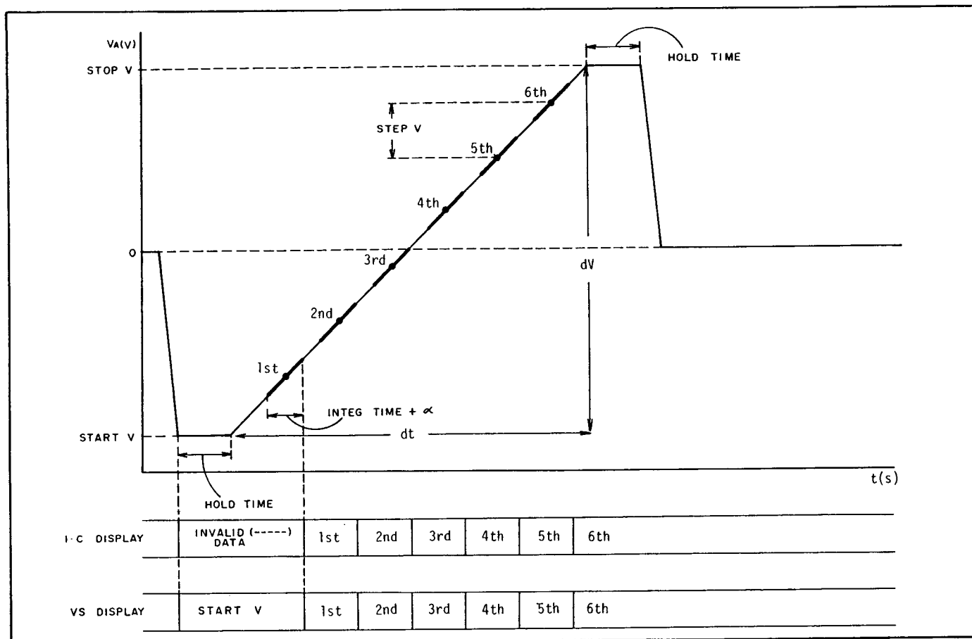
Figure 3-18. Relationship between C-V Measurement and Displays for \nearrow (Single Ramp Wave).
