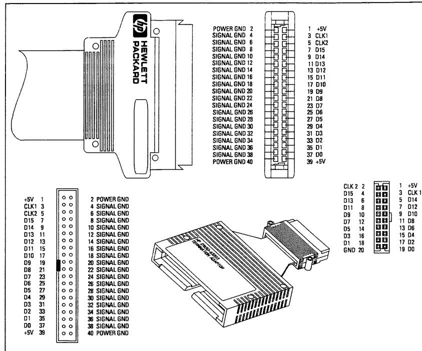
Figure 5A. Pinout for probe cable and 100-k \Omega termination adapter (HP part number 01650-63203)
