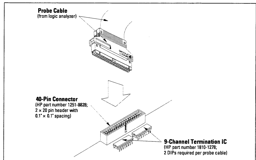
Figure 6B. Connecting probe cable to 40-pin connector with termination DIPs
