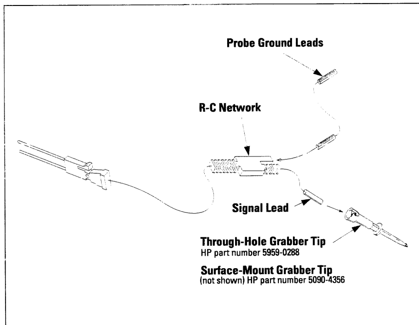
Figure 3. Connecting grabbers and ground leads to probes
