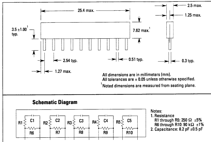
Figure 7A. 5-channel termination IC (HP part number 1810-1588)
