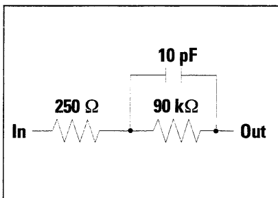
Figure 11. Hybrid network schematic diagram
