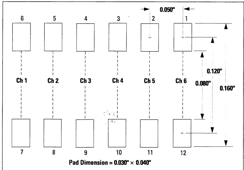
Figure 12. Recommended PC board pattern for surface mount termination RC network
