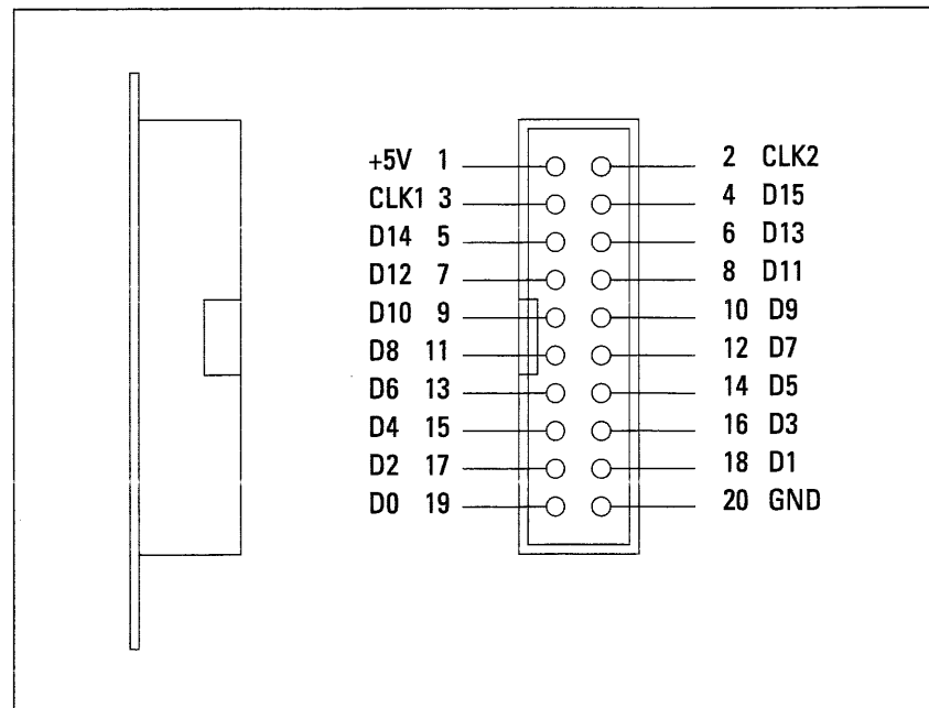
Figure 5B. Pinout for 20 pin connector (HP part number 1251-8106)
