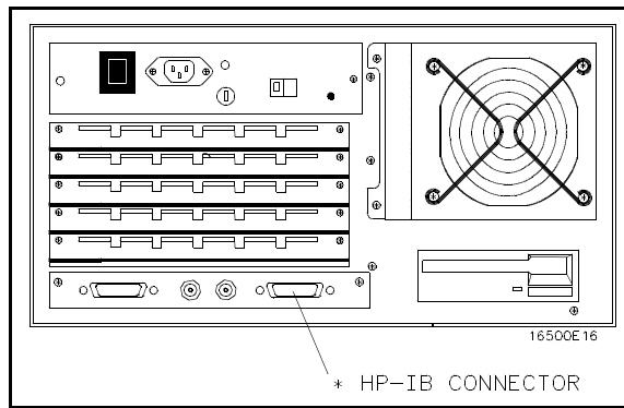
Figure 7-1. HP 16500A/16501A Rear Panel.
