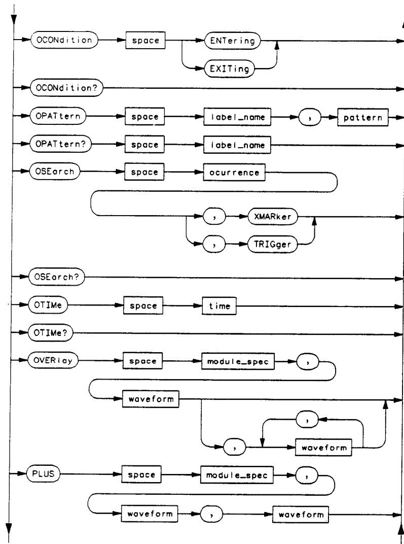
Figure 4-1. Waveform Subsystem Commands Syntax Diagram (Continued)
