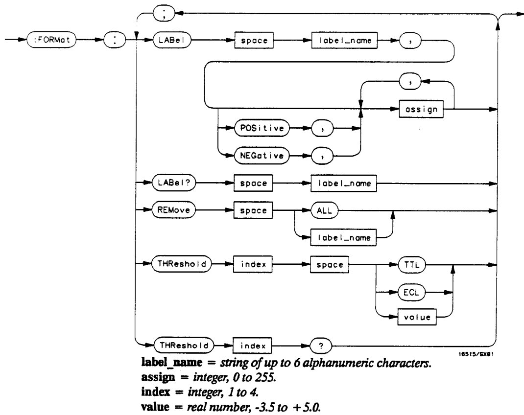
Figure 2-1. Format Subsystem Commands Syntax Diagram
