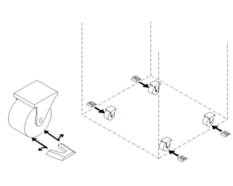
Installing the Wheel Chocks
