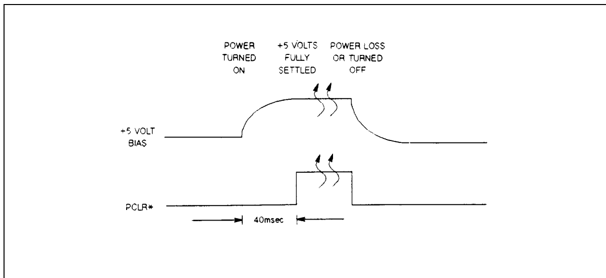
Figure 4-8. +5 V BIAS and PCLR* Timing Sequence
