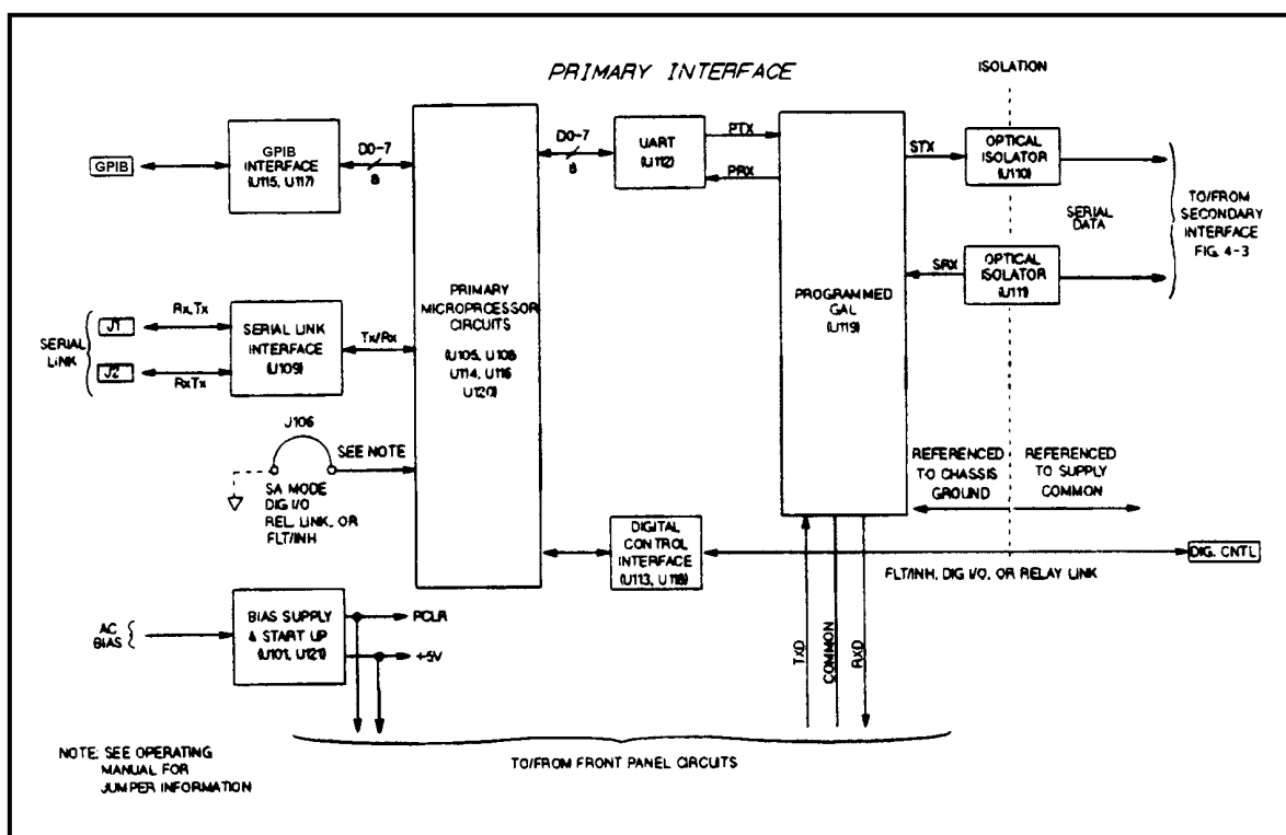
Figure 4-6. GPIB Board, Simplified Block Diagram (Models Keysight 664xA and 665xA Only)
