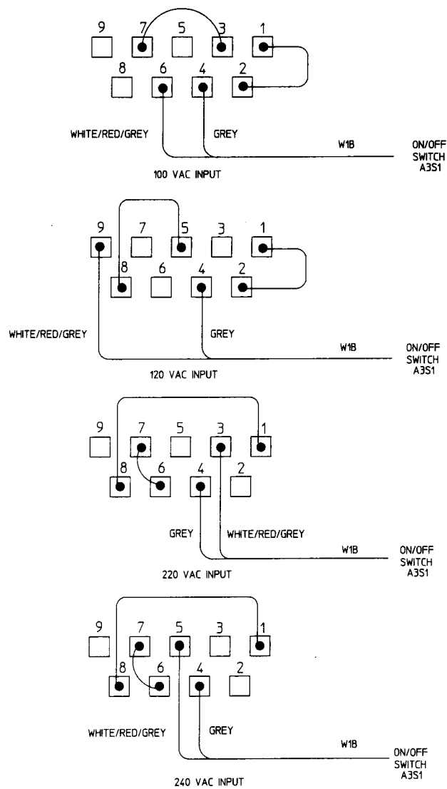
TRANSFORMER T1 PRIMARY-AC INPUT CONNECTIONS (ALL MODELS)
