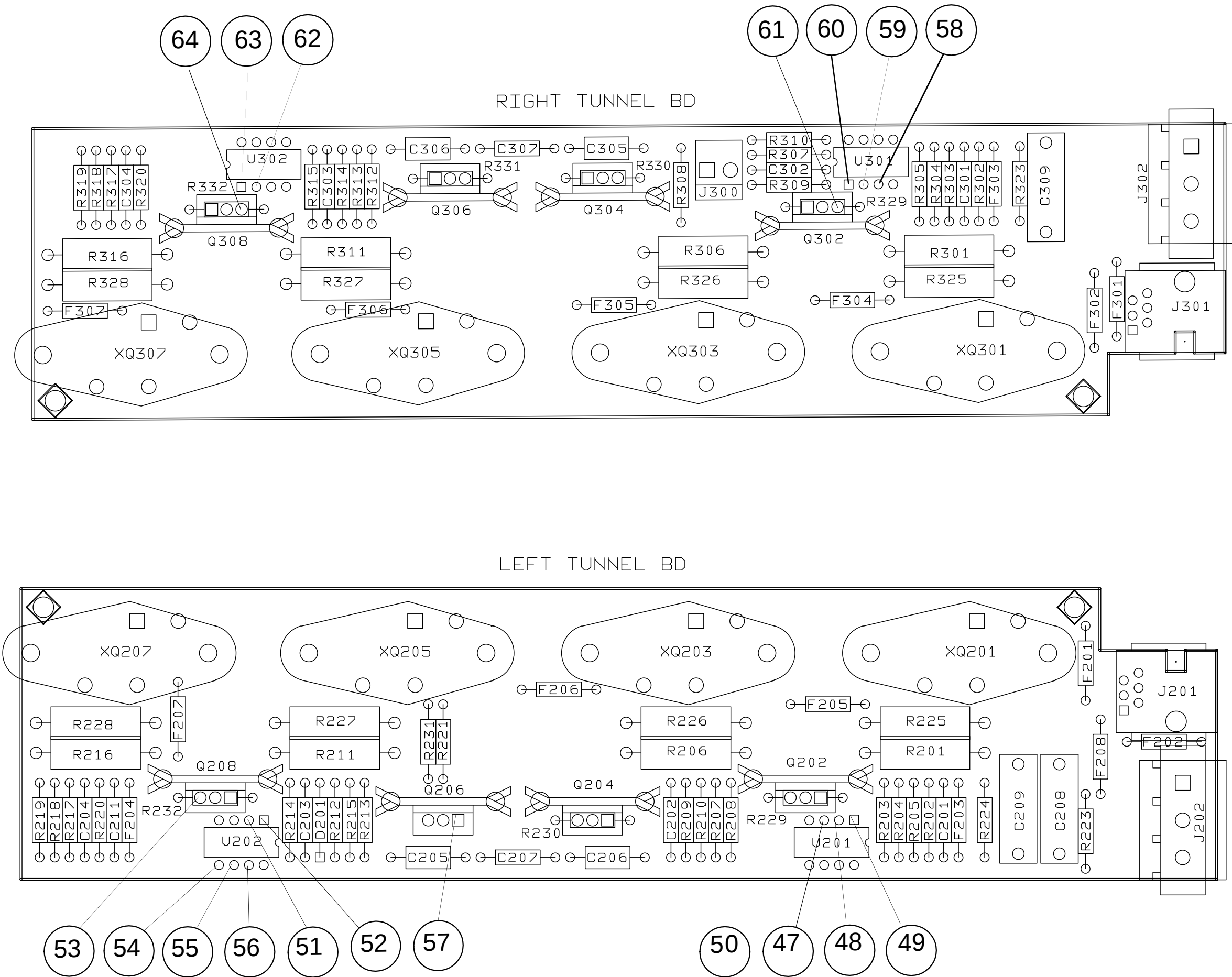
Artisan Technology Group - Quality Instrumentation ... Guaranteed | (888) 88-SOURCE | www.artisantech.com Figure 6-6 Left/Right Tunnel Board Assembly Diagram and Test Points for 655xA & 665xA Models Only
