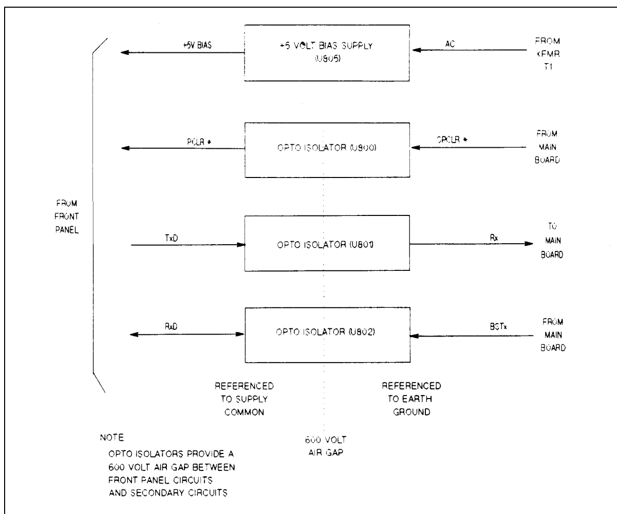
Figure 4-7. Isolator Board, Simplified Block Diagram (Models Keysight 654xA and 655xA)
