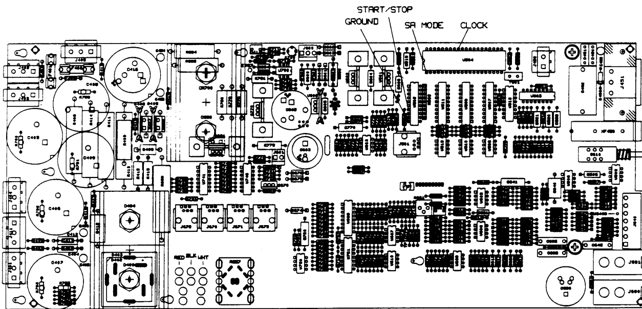
c. A1 MAIN BOARD
