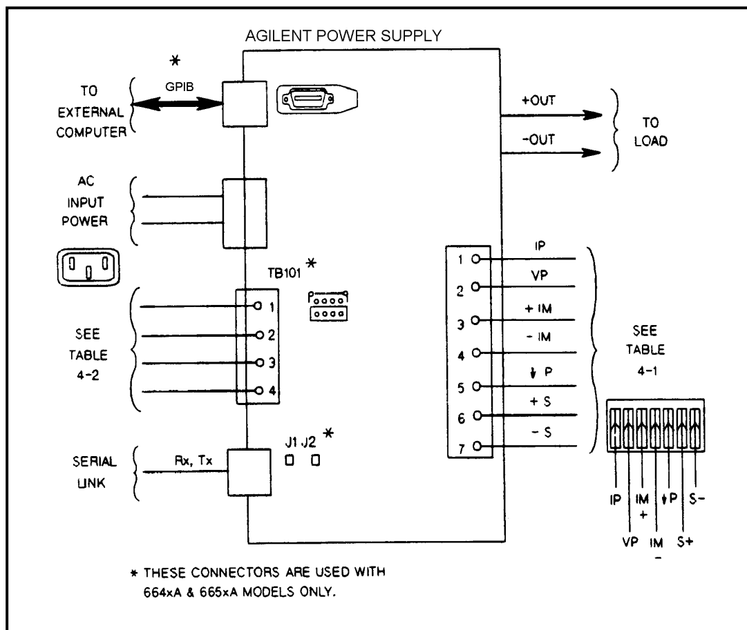
Figure 4-1. Keysight Power Supply, I/O Interface Diagram
