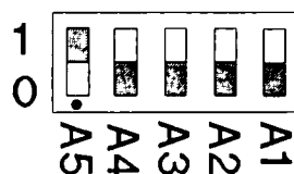
Figure 4-15. HP-IB Address Switch (Factory setting)
