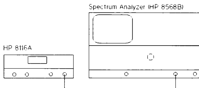
Figure 8-6. Sine Waveform Performance Test
