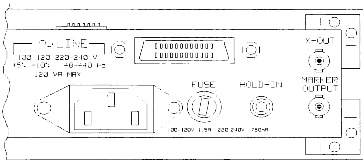
Figure 4-14. Rear panel
