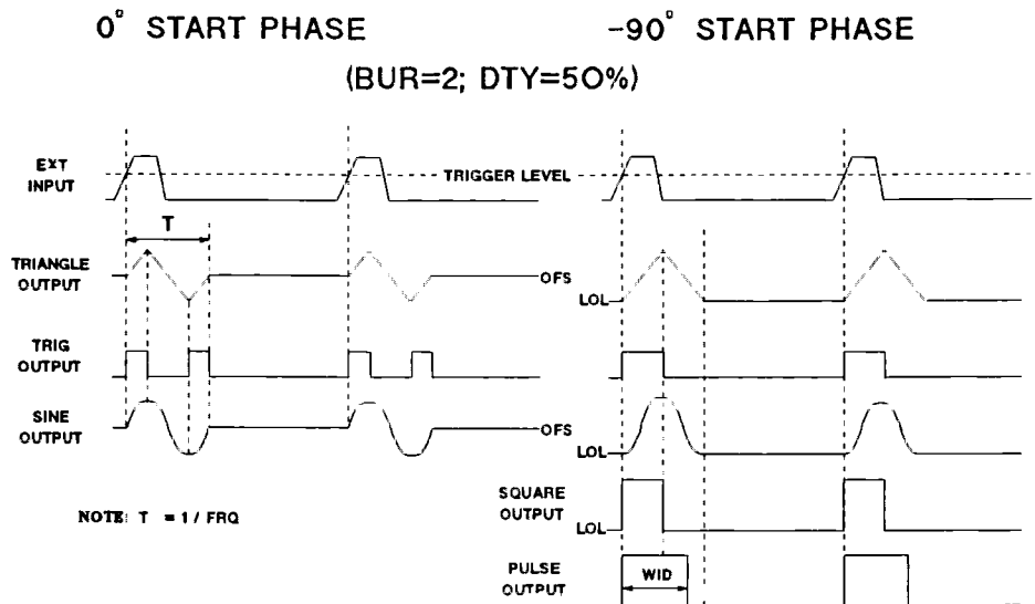
Figure 5-2. Typical signals in Trigger mode
