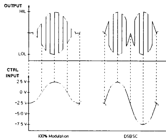
Figure 4-6. Amplitude Modulation
