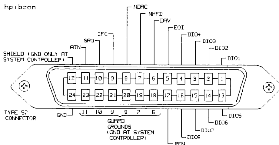
Figure 3-3. HB-IB Connector
