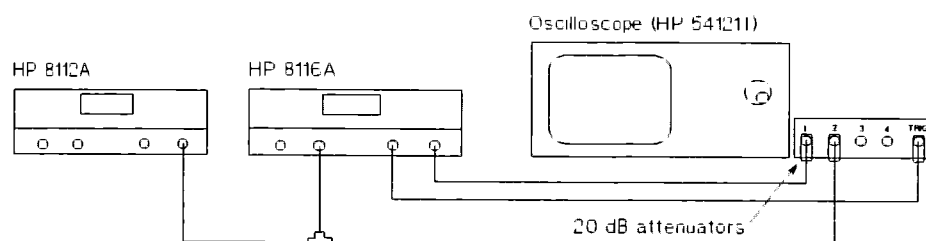
Figure 8-15. Pulse Width Modulation Verification Test
