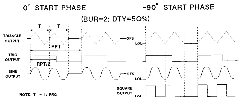
Figure 5-6. Typical outputs in Internal Burst mode
