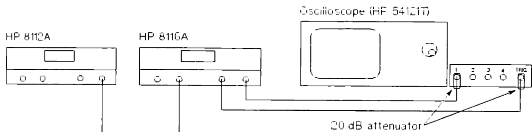
Figure 8-13. Frequency Modulation Verification Test
