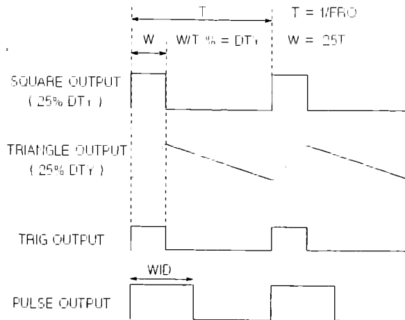
Figure 4-11. Timing parameters
