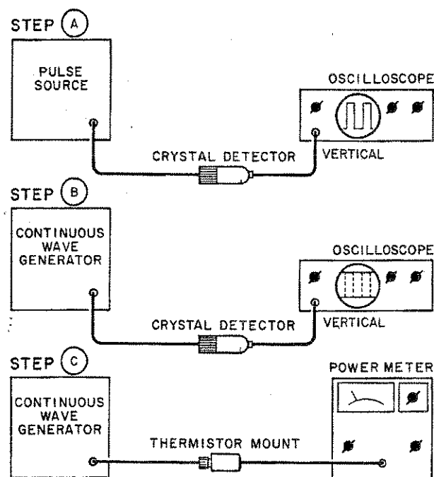
Figure 1. Peak Power Measurement
