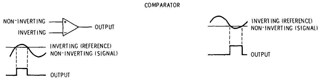
Figure 8-15. Comparator
