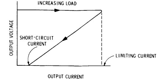
Figure 8-65. Current Foldback
