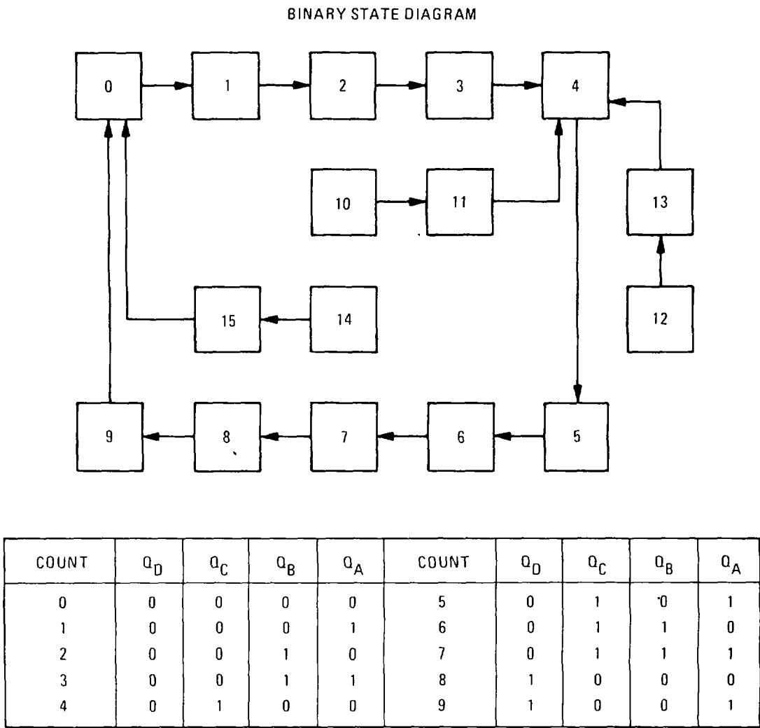
Figure 8-12. Programmable Counter
