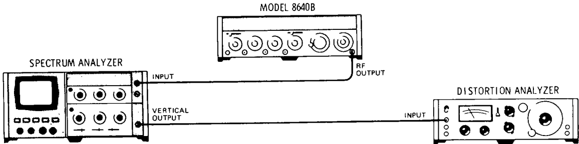
Figure 4-19. AM Distortion Test Setup.
