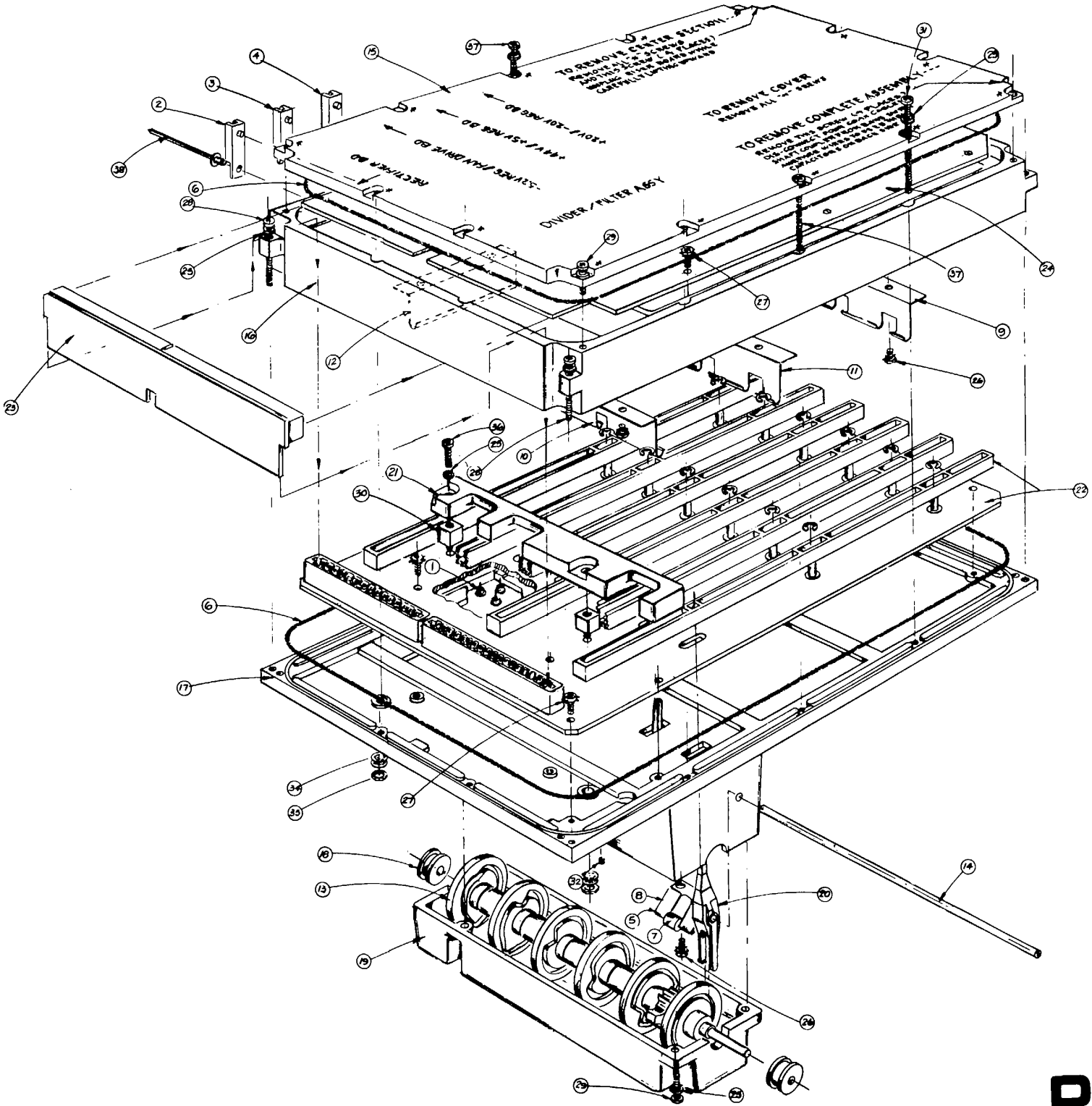
Figure 8-80. A10 Divider/Filter Assembly Illustrated Parts Breakdown
