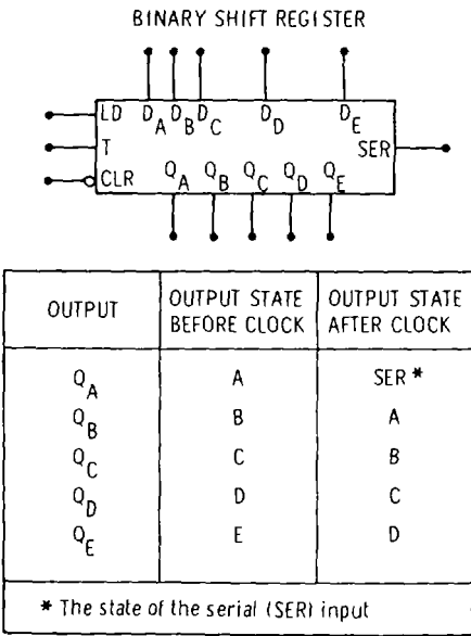
Figure 8-10. Binary Shift Register
