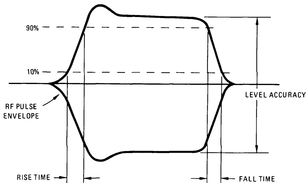
Figure 4-23. Pulse Measurements
