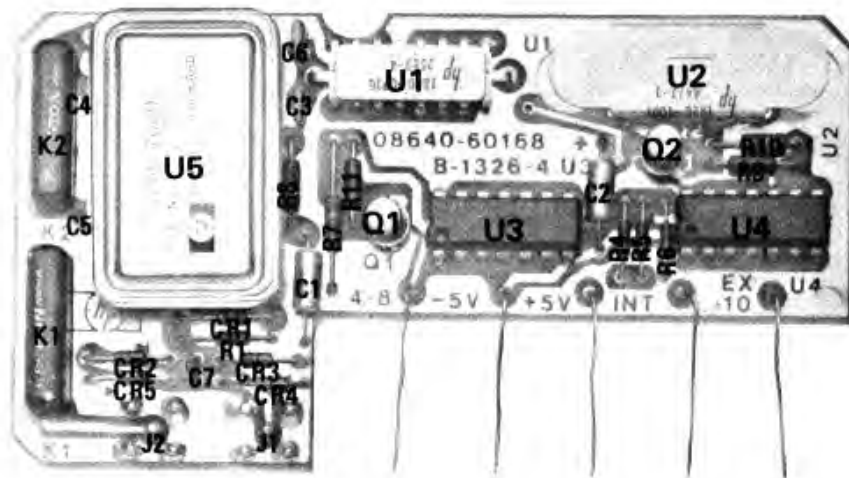
Figure 8-55. A8A1 RF Scaler Assembly Component Locations (P/O Change 10)
