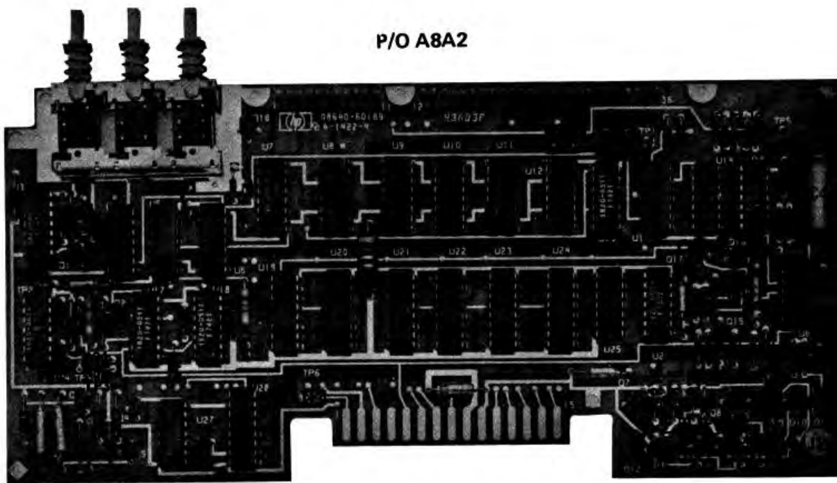
Figure 8-63. P/O A8A2 Counter/Lock Board Assembly Component Locations (P/O Change 19)
