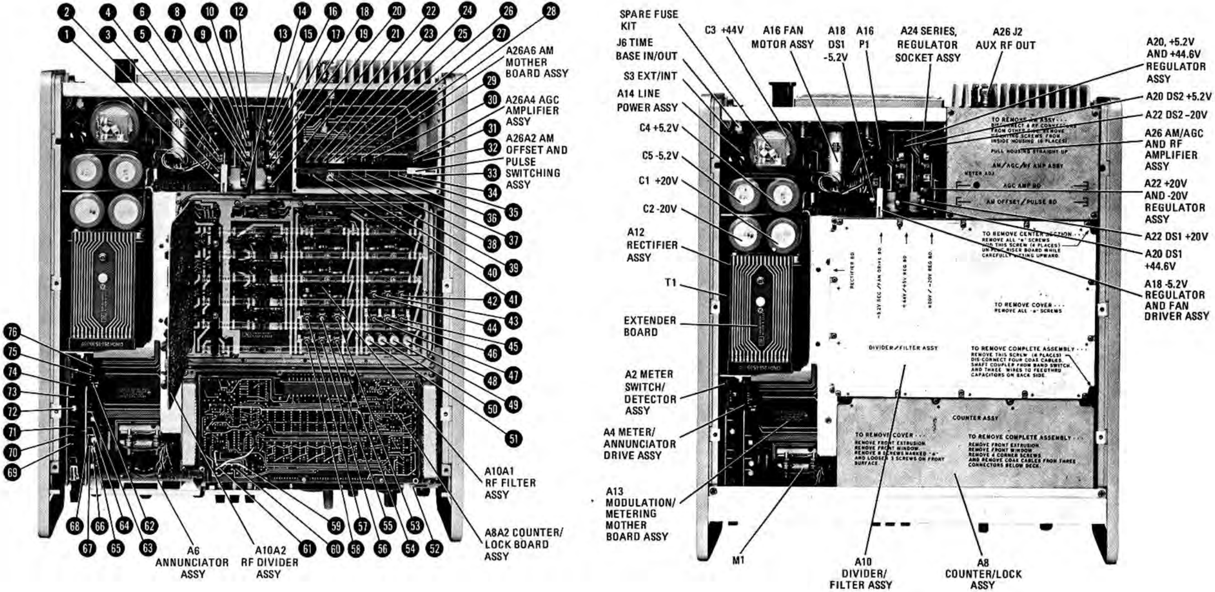
Figure 8-82. Top Internal Views (Options 001 Shown)
