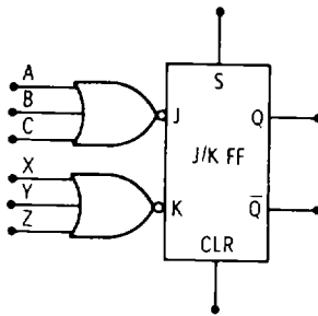
MULTIPLE INPUT J/K FLIP-FLOP
