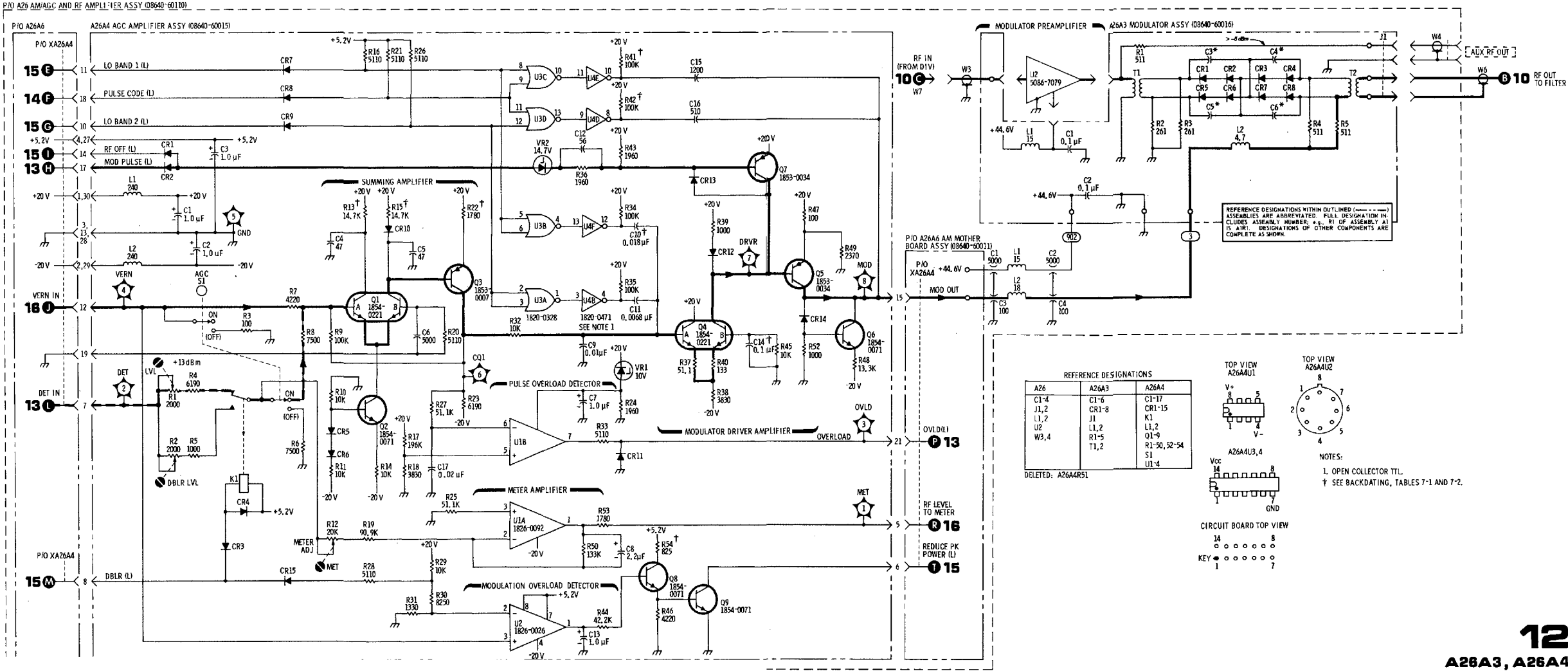
Figure 8-42. AGC Amplifiers and Amplitude Modulator Schematic Diagram.
