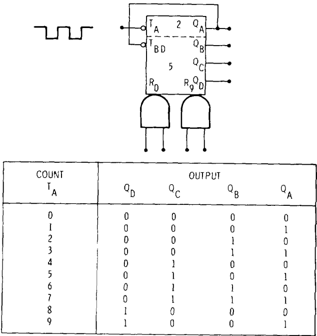
Figure 8-11. Basic Decade Counter (Scaler)
