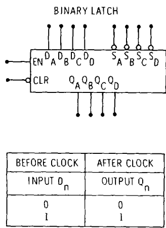
Figure 8-9. Binary Latch
