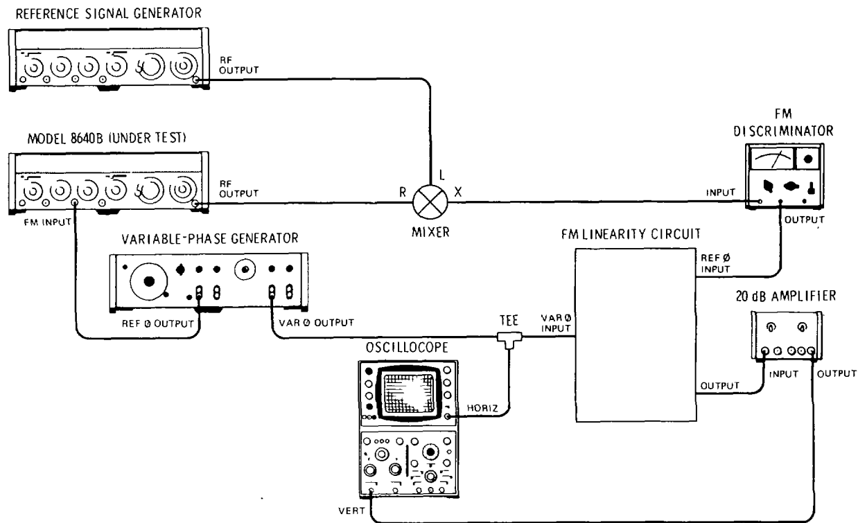
Figure 5-7. FM Linearity Adjustment Test Setup
