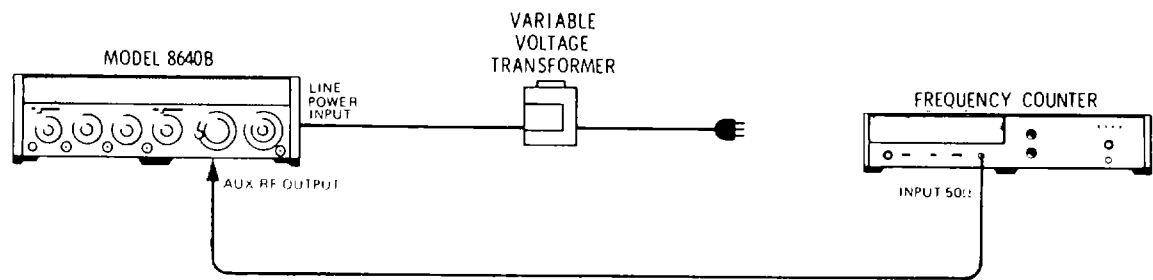
Figure 4-3. Frequency Stability us Line Voltage Test Setup
