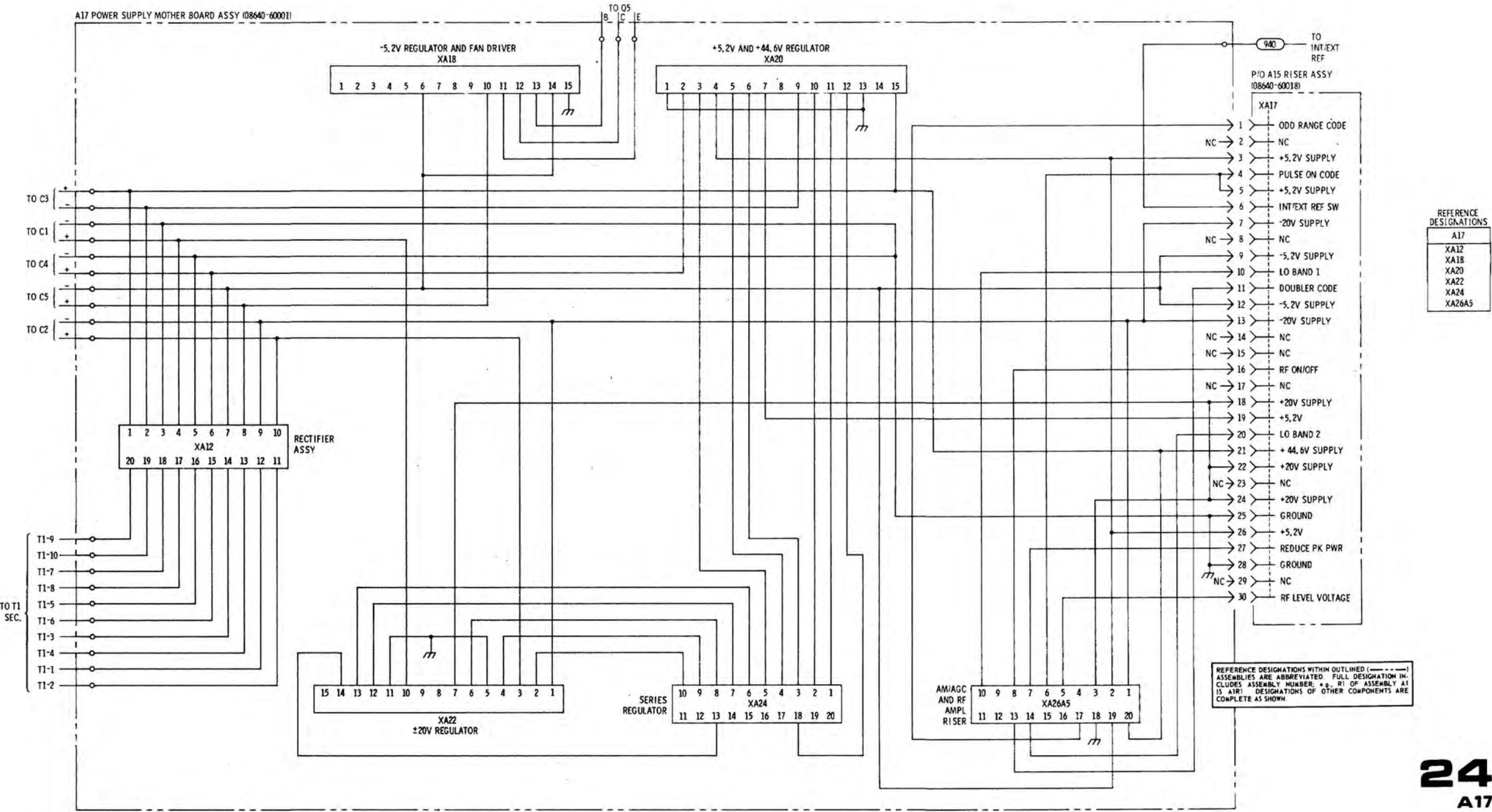
Figure 8-73. Power Supply Mother Board Schematic Diagram
