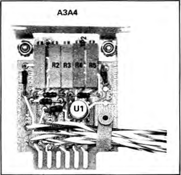
Figure 8-22. P/O A3A4 Connector Board Assembly Component Locations
