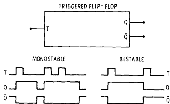
Figure 8-4. Triggered Flip-Flop
