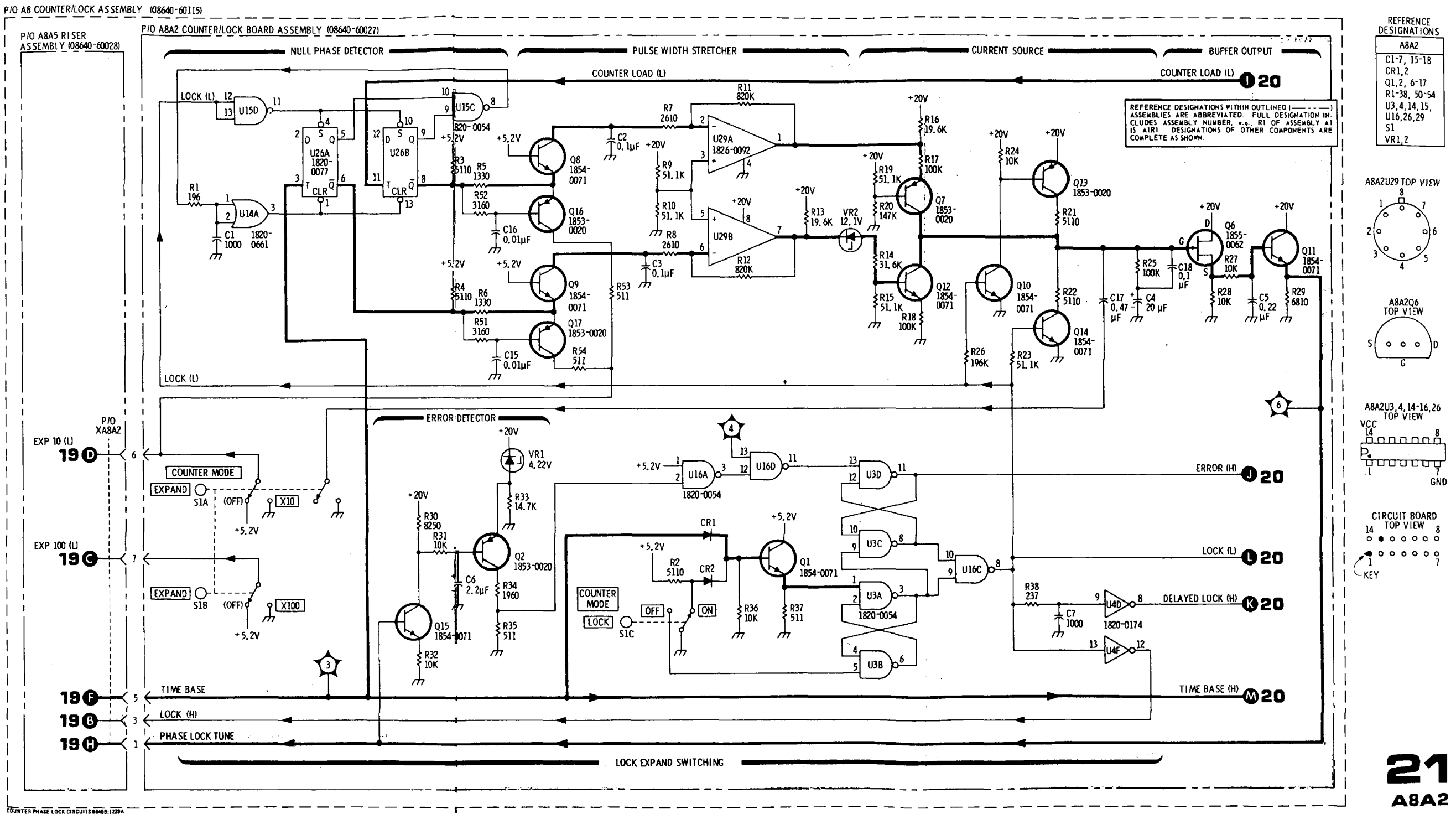
Figure 8-64. Counter Phase Lock Circuits Schematic Diagram
