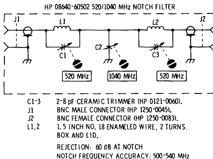
Figure 1-7. 520/1040 MHz Notch Filter.
