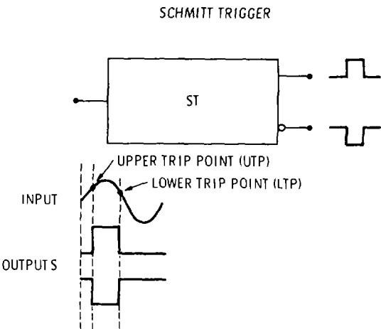
Figure 8-6. Schmitt Trigger
