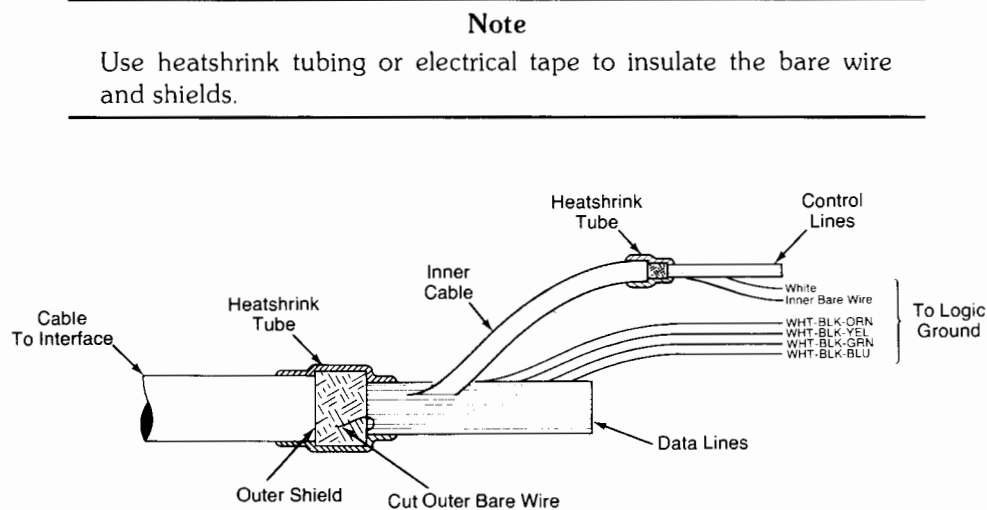
Figure 2-9. Preparing the Interface Cable
