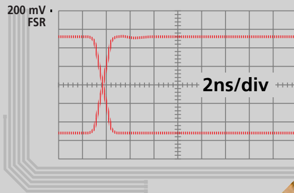
Positive and negative step responses show little or no overshoot or undershoot
