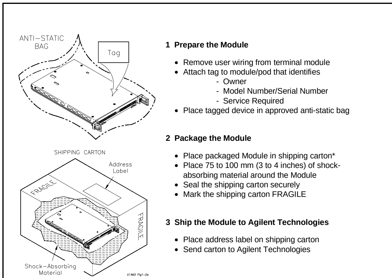
Figure 1-3. Packaging/Shipping Guidelines
