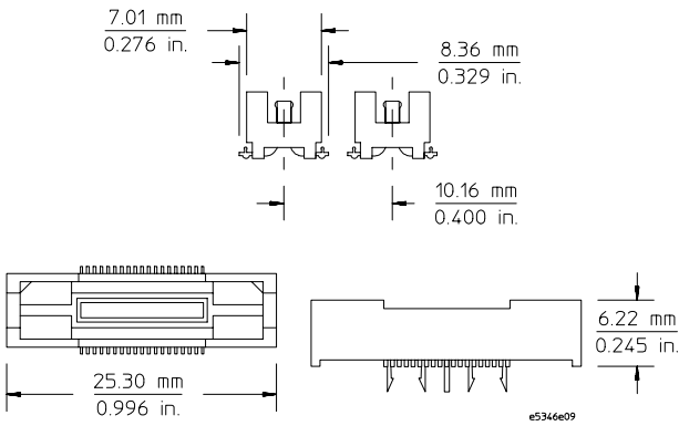
38-pin MICTOR connector dimensions
