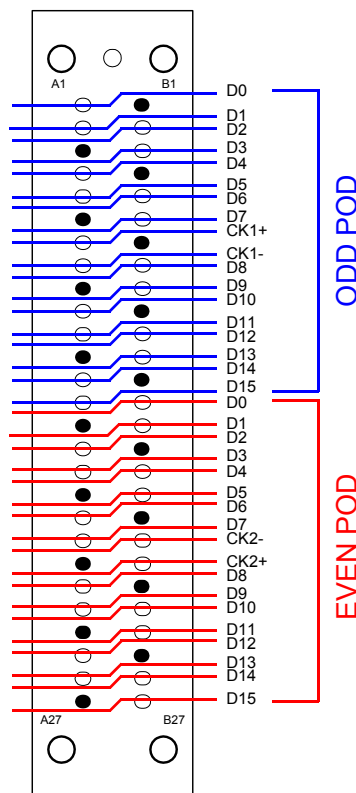
Figure 45 34-bit single-ended routing (E5402A, E5404A, and E5406A)
