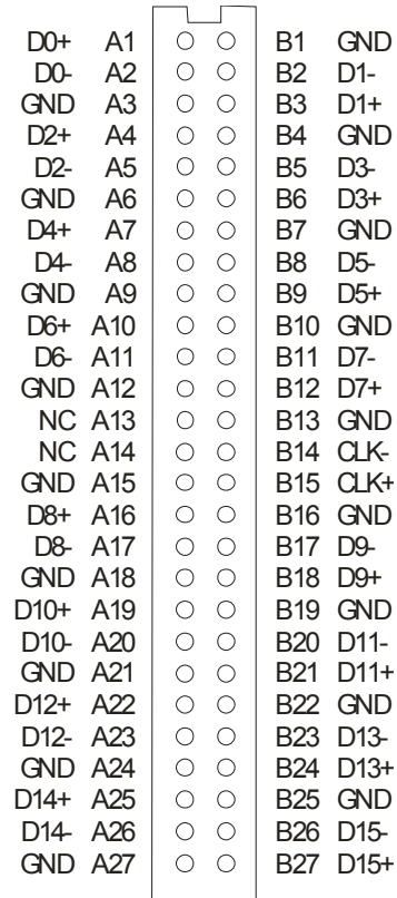
Figure 16 Pad numbers for E5405A-pro series.
