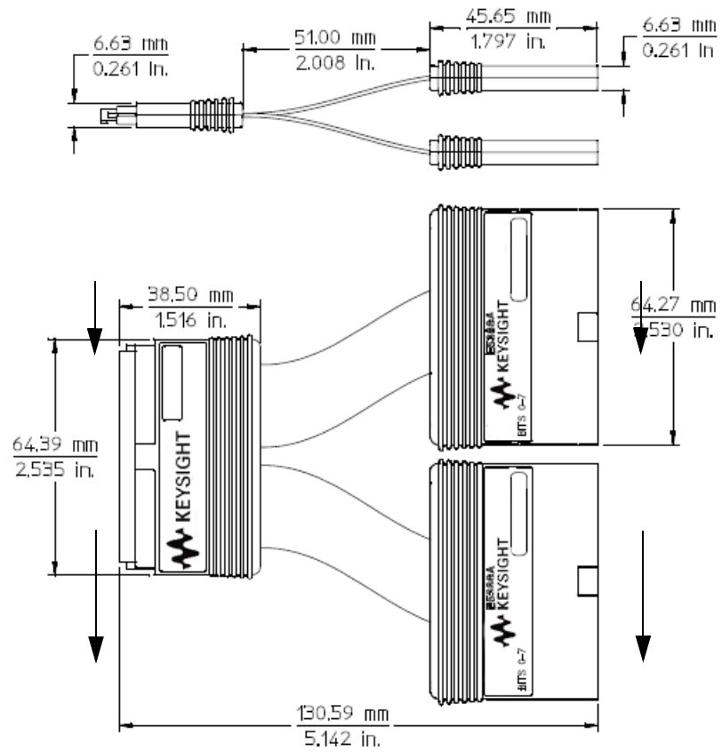
Figure 18 E5386A dimensions
