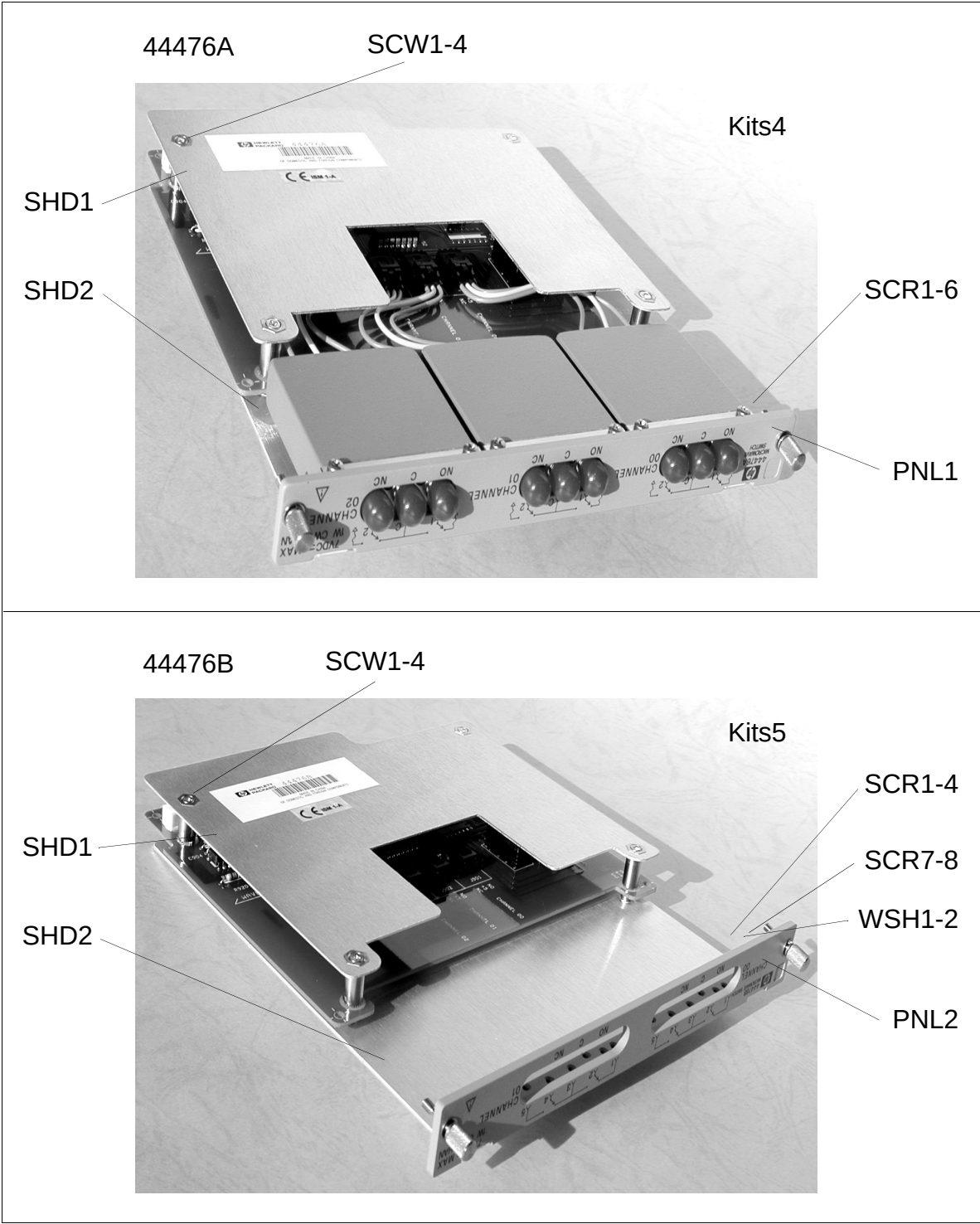
Figure 6-10. Mechanical Kits 4 & 5
