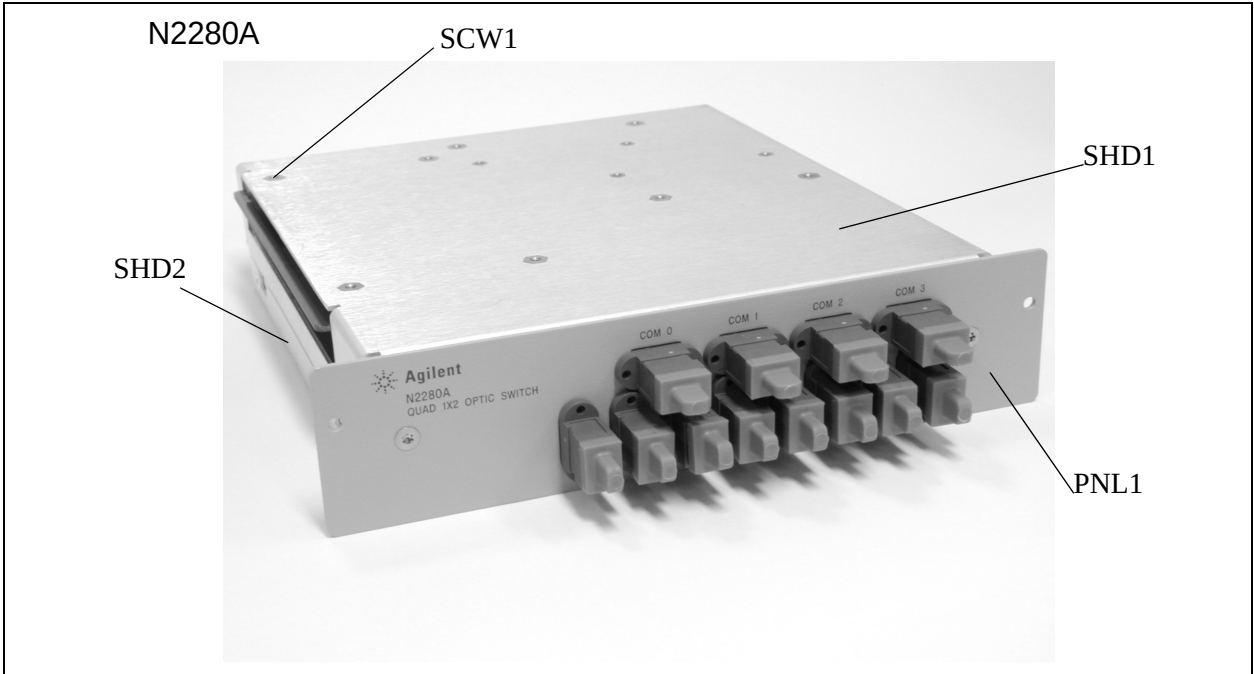
Figure 6-17. Mechanical Kits 12
