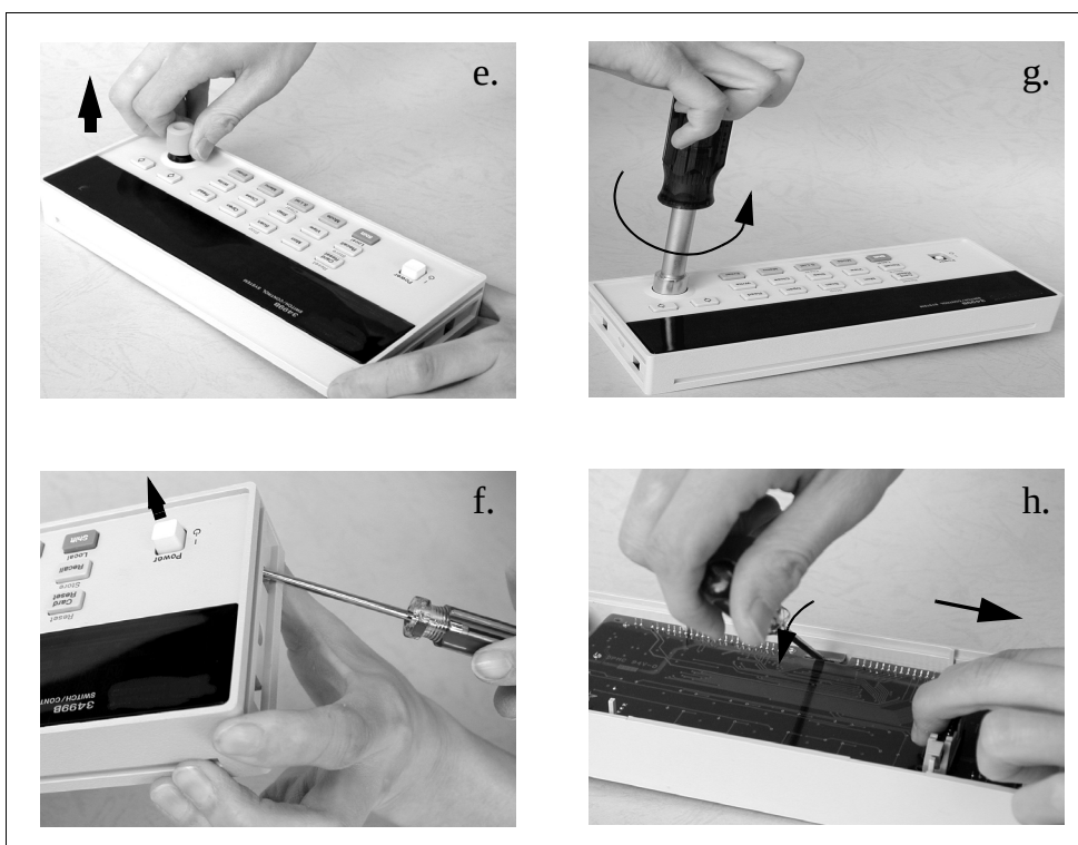
Figure 6-2. Front-Panel Disassembly
