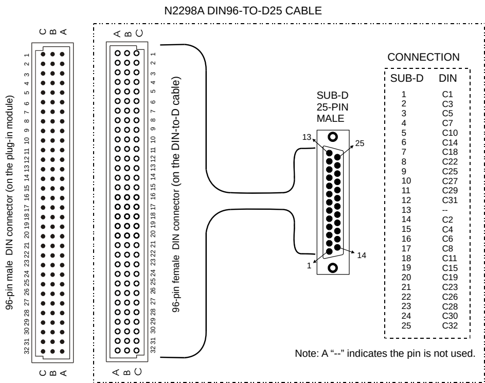
Figure 6-28. Agilent N2298A Cable
