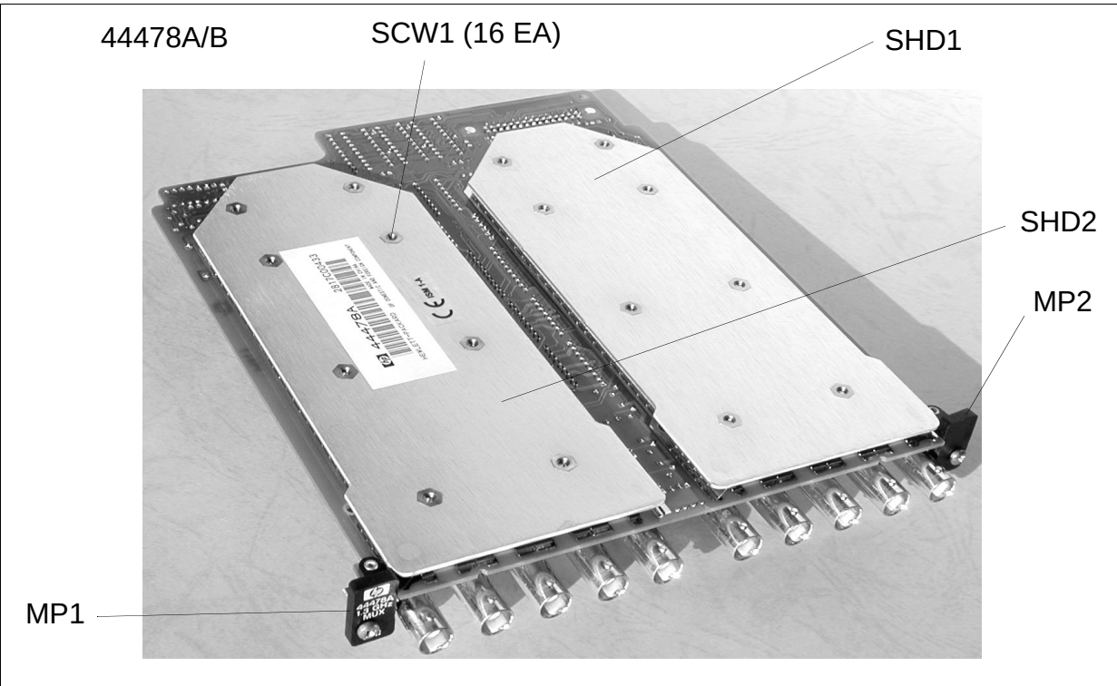
Figure 6-11. Mechanical Kits 6
