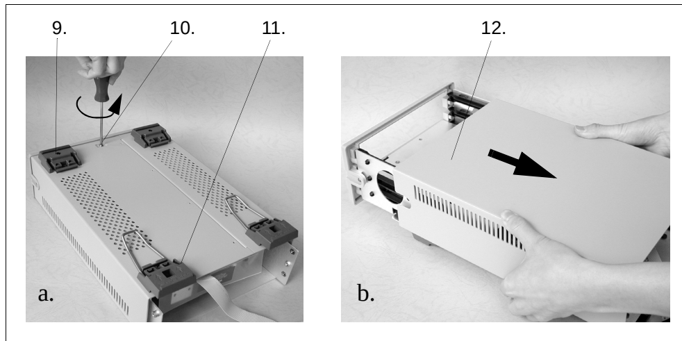
Figure 6-3. Cover Removal
