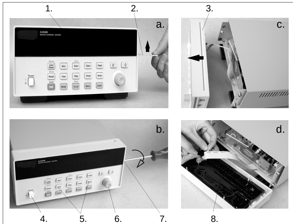
Figure 6-1. Front-Panel Removal
