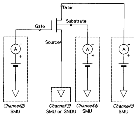
Measurement Circuit
