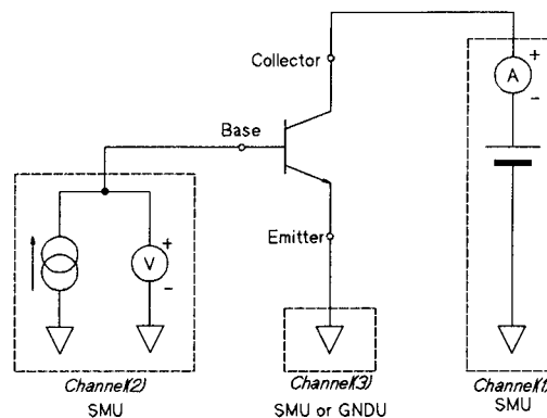
Measurement Circuit
