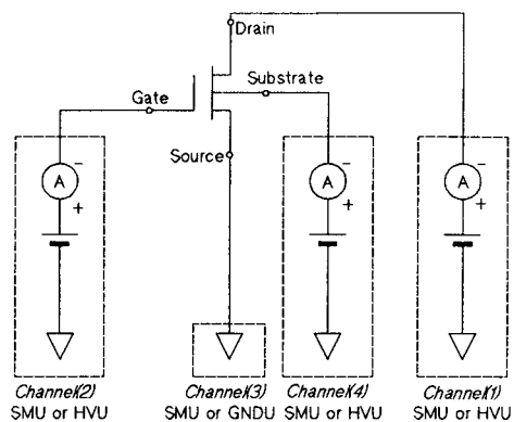
Measurement Circuit
