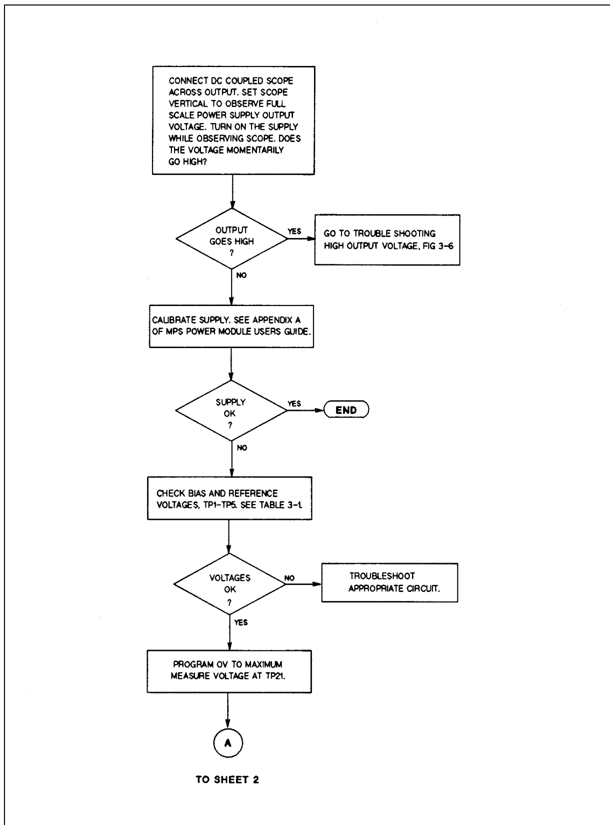
Figure 3-4. Troubleshooting Overvoltage at Turn-On (Sheet 1 of 2)
