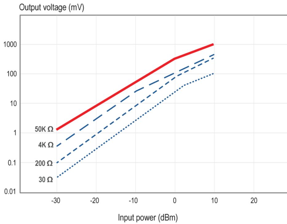
Figure 1. Typical transfer characteristics.
