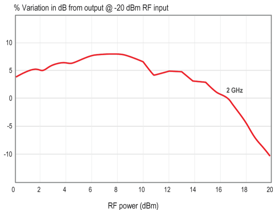
Figure 5. Typical square law deviation.
