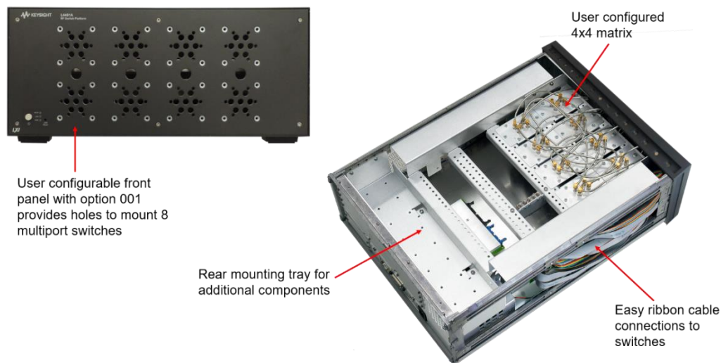
Figure 3. L4491A Customization
