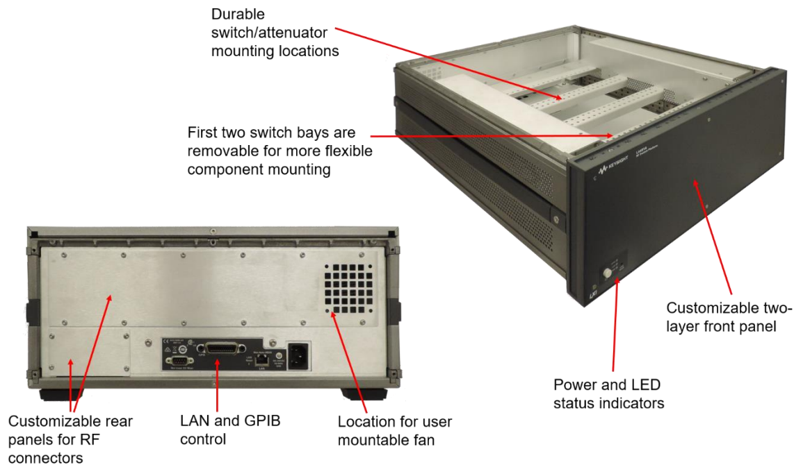
Figure 2. L4491A RF Switch Platform
