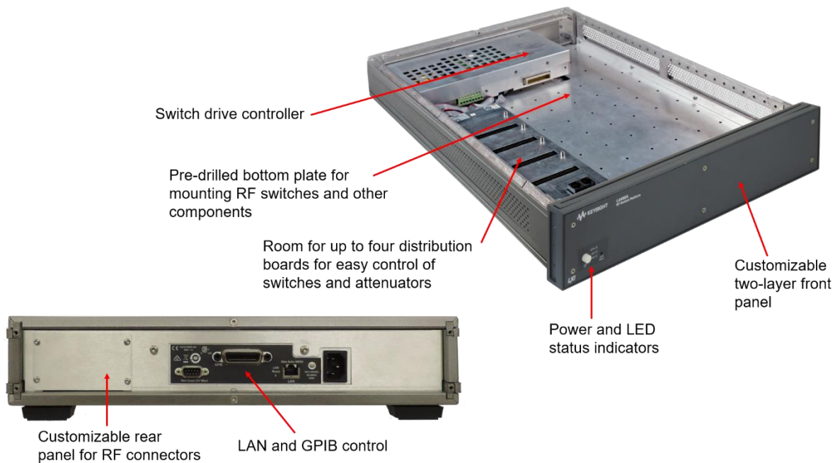
Figure 1. L4490A RF Switch Platform
