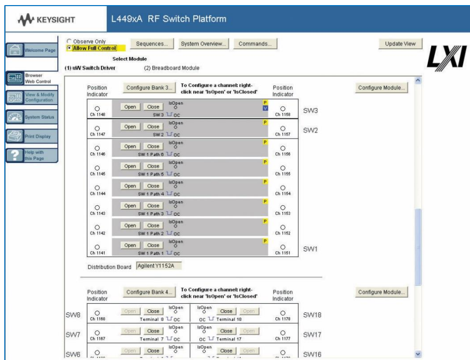
Figure 6. The web interface makes it easy to set up, troubleshoot and maintain your test remotely
