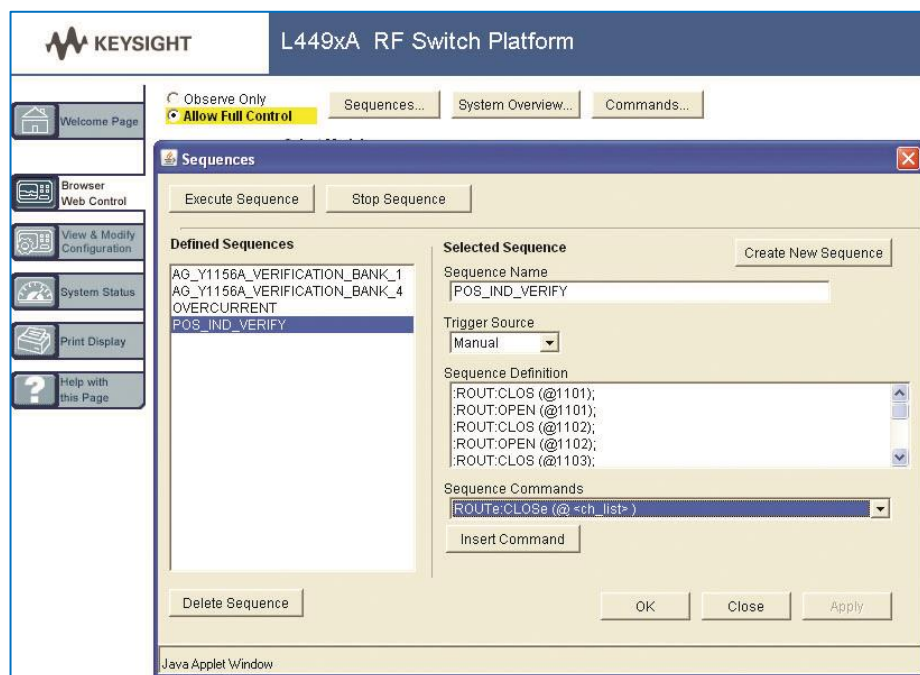
Figure 7. L4490A/91A switch sequences developed/executed from the Web interface or programming environment
