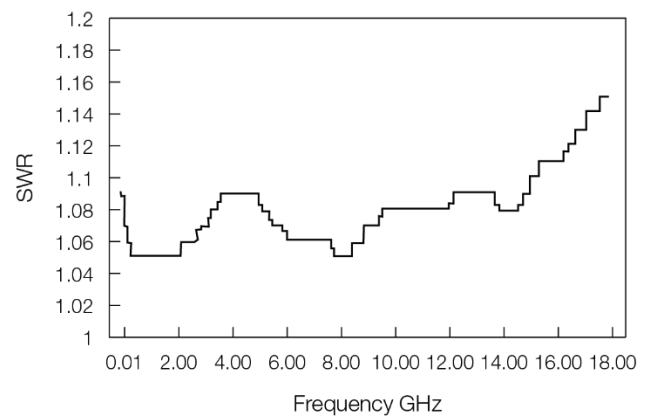
Typical SWR, 9 kHz to 6 GHz ( 25^{\circ}\text{C} \pm 10^{\circ}\text{C} ) for E9304A sensors.
