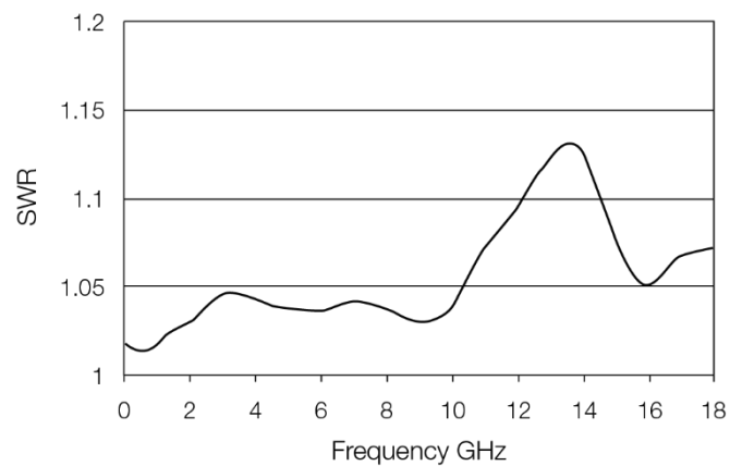
Typical SWR, 10 MHz to 18 GHz ( 25^{\circ}\text{C} \pm 10^{\circ}\text{C} ) for E9300H and E9301H sensors.
