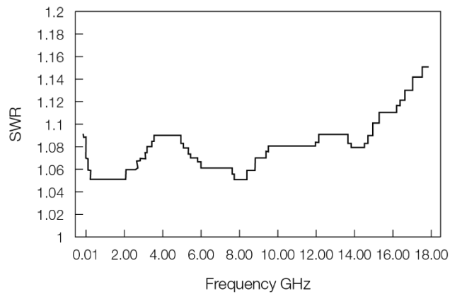
Typical SWR, 10 MHz to 18 GHz ( 25^{\circ}\text{C} \pm 10^{\circ}\text{C} ) for E9300A and E9301A sensor.
